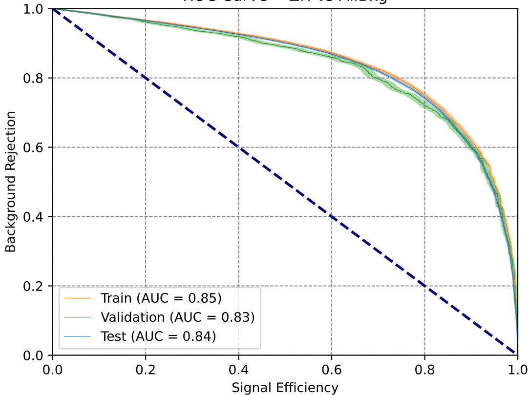
ROC Curve -- ZH vs AllBkg
