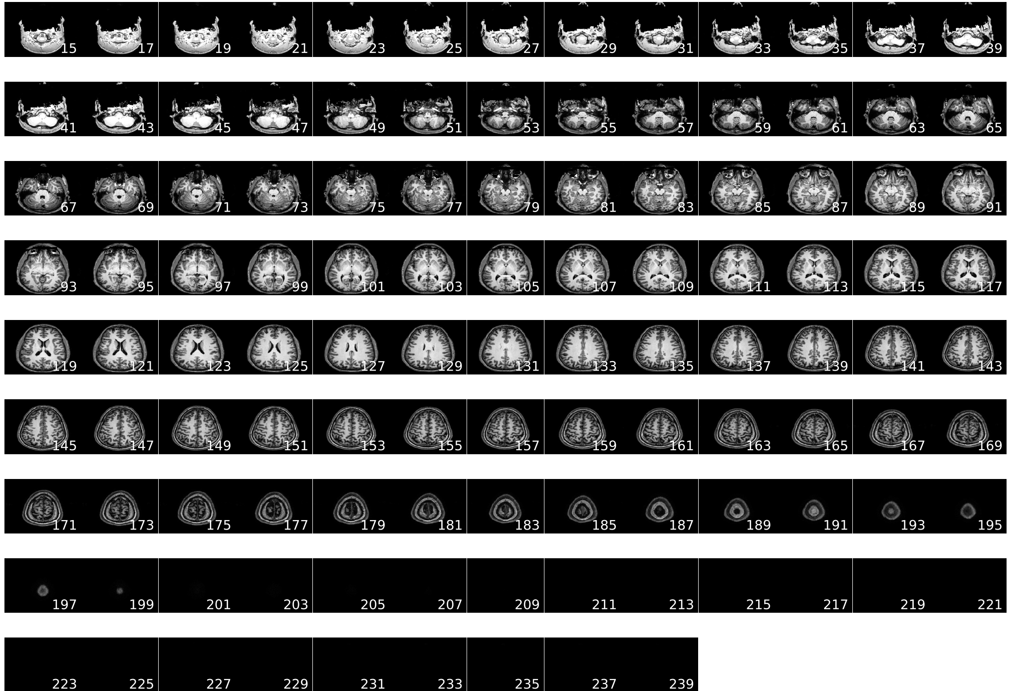
Volume, subject sub-306 (ses-BL_T1w)
