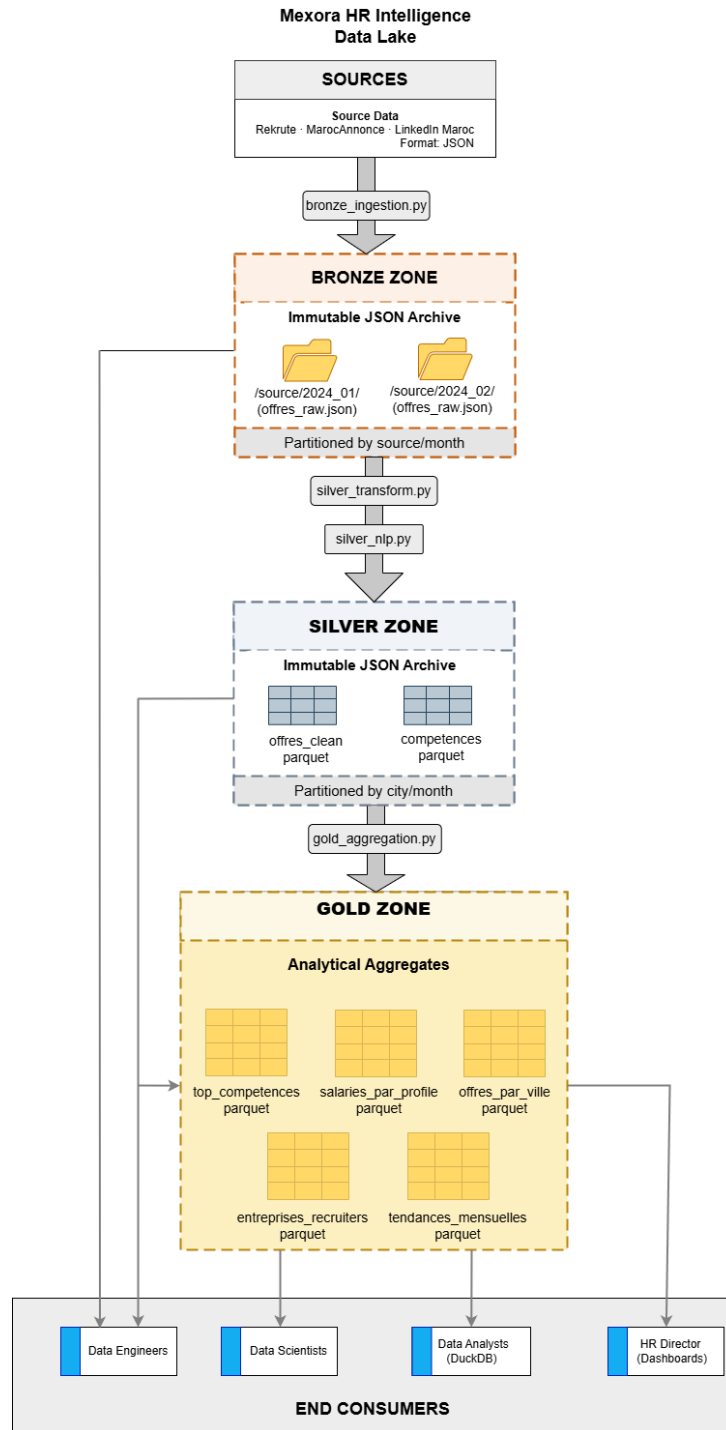
Figure 1. Bronze/Silver/Gold Data Lake architecture — Mexora RH Intelligence. Data flows from three job platforms (Rekrute, MarocAnnonce, LinkedIn) through three quality zones to end being utilized by their respective end consumers
