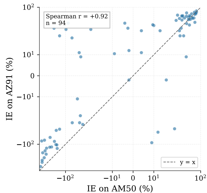
AM50 vs. each commercial-cluster alloy (symlog axes)
