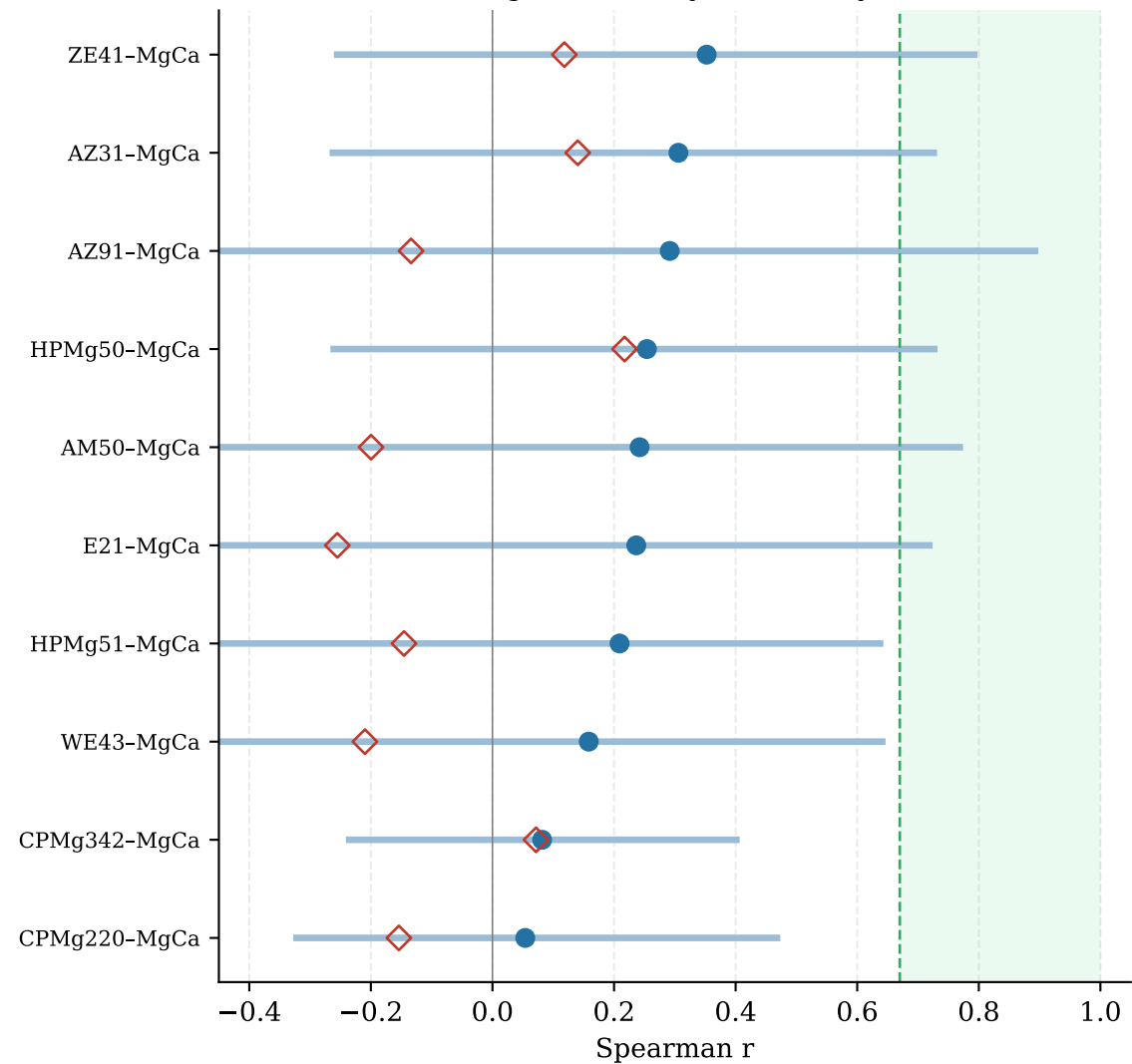
MgCa vs. every other alloy
