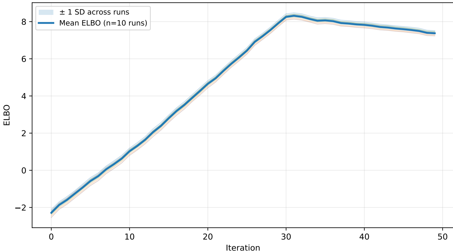
ELBO convergence across runs D-Vine • d=5 • ind-tree=2 • n=1000 • BGTM
