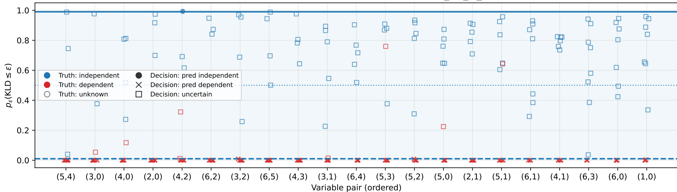
Posterior practical-independence probability per pair across seeds C-Vine • d=7 • ind-tree=2 • n=1000 • BGTM • \epsilon=0.001 , \gamma=0.99 • Pairs ordered by mean( p_{\text{kld\_le\_eps}} ) across seeds.
