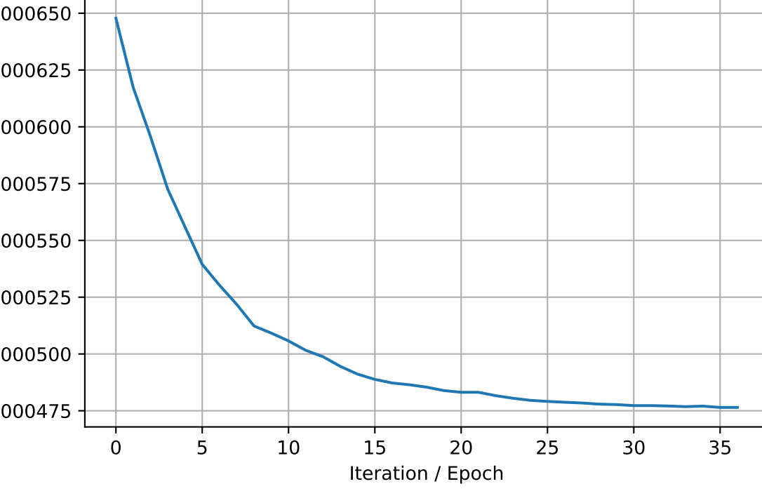
mu_norm
