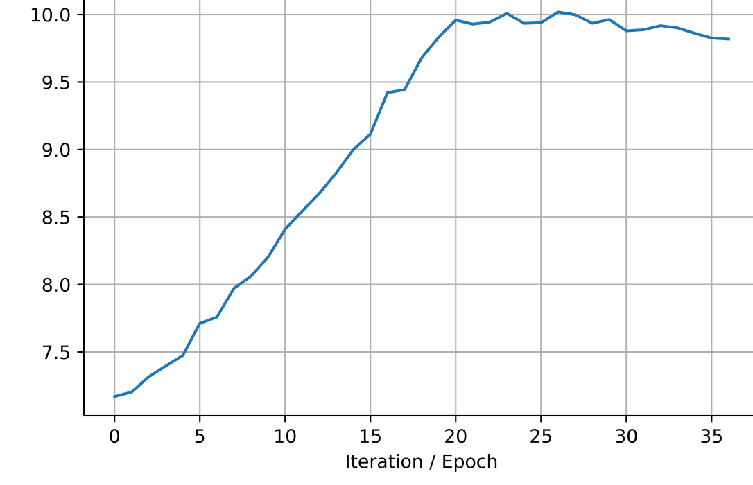
train_loss
