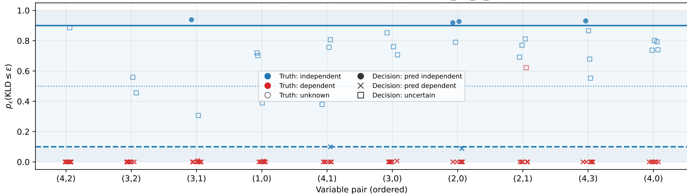
Posterior practical-independence probability per pair across seeds D-Vine • d=5 • ind-tree=2 • n=1000 • BGTM • \epsilon=0.001 , \gamma=0.90 • Pairs ordered by mean( p_{\text{kld\_le\_eps}} ) across seeds.
