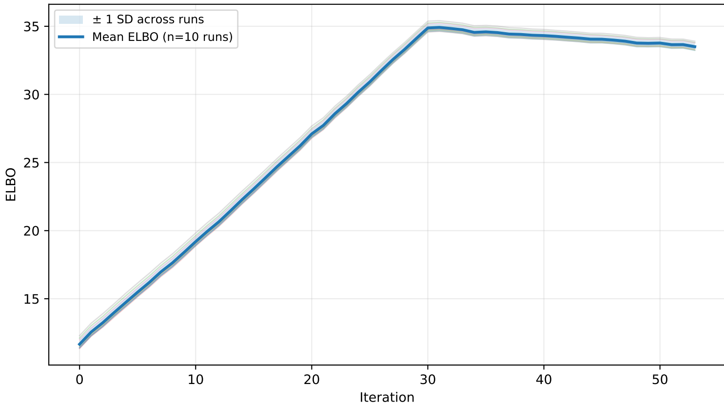
ELBO convergence across runs R-Vine • d=7 • ind-tree=2 • n=1000 • BGTM
