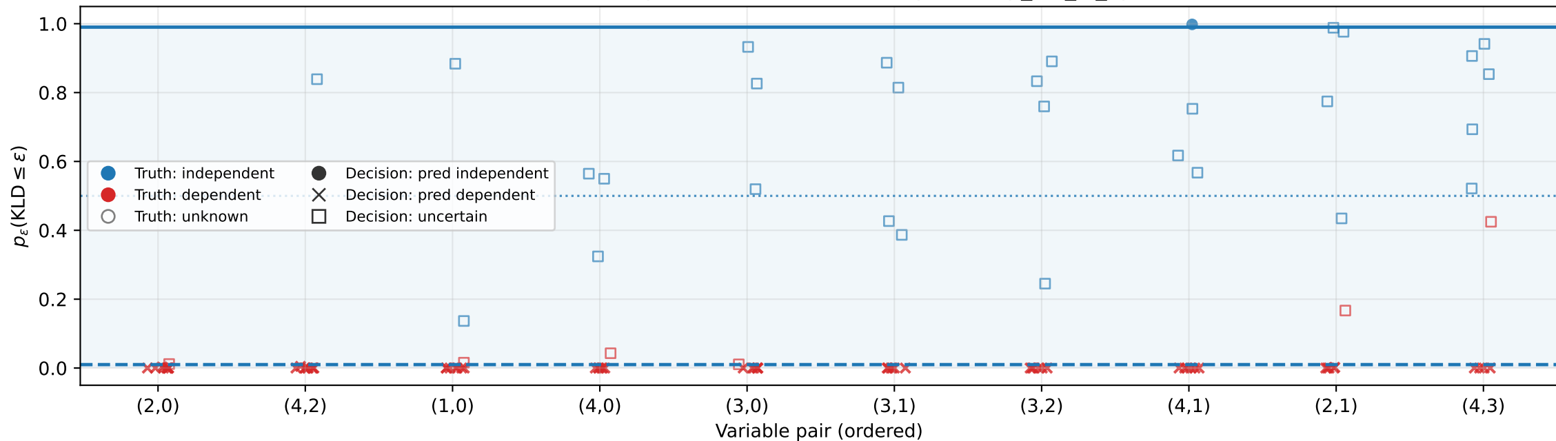
Posterior practical-independence probability per pair across seeds C-Vine • d=5 • ind-tree=2 • n=1000 • BGTM • \varepsilon=0.001 , \gamma=0.99 • Pairs ordered by mean( p_{\text{kld\_le\_eps}} ) across seeds.
