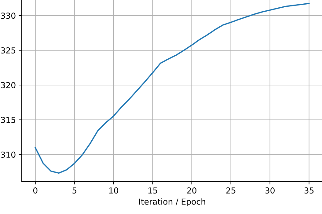
sigma_max
