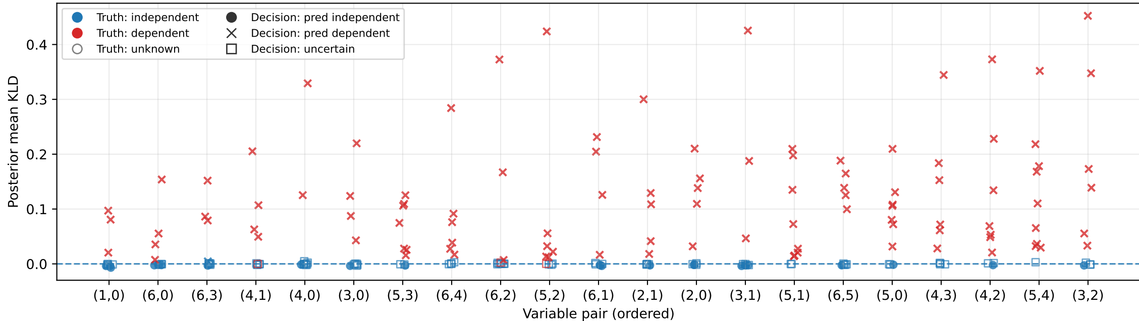
Posterior mean KLD per pair across seeds R-Vine • d=7 • ind-tree=2 • n=1000 • BGTM • Pairs ordered by mean(kld_mean) across seeds.
