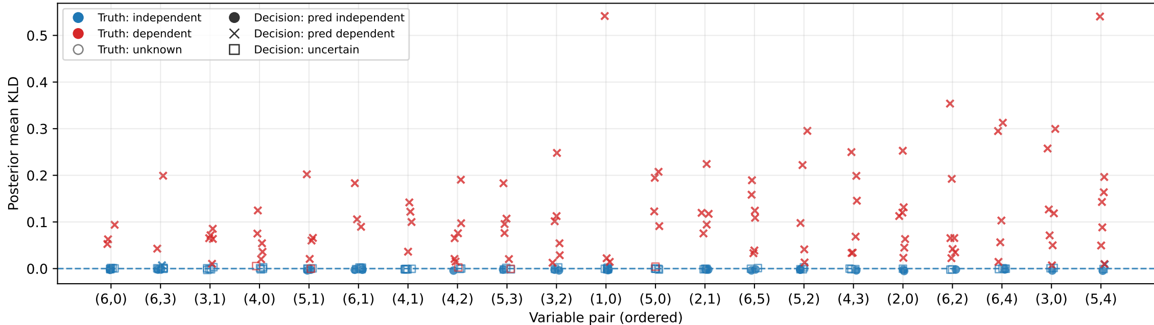
Posterior mean KLD per pair across seeds C-Vine • d=7 • ind-tree=2 • n=1000 • BGTM • Pairs ordered by mean(kld_mean) across seeds.
