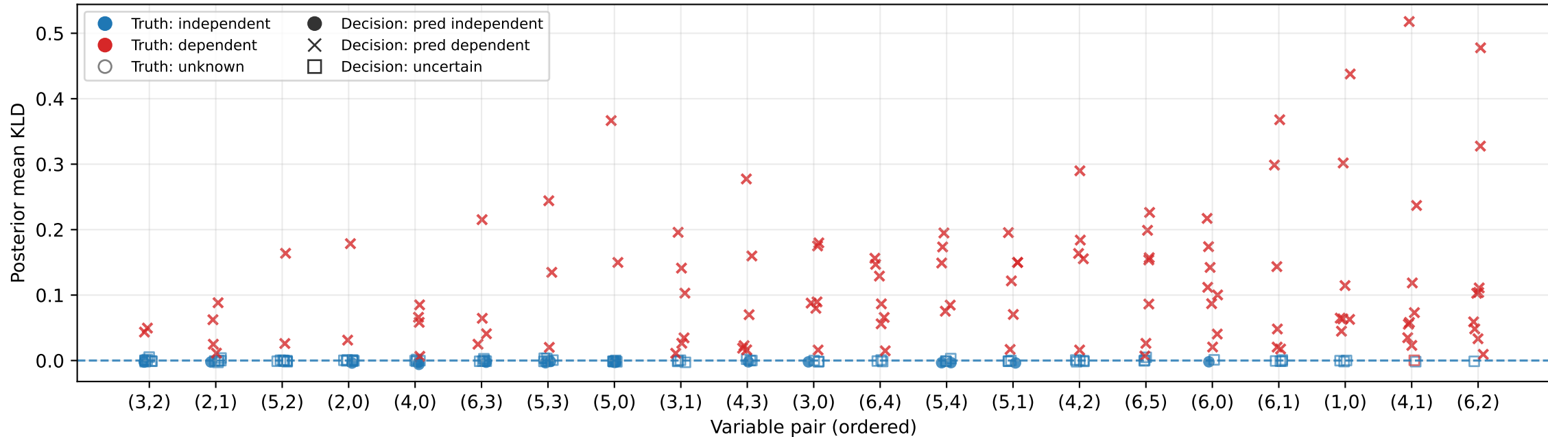
Posterior mean KLD per pair across seeds D-Vine • d=7 • ind-tree=2 • n=1000 • BGTM • Pairs ordered by mean(kld_mean) across seeds.
