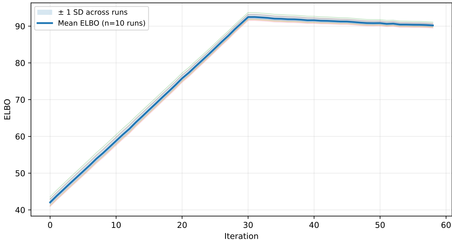
ELBO convergence across runs R-Vine • d=10 • ind-tree=3 • n=1000 • BGTM
