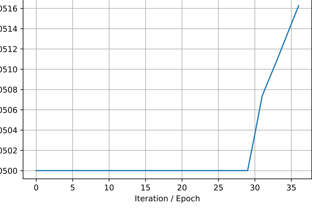
elbo_per_obs
