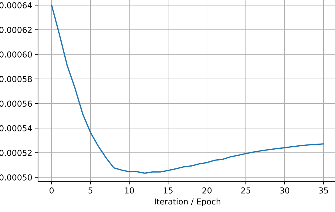
mu_norm
