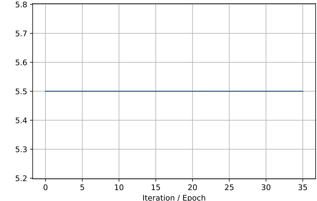
tau1_mean
