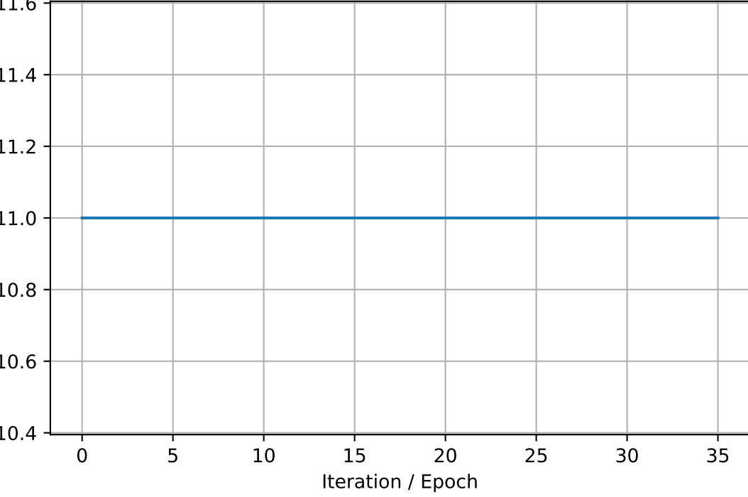
tau2_mean
