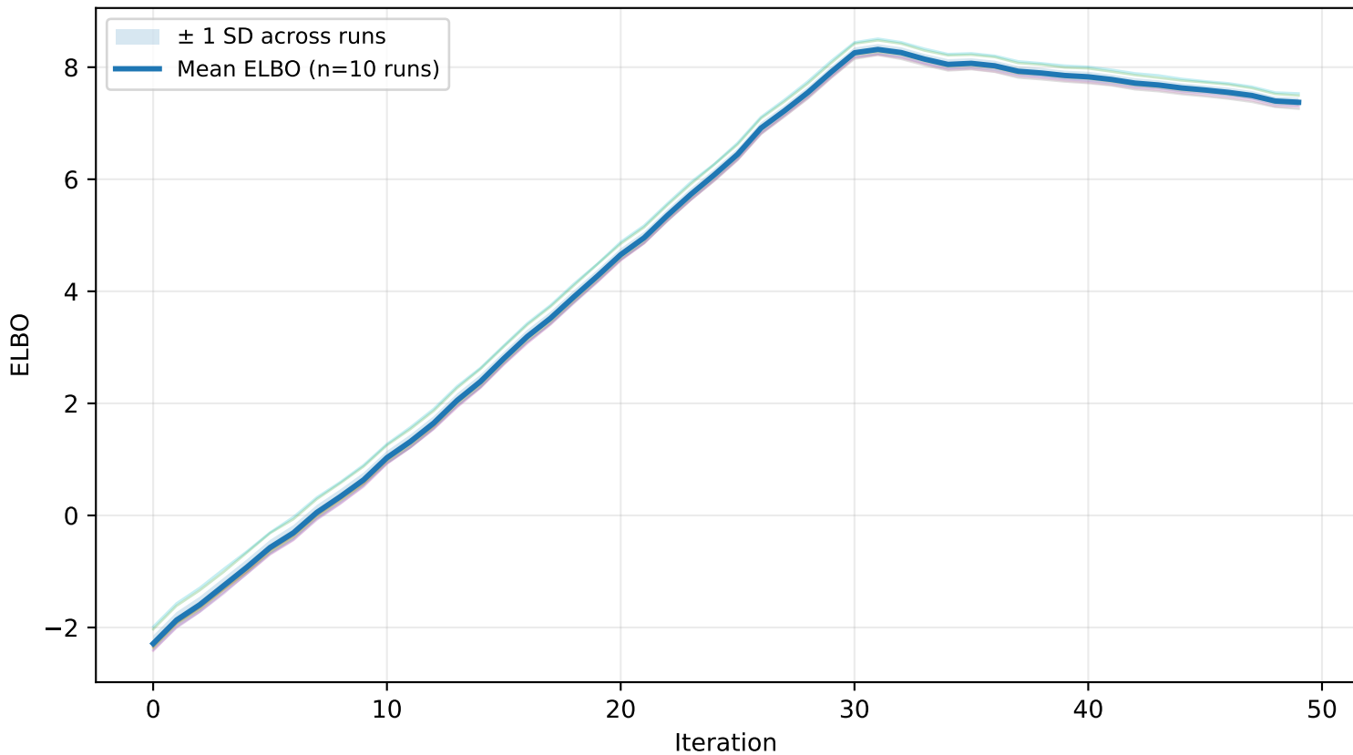
ELBO convergence across runs R-Vine • d=5 • ind-tree=2 • n=1000 • BGTM
