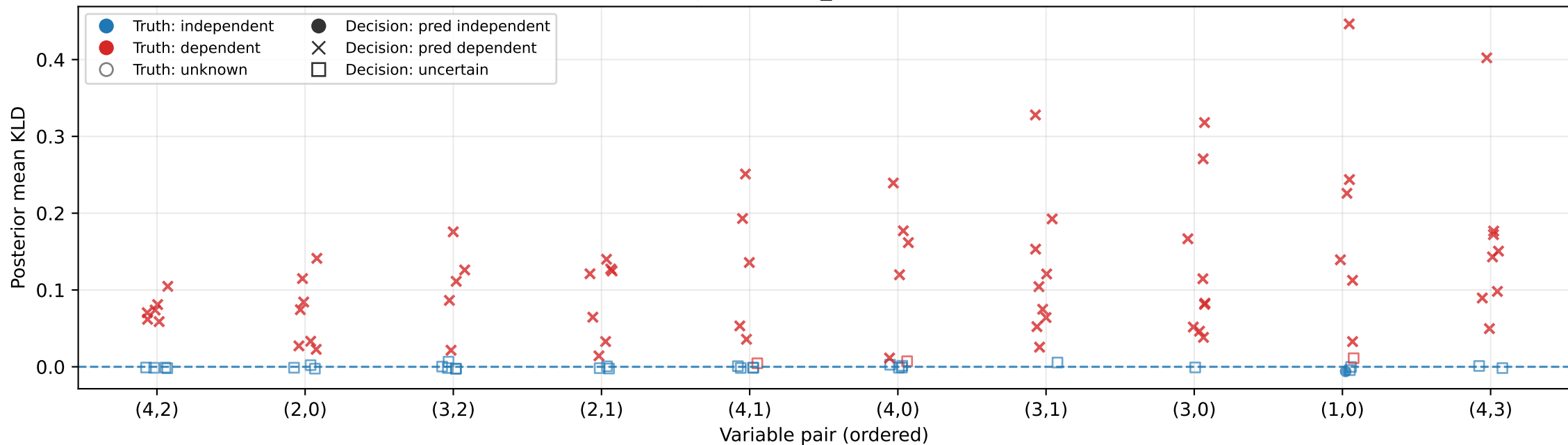
Posterior mean KLD per pair across seeds R-Vine • d=5 • ind-tree=2 • n=1000 • BGTM • Pairs ordered by mean(kld_mean) across seeds.
