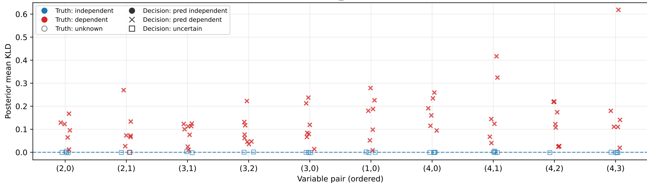
Posterior mean KLD per pair across seeds D-Vine • d=5 • ind-tree=2 • n=1000 • BGTM • Pairs ordered by mean(kld_mean) across seeds.
