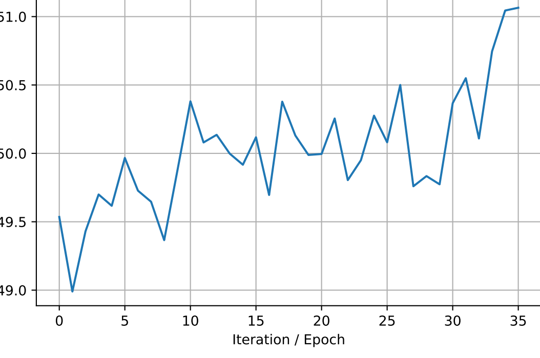
mu_std
