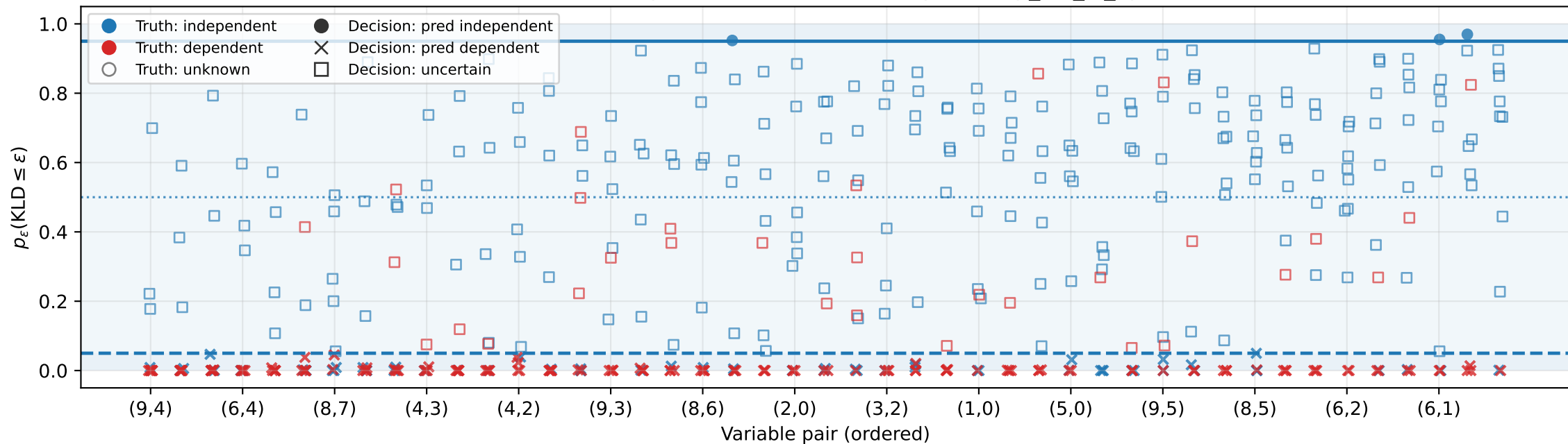
Posterior practical-independence probability per pair across seeds D-Vine • d=10 • ind-tree=3 • n=1000 • BGTM • \varepsilon=0.001 , \gamma=0.95 • Pairs ordered by mean( p_{\text{kld\_le\_eps}} ) across seeds.
