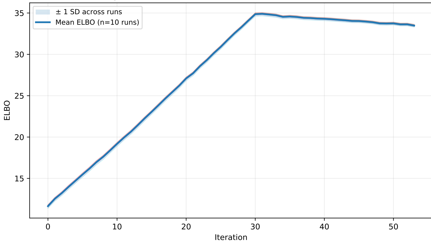
ELBO convergence across runs D-Vine • d=7 • ind-tree=2 • n=1000 • BGTM
