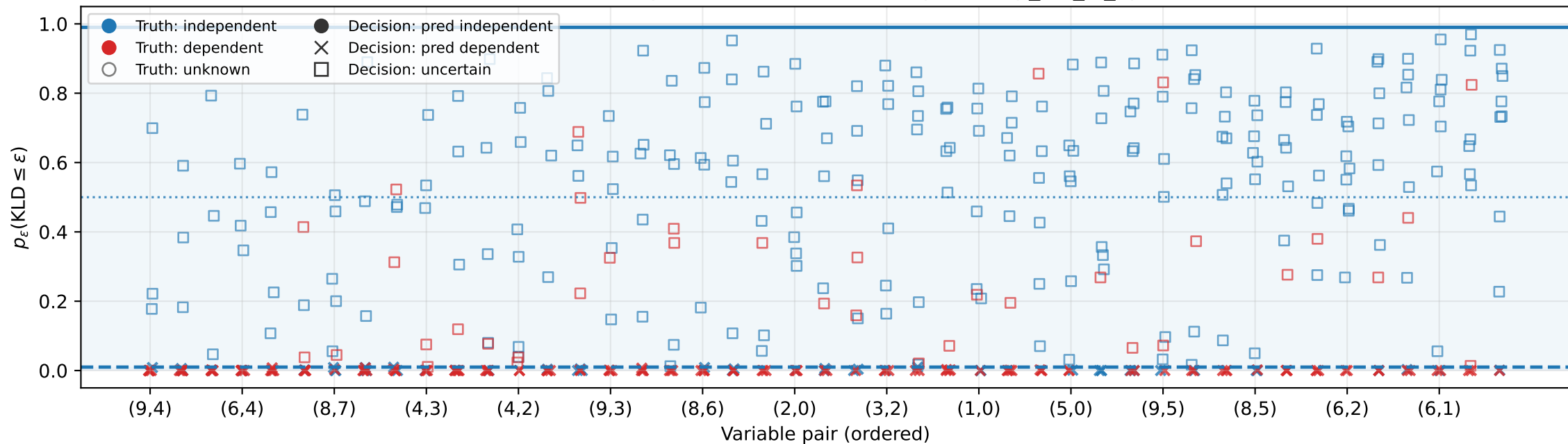
Posterior practical-independence probability per pair across seeds D-Vine • d=10 • ind-tree=3 • n=1000 • BGTM • \varepsilon=0.001 , \gamma=0.99 • Pairs ordered by mean( p_{\text{kld\_le\_eps}} ) across seeds.
