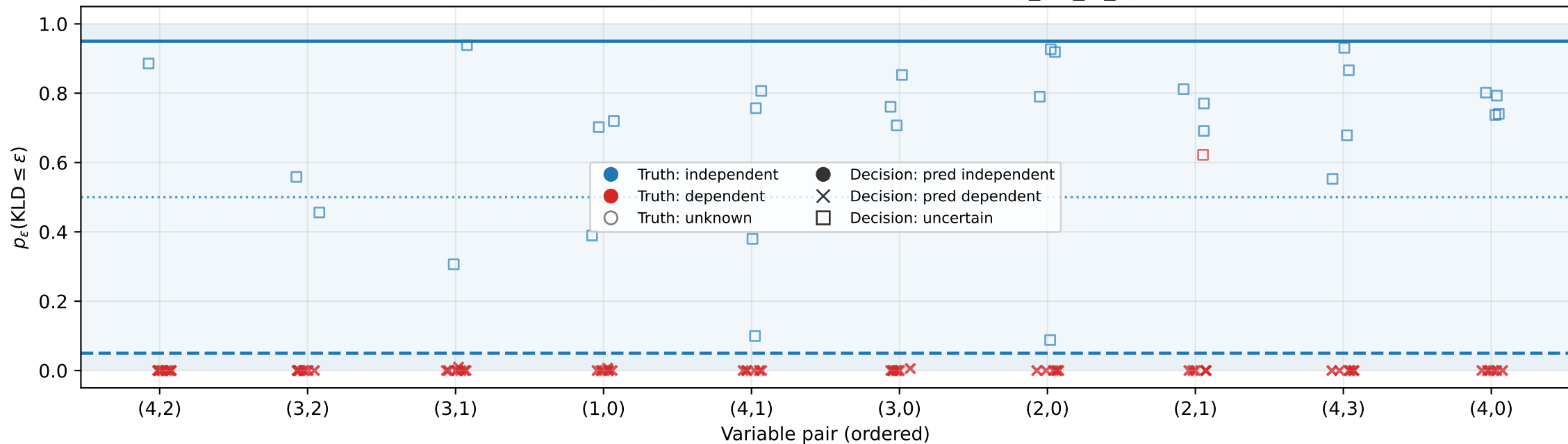
Posterior practical-independence probability per pair across seeds D-Vine • d=5 • ind-tree=2 • n=1000 • BGTM • \varepsilon=0.001 , \gamma=0.95 • Pairs ordered by mean( p_{\text{kld\_le\_eps}} ) across seeds.
