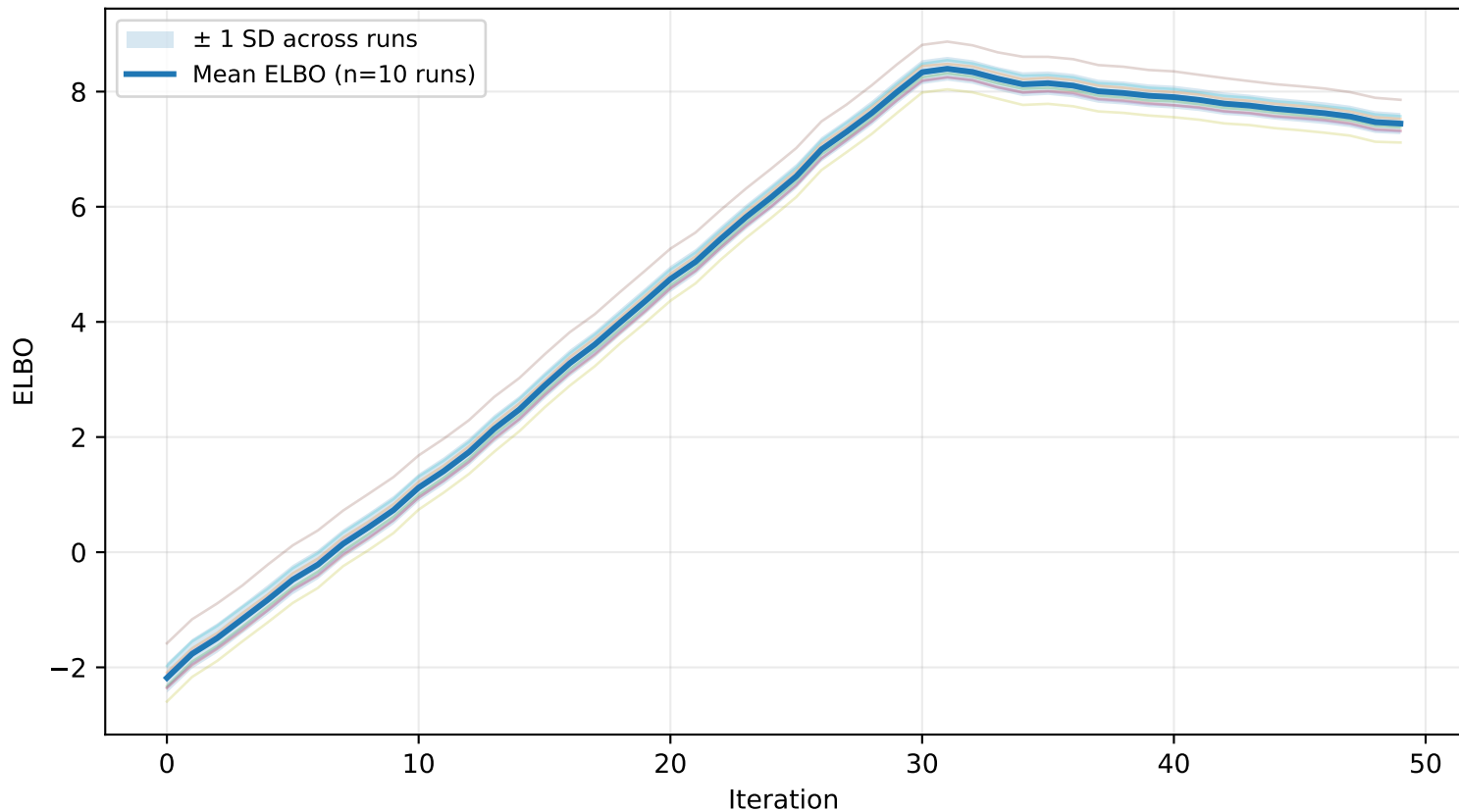
ELBO convergence across runs C-Vine • d=5 • ind-tree=2 • n=1000 • BGTM
