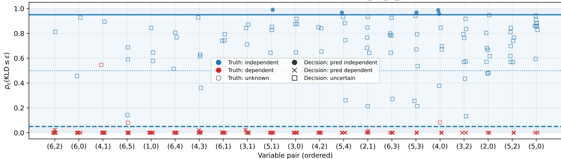
Posterior practical-independence probability per pair across seeds D-Vine • d=7 • ind-tree=2 • n=1000 • BGTM • \epsilon=0.001 , \gamma=0.95 • Pairs ordered by mean( p_{\text{kld\_le\_eps}} ) across seeds.
