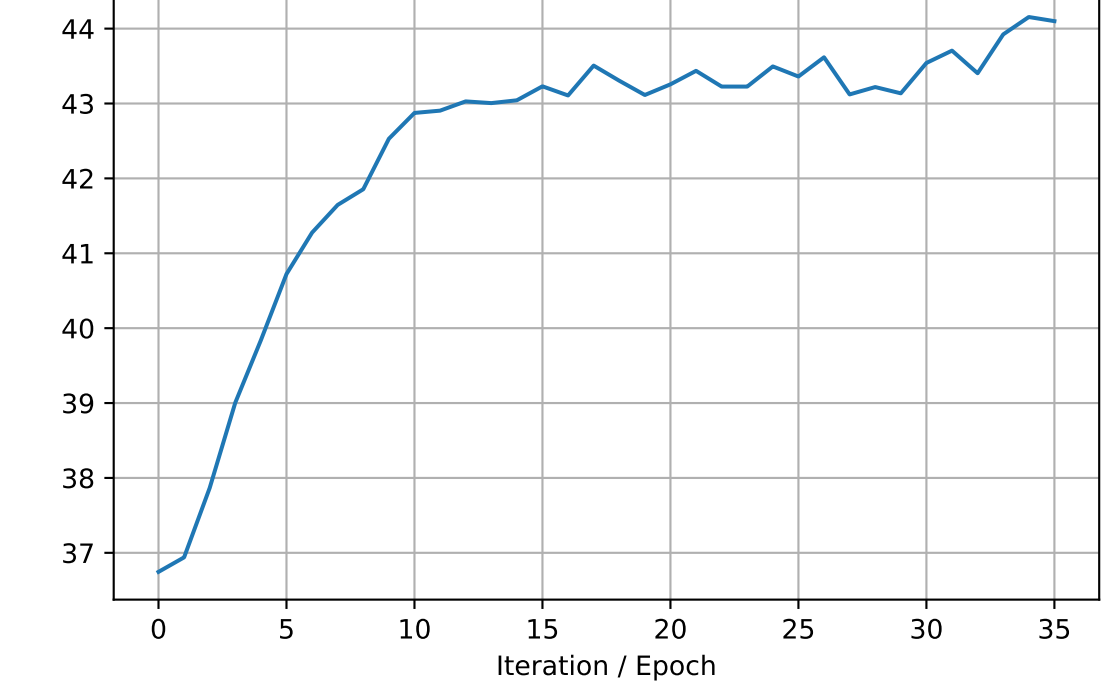
mu_mean
