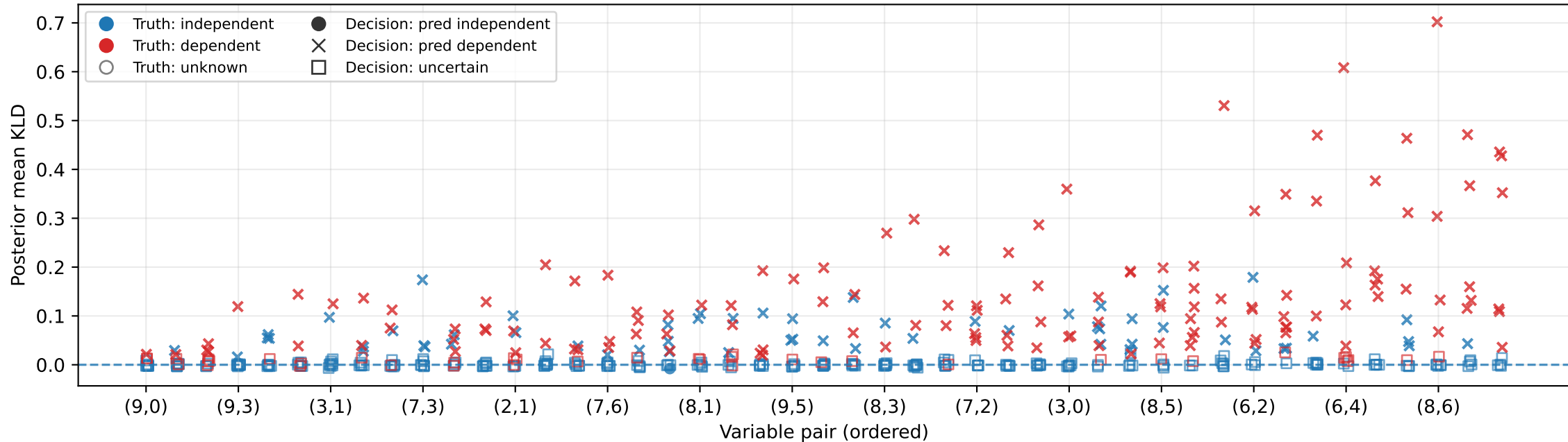
Posterior mean KLD per pair across seeds C-Vine • d=10 • ind-tree=3 • n=1000 • BGTM • Pairs ordered by mean(kld_mean) across seeds.
