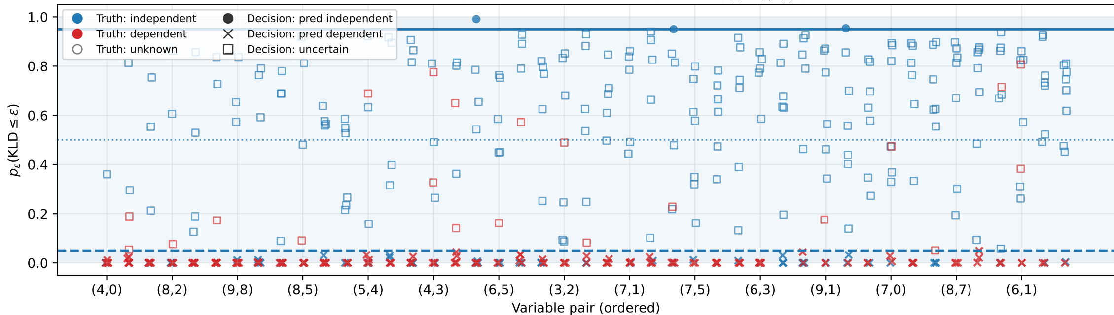
Posterior practical-independence probability per pair across seeds C-Vine • d=10 • ind-tree=3 • n=1000 • BGTM • \varepsilon=0.001 , \gamma=0.95 • Pairs ordered by mean( p_{\text{kld\_le\_eps}} ) across seeds.
