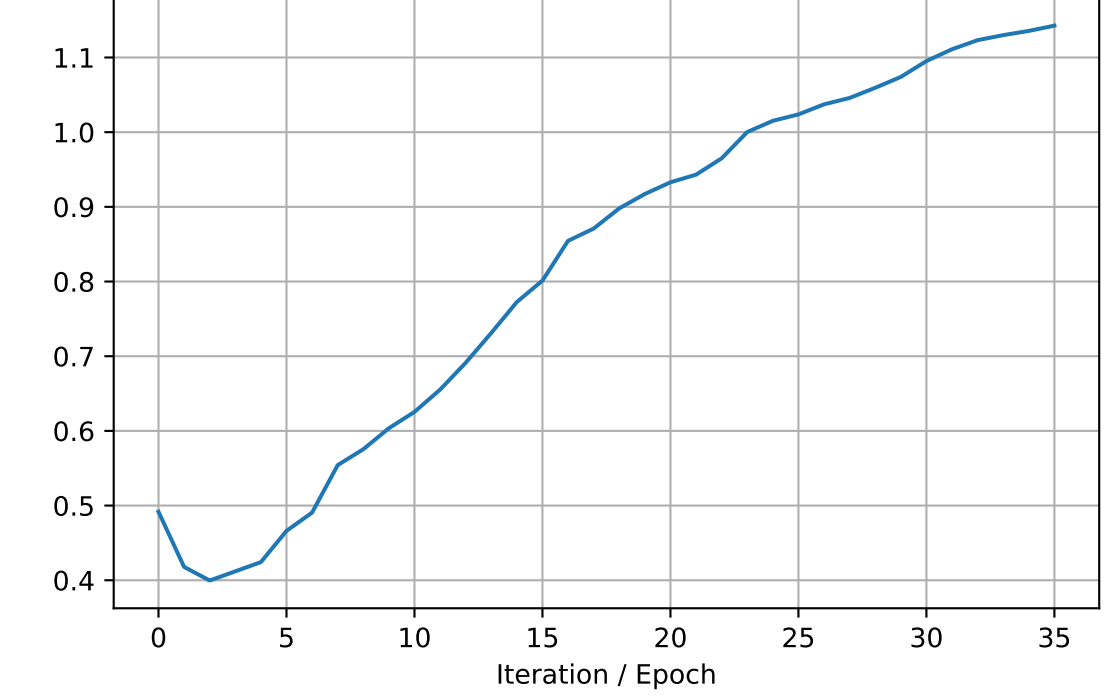
tau1_target
