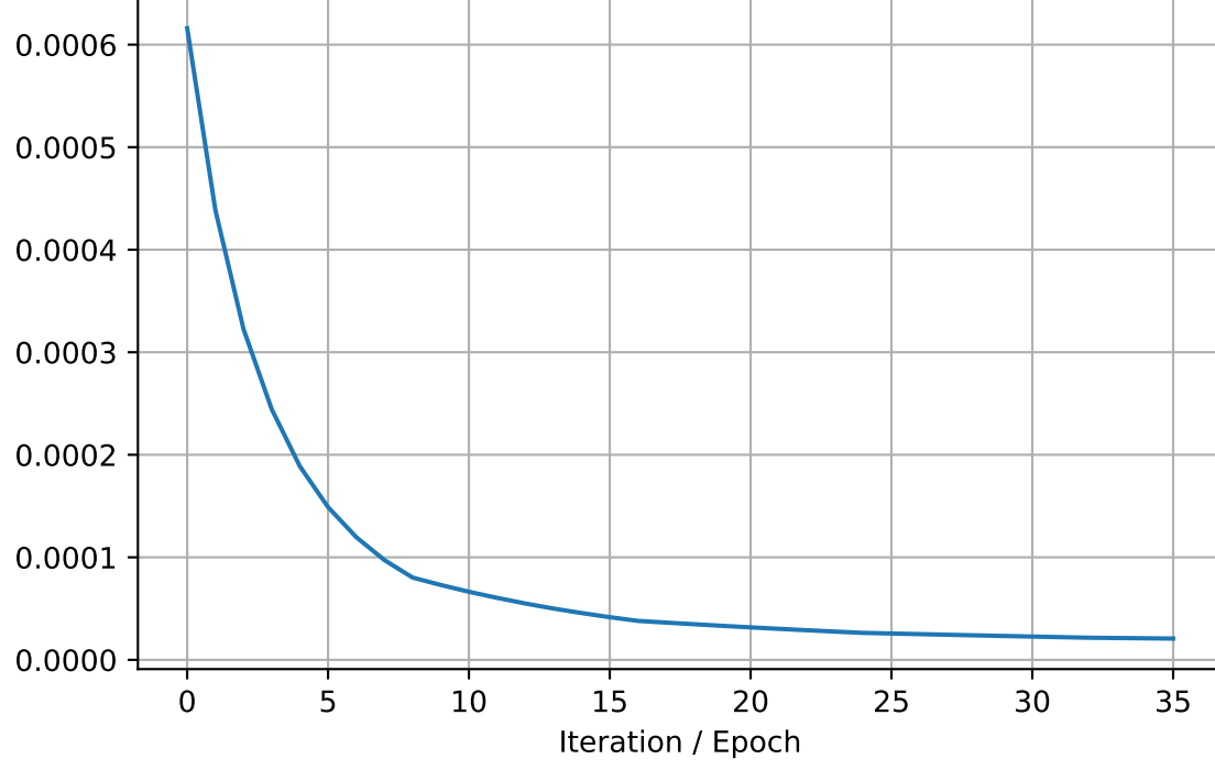
tau4_target
