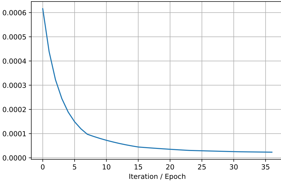
tau4_target
