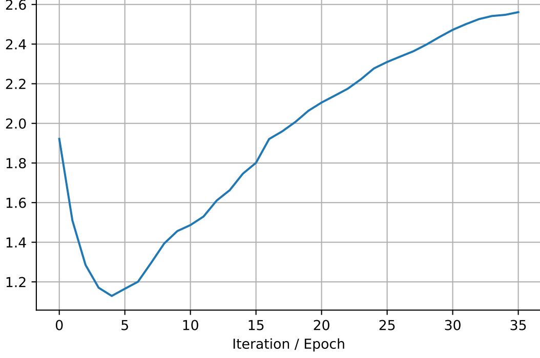
tau2_target
