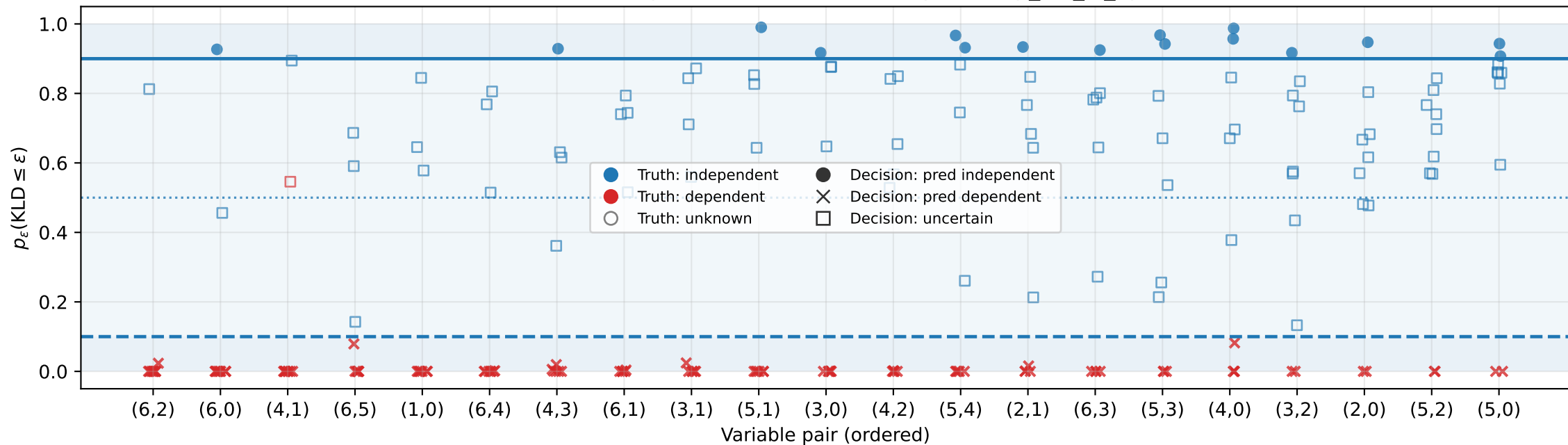
Posterior practical-independence probability per pair across seeds D-Vine • d=7 • ind-tree=2 • n=1000 • BGTM • \epsilon=0.001 , \gamma=0.90 • Pairs ordered by mean( p_{\text{kld\_le\_eps}} ) across seeds.
