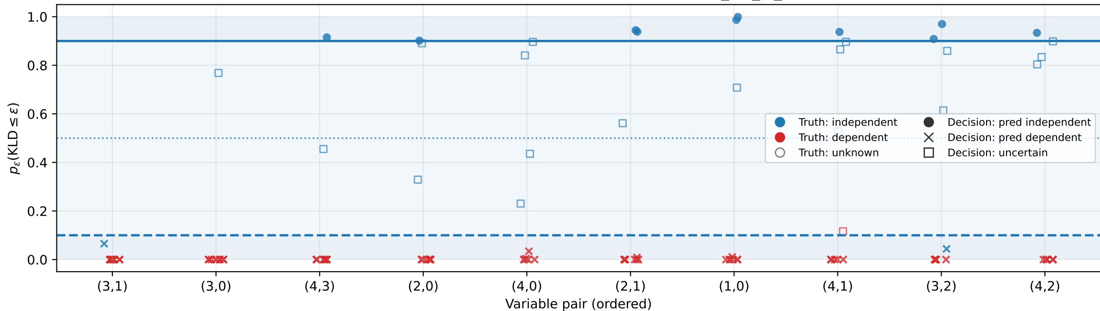
Posterior practical-independence probability per pair across seeds R-Vine • d=5 • ind-tree=2 • n=1000 • BGTM • \varepsilon=0.001 , \gamma=0.90 • Pairs ordered by mean( p_{\text{kld\_le\_eps}} ) across seeds.
