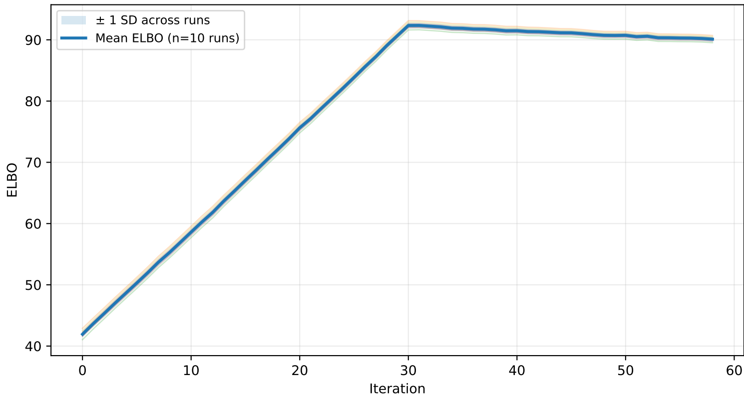
ELBO convergence across runs C-Vine • d=10 • ind-tree=3 • n=1000 • BGTM
