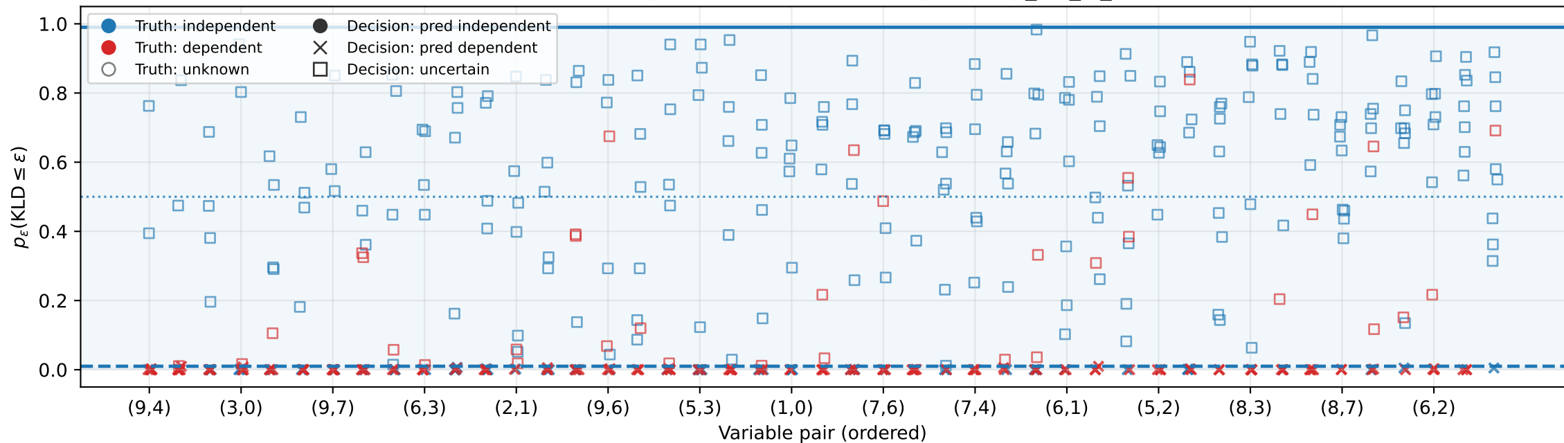
Posterior practical-independence probability per pair across seeds R-Vine • d=10 • ind-tree=3 • n=1000 • BGTM • \epsilon=0.001 , \gamma=0.99 • Pairs ordered by mean( p_{\text{kld\_le\_eps}} ) across seeds.
