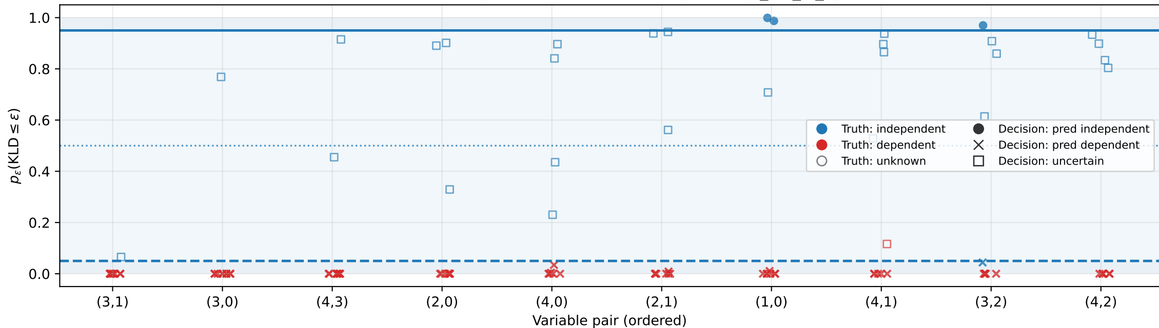
Posterior practical-independence probability per pair across seeds R-Vine • d=5 • ind-tree=2 • n=1000 • BGTM • \epsilon=0.001 , \gamma=0.95 • Pairs ordered by mean( p_{\text{kld\_le\_eps}} ) across seeds.
