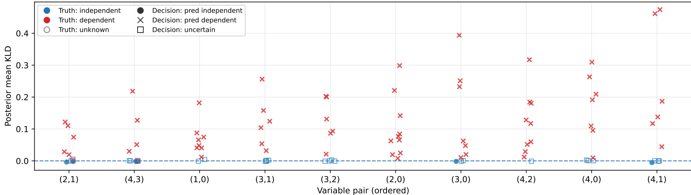
Posterior mean KLD per pair across seeds C-Vine • d=5 • ind-tree=2 • n=1000 • BGTM • Pairs ordered by mean(kld_mean) across seeds.
