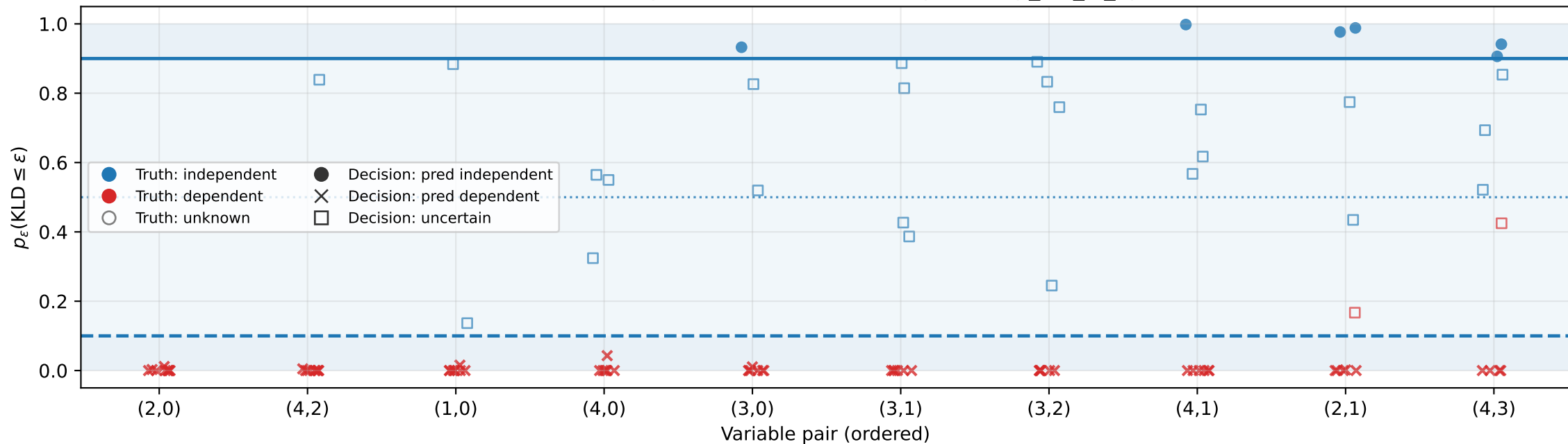
Posterior practical-independence probability per pair across seeds C-Vine • d=5 • ind-tree=2 • n=1000 • BGTM • \varepsilon=0.001 , \gamma=0.90 • Pairs ordered by mean( p_{\text{kld\_le\_eps}} ) across seeds.
