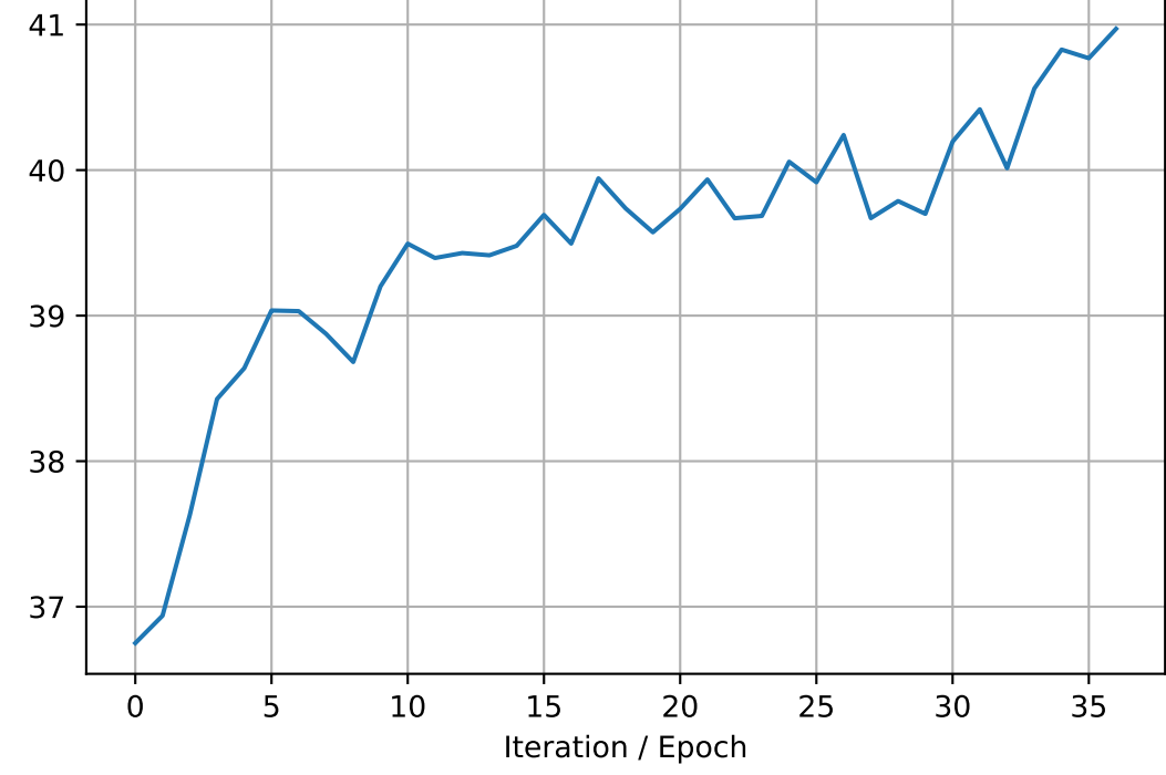
mu_mean
