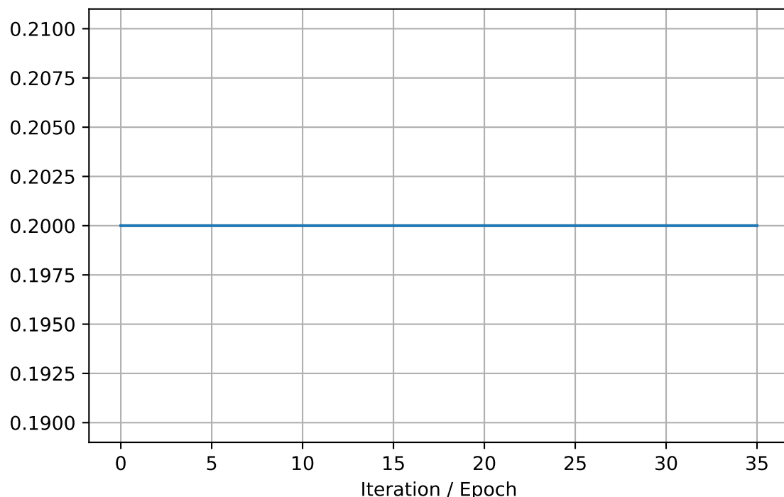
tau4_mean
