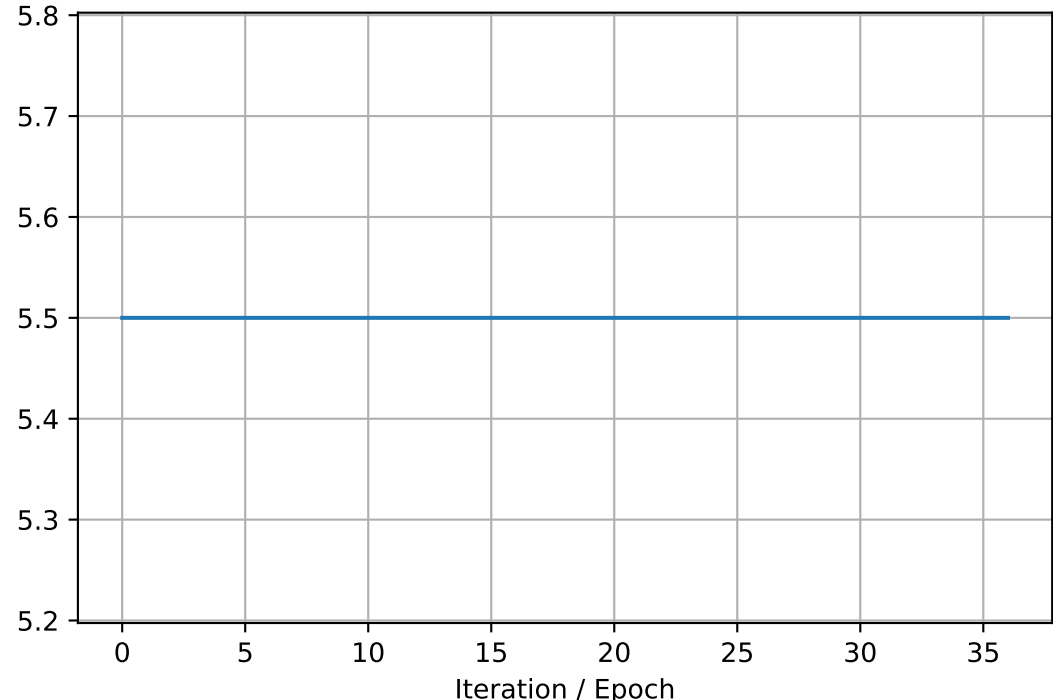
tau1_mean
