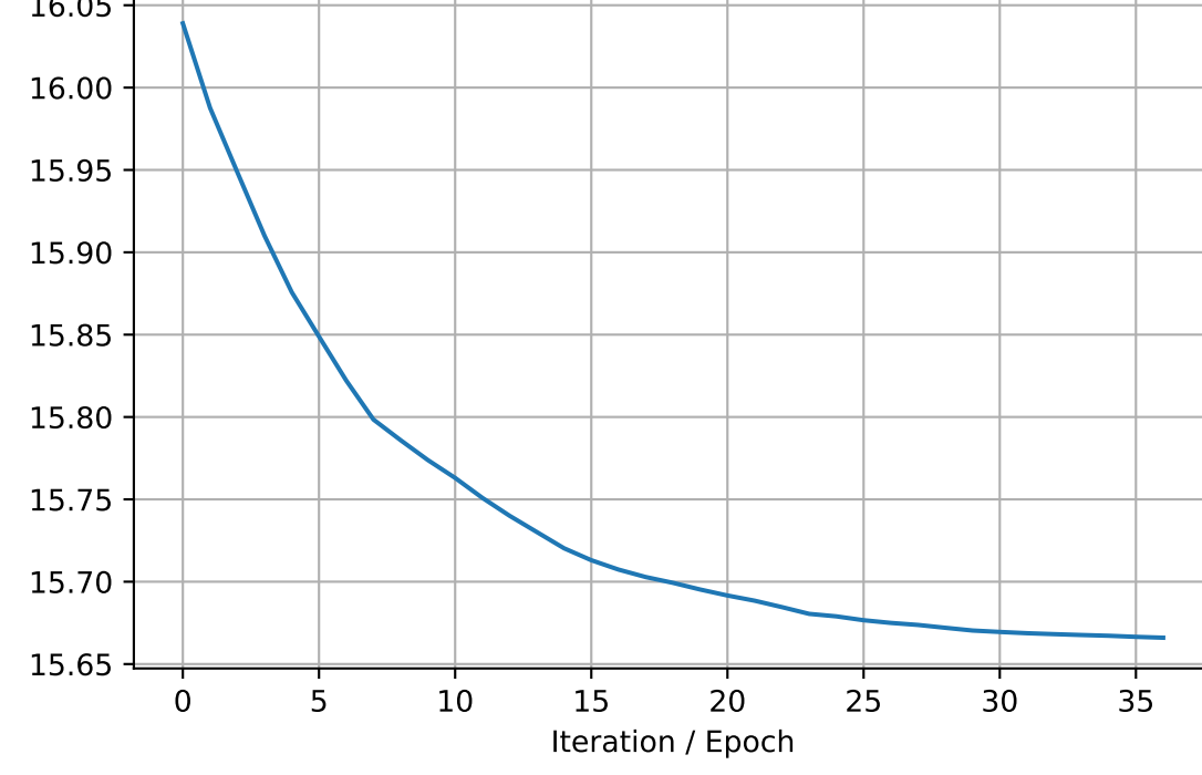
sigma_mean
