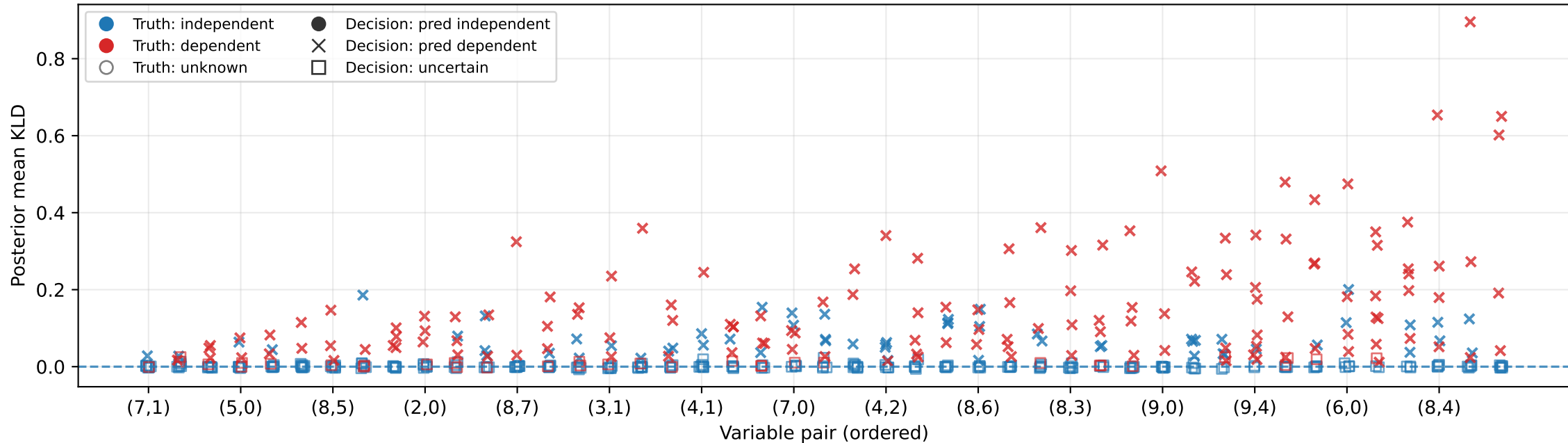
Posterior mean KLD per pair across seeds R-Vine • d=10 • ind-tree=3 • n=1000 • BGTM • Pairs ordered by mean(kld_mean) across seeds.
