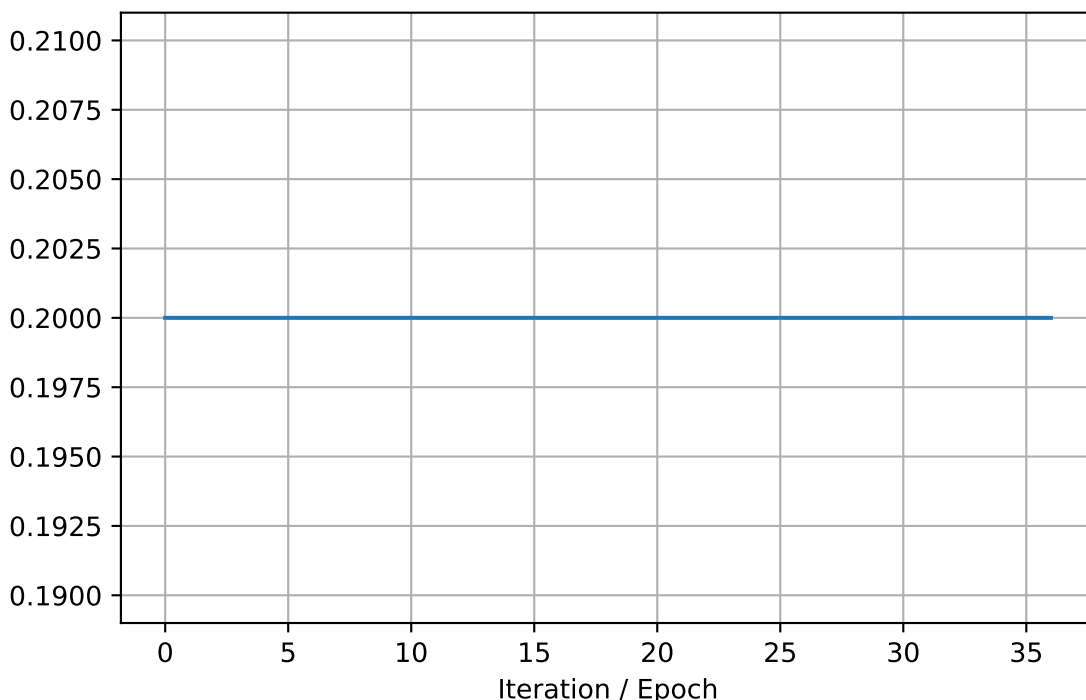
tau4_mean
