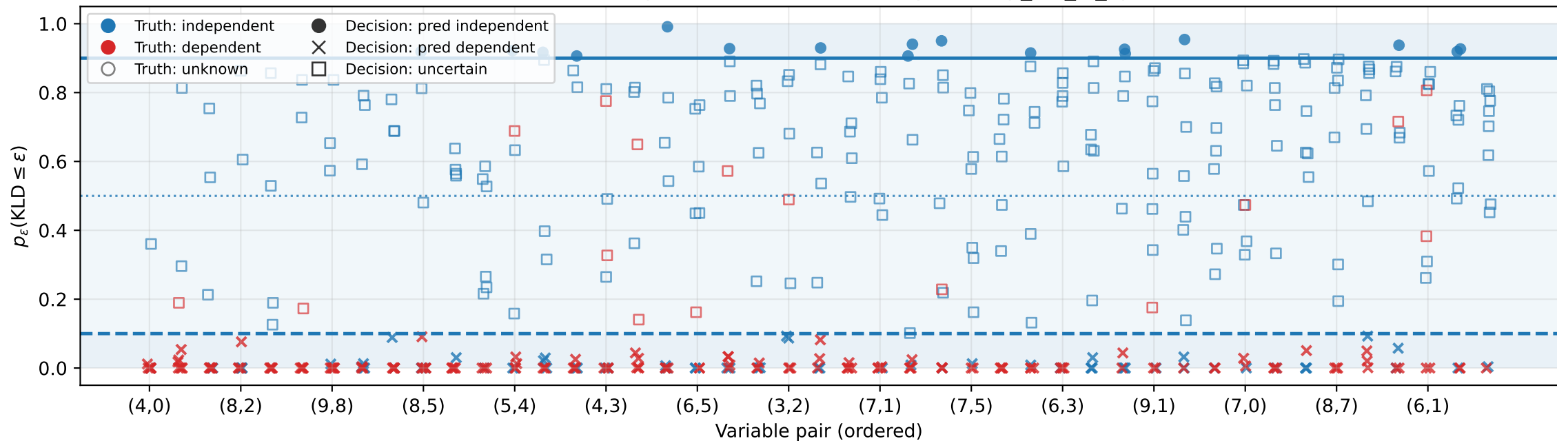
Posterior practical-independence probability per pair across seeds C-Vine • d=10 • ind-tree=3 • n=1000 • BGTM • \varepsilon=0.001 , \gamma=0.90 • Pairs ordered by mean( p_{\text{kld\_le\_eps}} ) across seeds.
