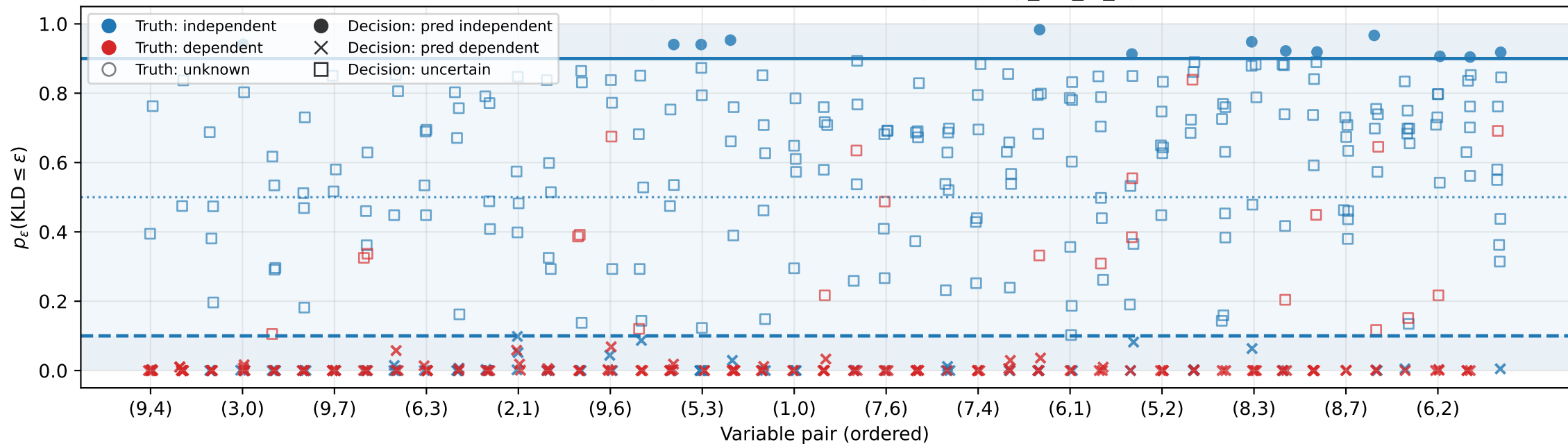
Posterior practical-independence probability per pair across seeds R-Vine • d=10 • ind-tree=3 • n=1000 • BGTM • \varepsilon=0.001 , \gamma=0.90 • Pairs ordered by mean( p_{\text{kld\_le\_eps}} ) across seeds.
