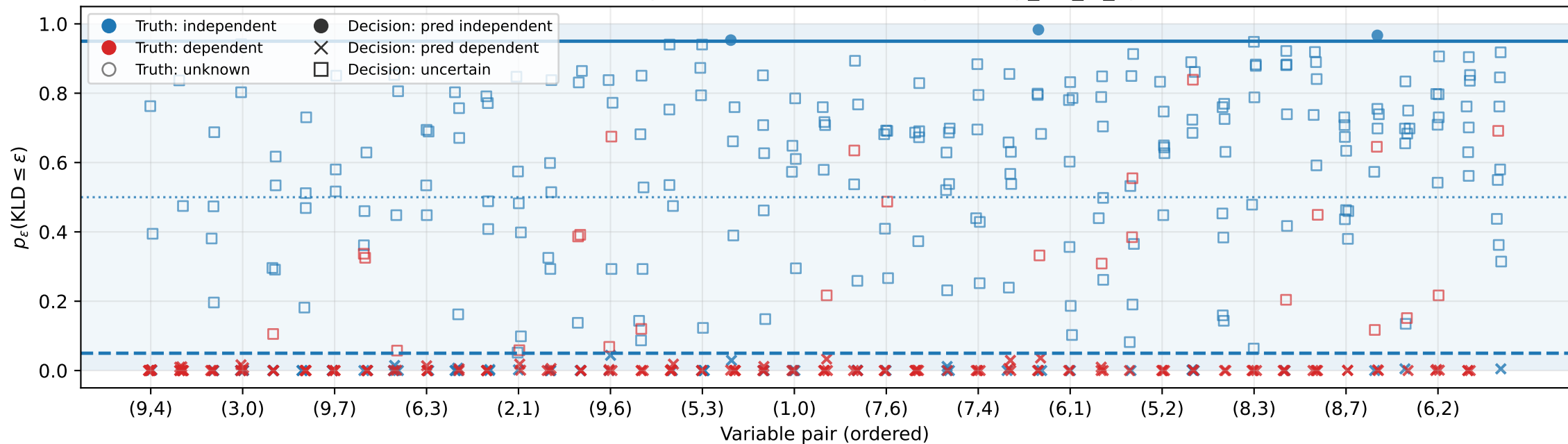
Posterior practical-independence probability per pair across seeds R-Vine • d=10 • ind-tree=3 • n=1000 • BGTM • \epsilon=0.001 , \gamma=0.95 • Pairs ordered by mean( p_{\text{kld\_le\_eps}} ) across seeds.
