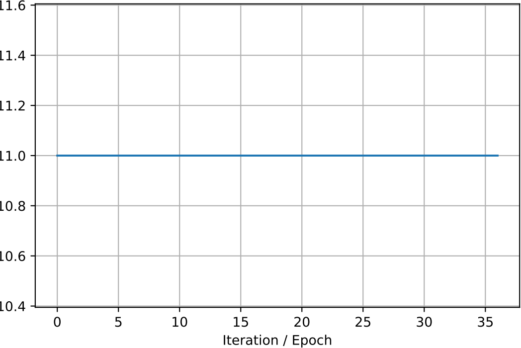
tau2_mean
