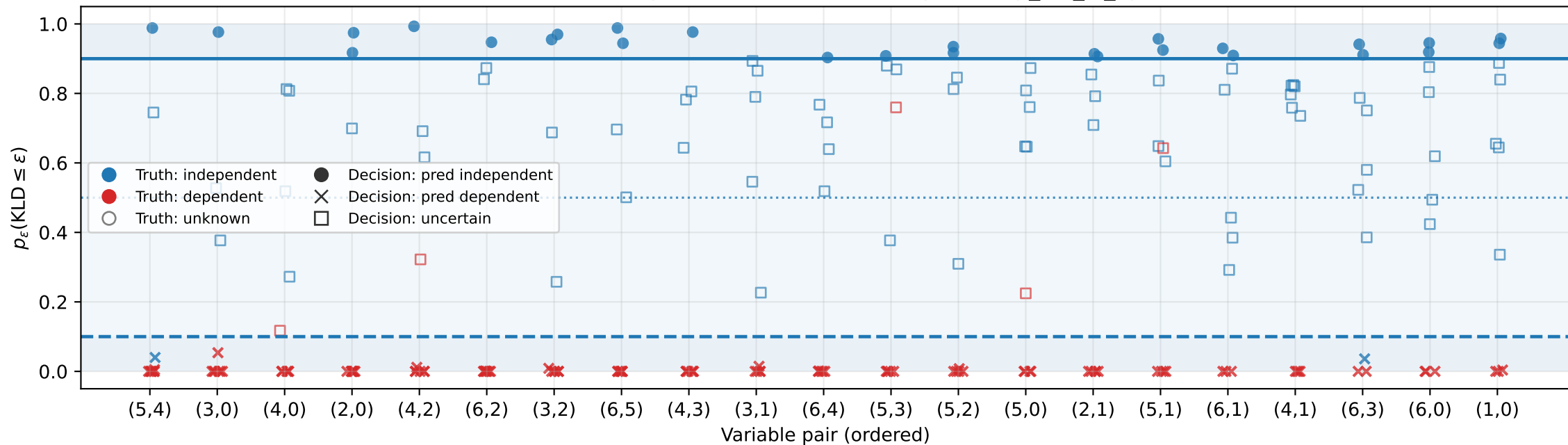
Posterior practical-independence probability per pair across seeds C-Vine • d=7 • ind-tree=2 • n=1000 • BGTM • \epsilon=0.001 , \gamma=0.90 • Pairs ordered by mean( p_{\text{kld\_le\_eps}} ) across seeds.
