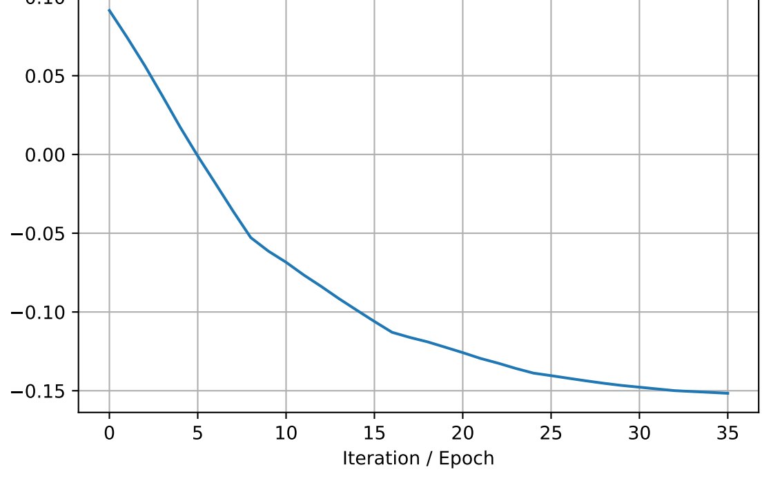
sigma_min
