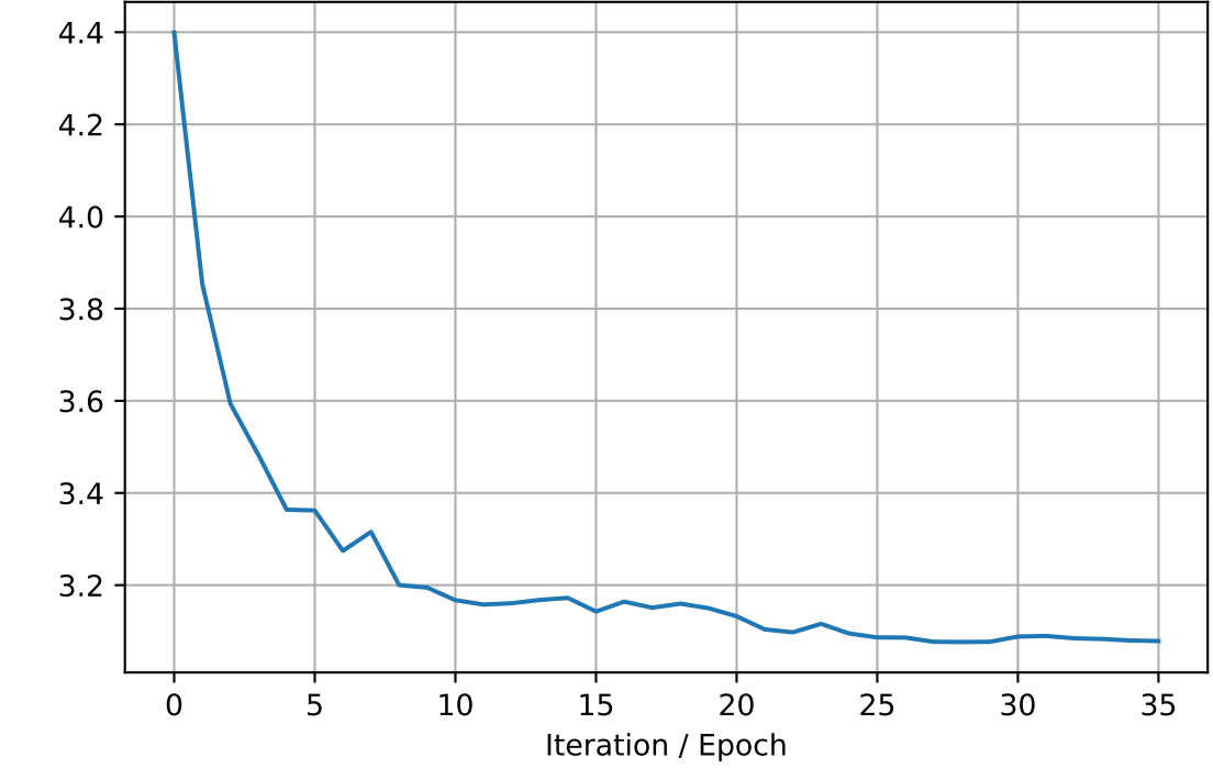
tau1_var
