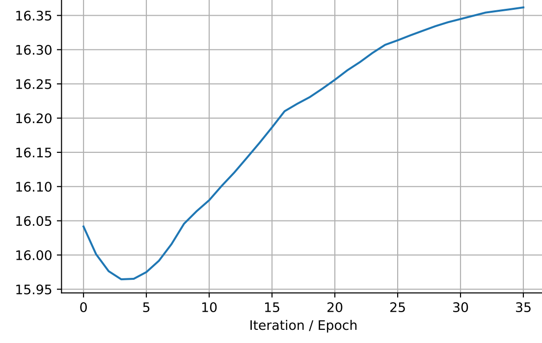
sigma_mean
