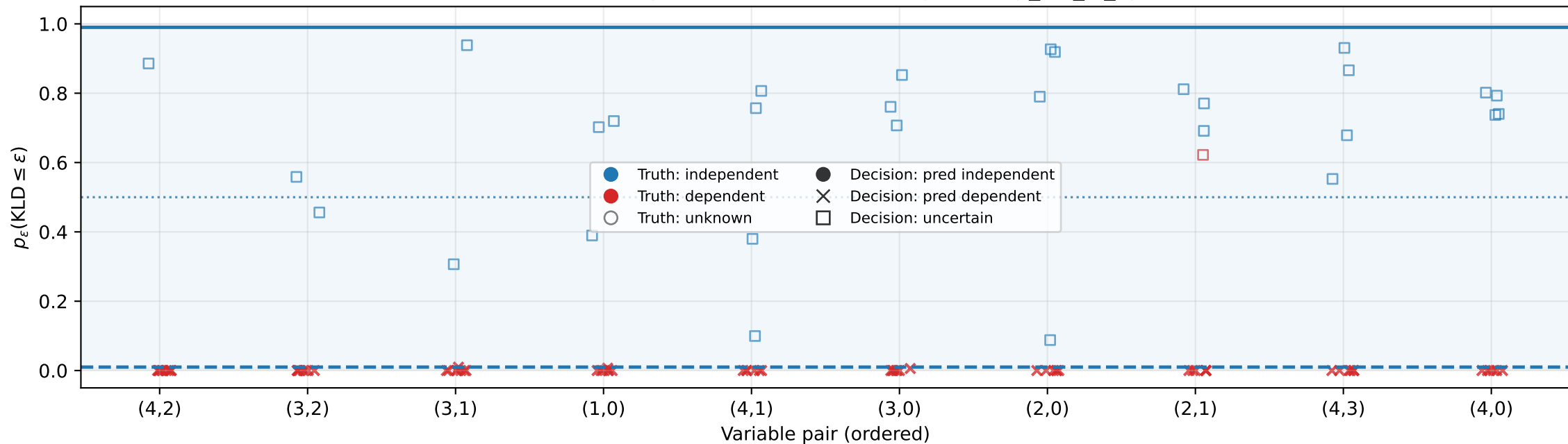
Posterior practical-independence probability per pair across seeds D-Vine • d=5 • ind-tree=2 • n=1000 • BGTM • \epsilon=0.001 , \gamma=0.99 • Pairs ordered by mean( p_{\text{kld\_le\_eps}} ) across seeds.
