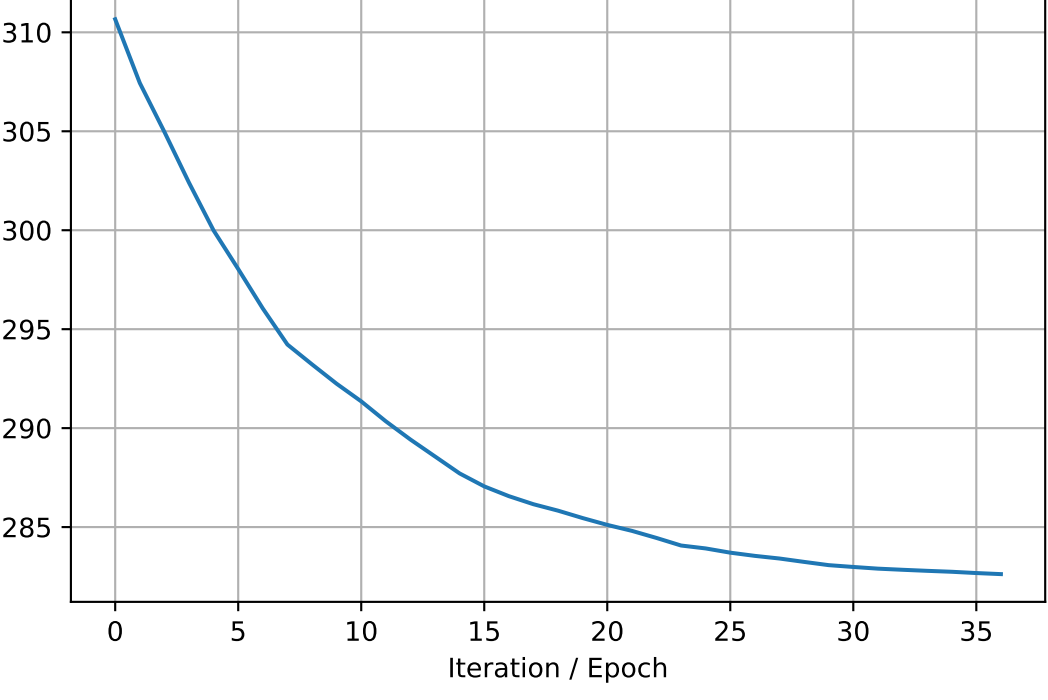
sigma_max
