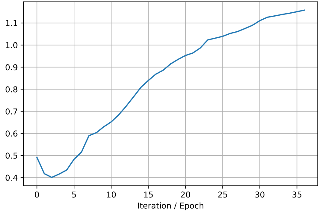
tau1_target
