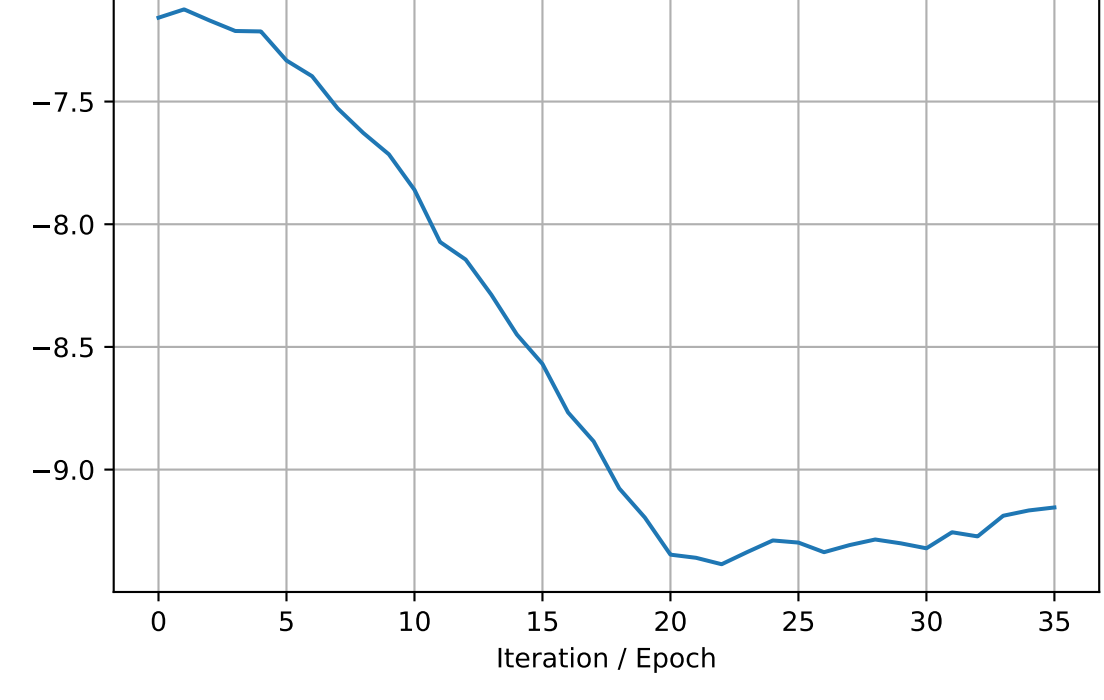
elbo_per_obs
