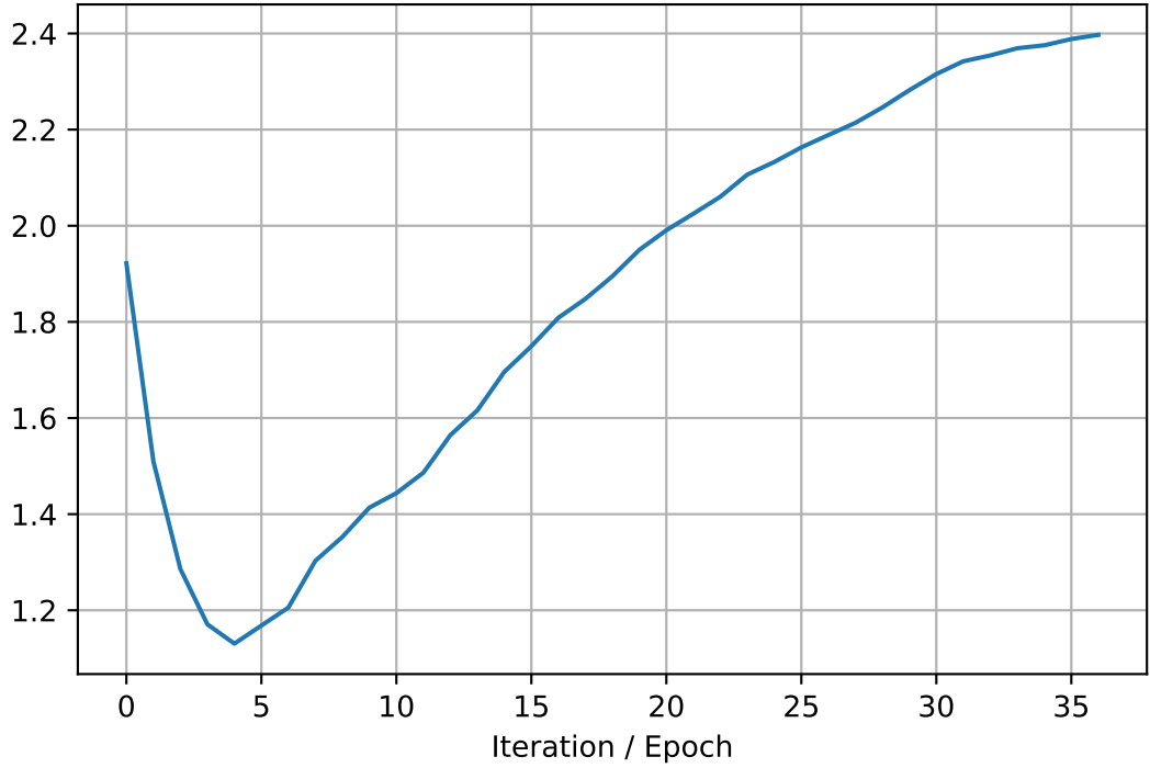
tau2_target
