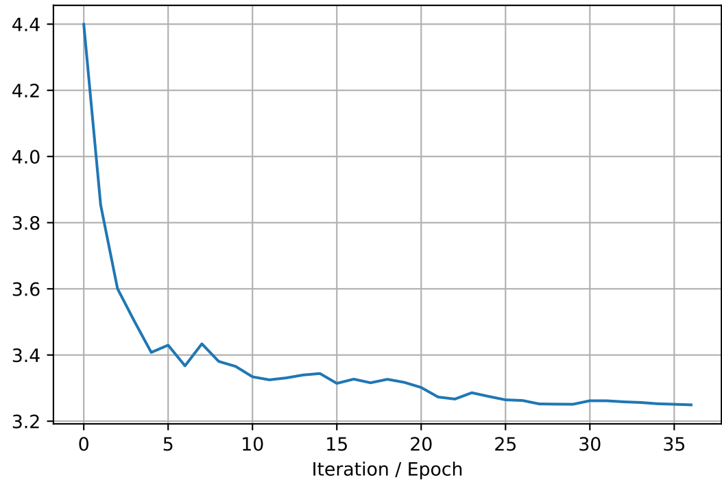
tau1_var
