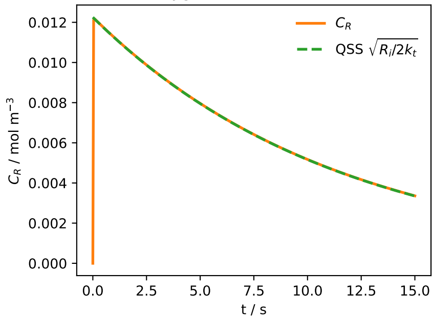
Oxygen-free QSS radicals
