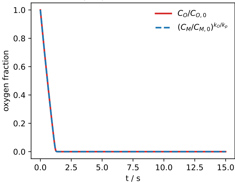
Slutzky Eq. 3 (constant-rate fork)
