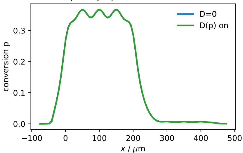
G0|G80 grayscale (thin film in x)
