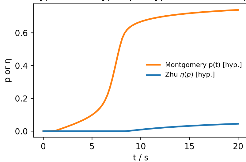
Hypothetical Type-I p \rightarrow Type-II network map
