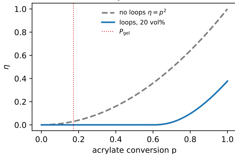
Hypothetical Type-I p \rightarrow Type-II network map
