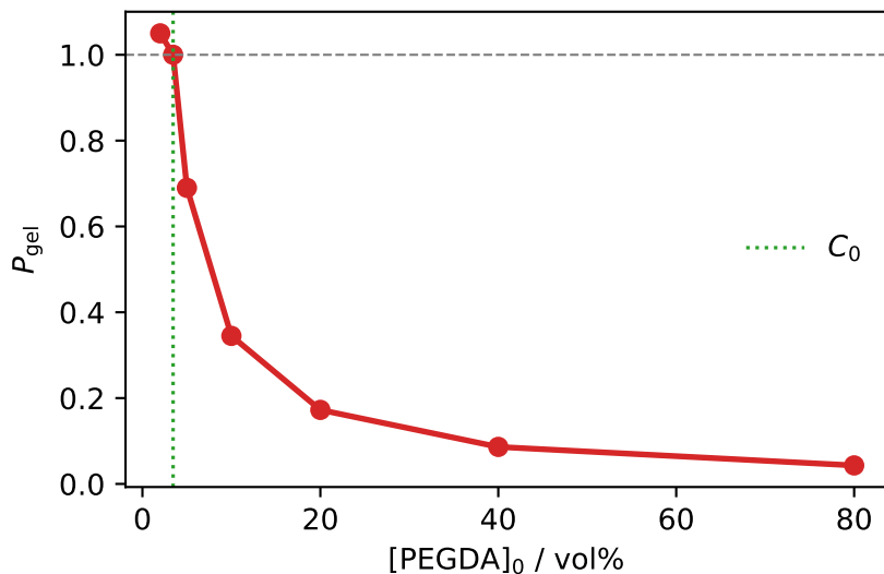
Phantom modulus (Eq. 38)
