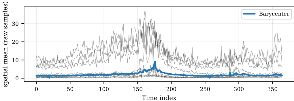
class_0 [eucl_raw] — barycenter + samples
