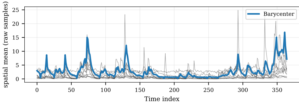
class_3 [eucl_raw] — barycenter + samples
