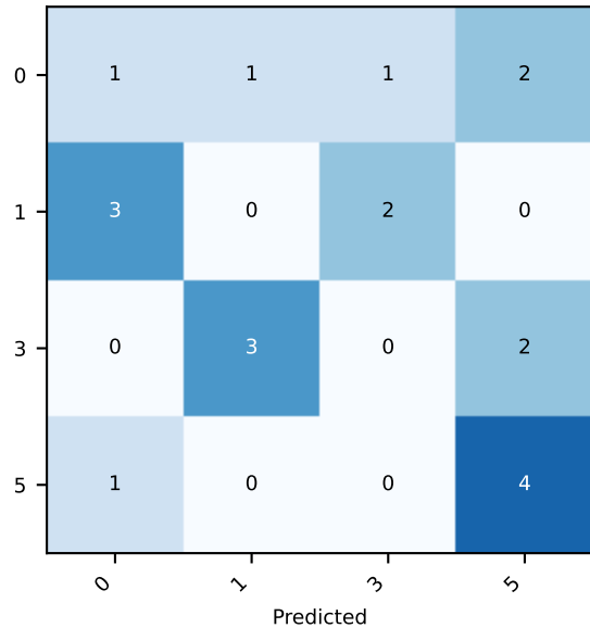
eucl_params f1=0.204
