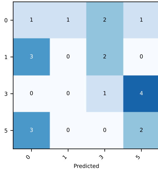
wasps f1=0.175
