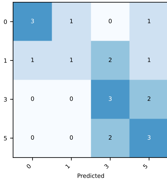
wasps f1=0.488
