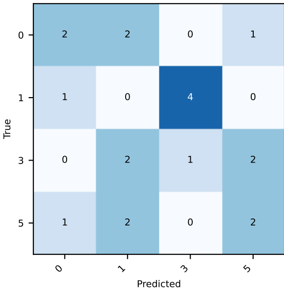
eucl_params f1=0.261
