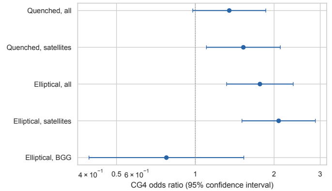
Fig. 2. Adjusted CG_4 odds ratios for the unique star-formation and morphology outcomes in the pooled secondary models, including all-galaxy, satellite-only, and BGG-only rows. Bars show 95% confidence intervals; the vertical line marks equal odds.
