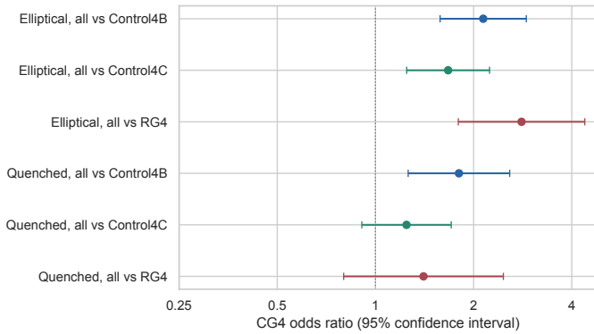
Fig. 1. Adjusted CG_4 odds ratios from the three separate per-control contrasts (colour-coded by control sample) for the all-member elliptical and quenched outcomes. Bars show 95% confidence intervals; the vertical line marks equal odds.
