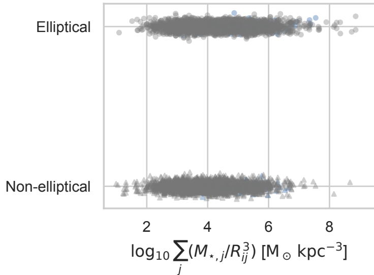
Elliptical morphology
