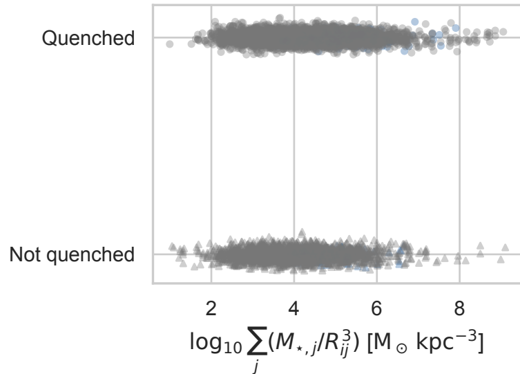
Quenched status
