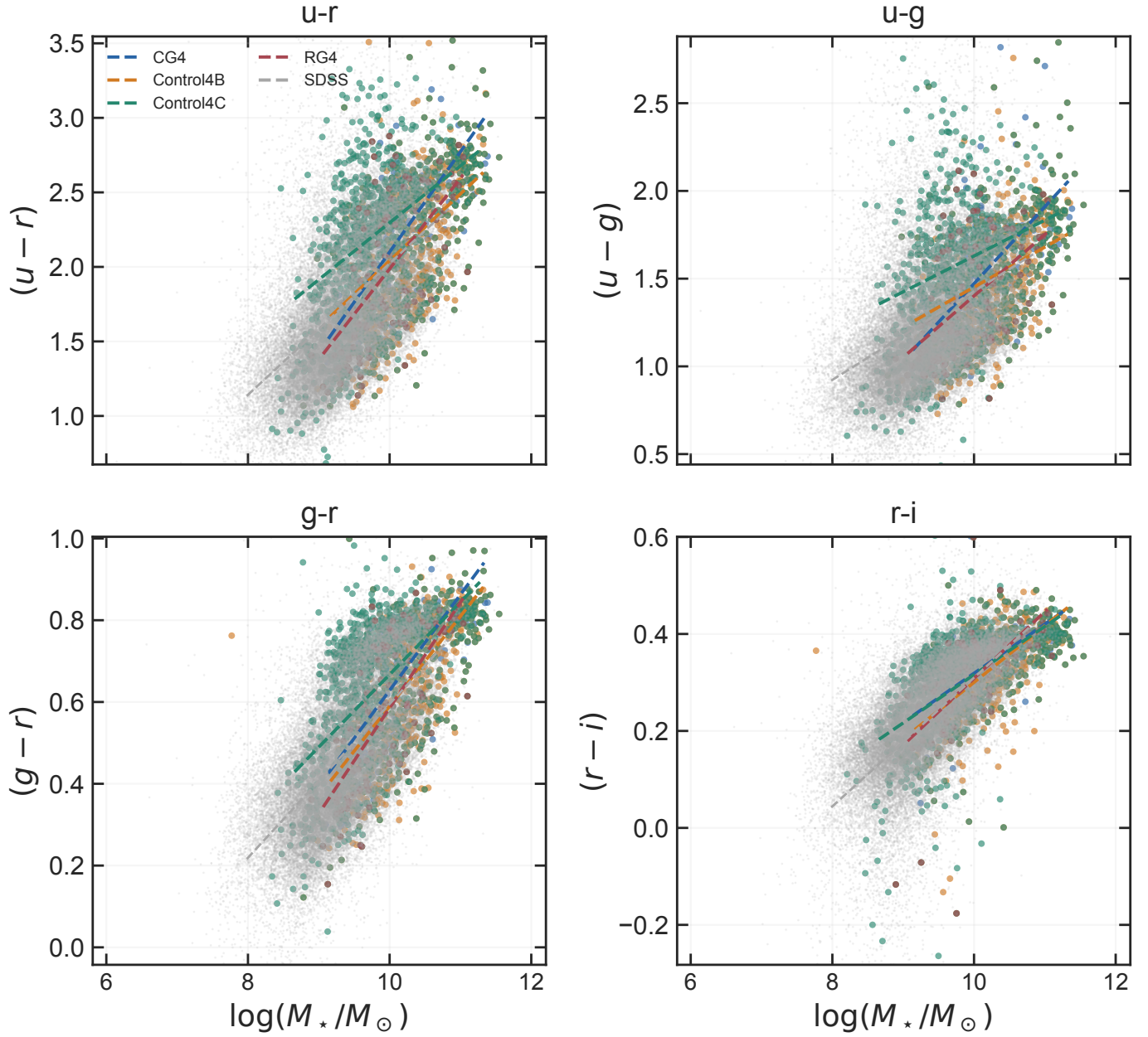
Fig. E.6. Optical colour as a function of stellar mass for CG 4 , the three control catalogues, and the matched SDSS reference sample. Dashed lines show the fitted catalogue relations.
