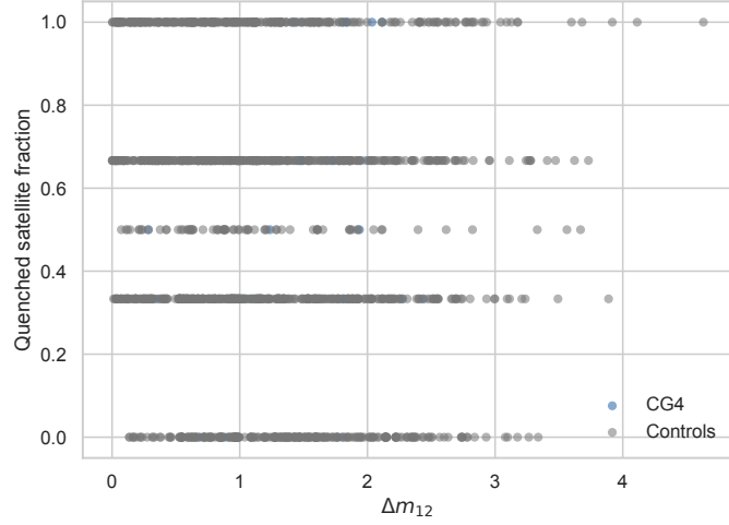
Fig. F.9. Quenched satellite fraction as a function of the first–second magnitude gap.
