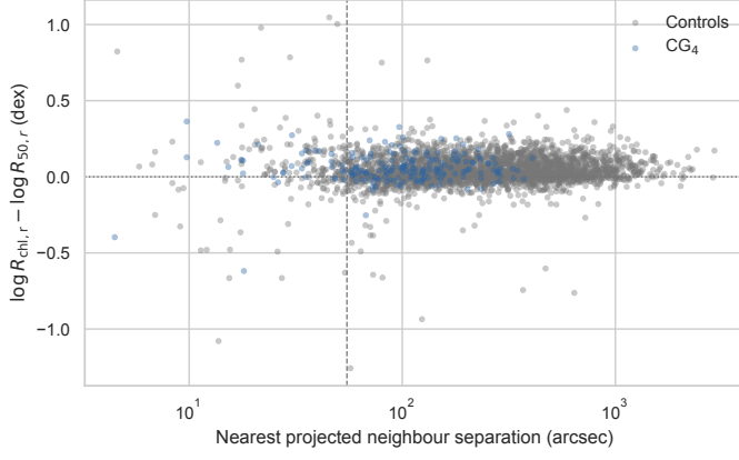
Fig. G.4. Per-galaxy difference between the Simard and Petrosian log half-light radii as a function of nearest projected neighbour separation. The dashed line marks the 55-arcsec crowding scale.
