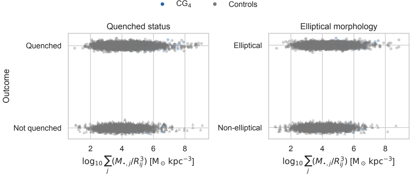
Fig. F.4. Quenched status and elliptical morphology as functions of the reconstructed pairwise tidal index. Colours distinguish CG 4 from control galaxies.
