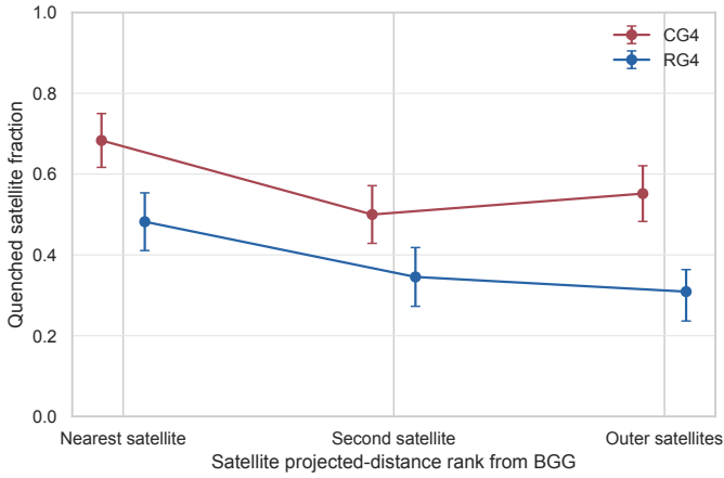
Fig. F.5. Quenched satellite fraction as a function of projected-distance rank from the BGG. Points show CG 4 and RG 4 fractions; bars show group-cluster bootstrap 16th–84th percentile intervals.
