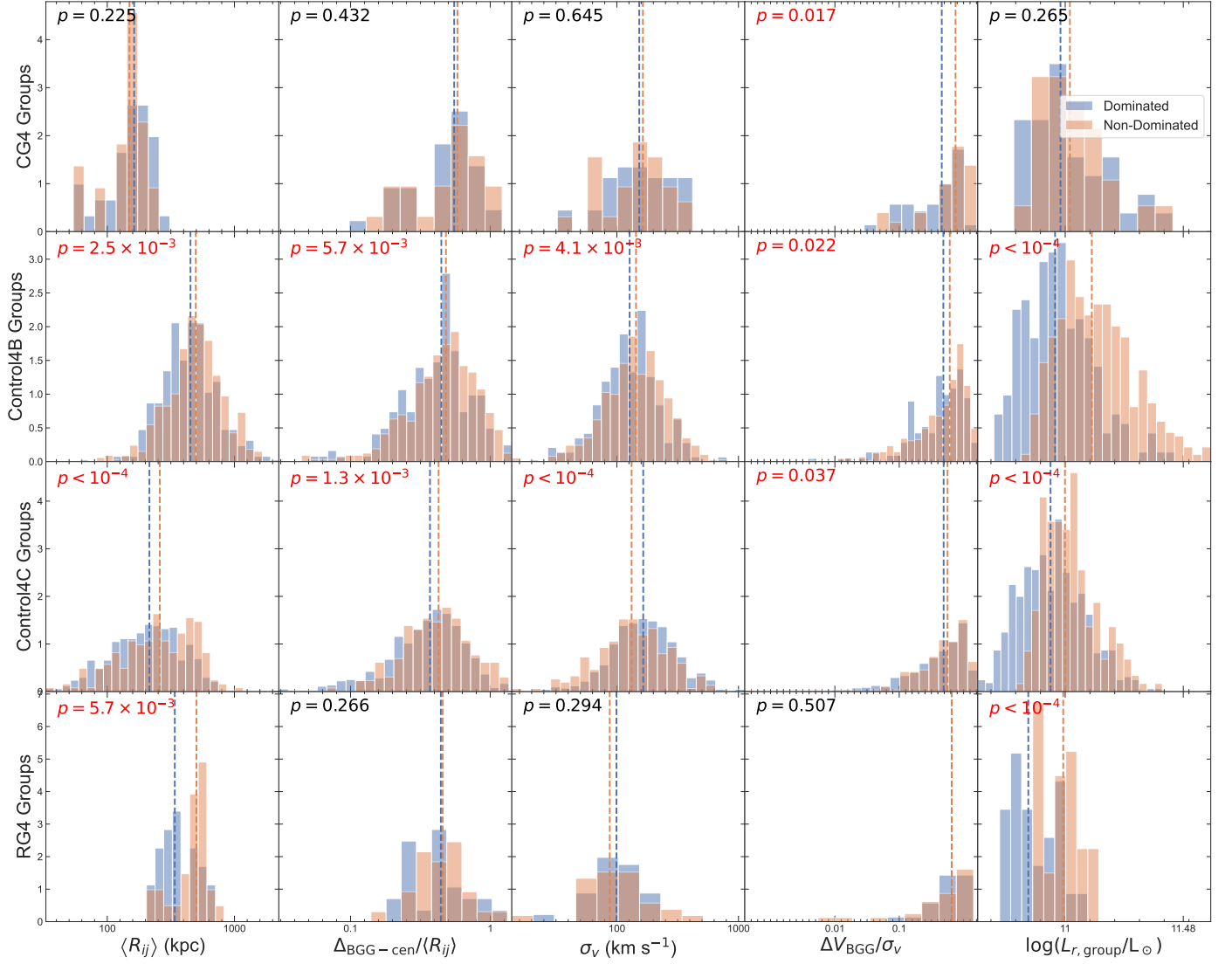
Fig. E.3. Distributions of the main group-scale observables in dominated and non-dominated systems.
