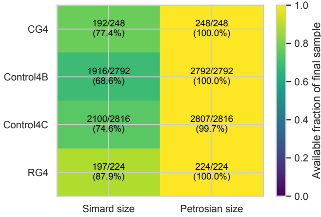
Fig. G.1. Availability of the seeing-corrected Simard half-light radius and the Petrosian half-light radius in each sample, after the bridge, quality, and blending cuts of Sect. 2.3.
