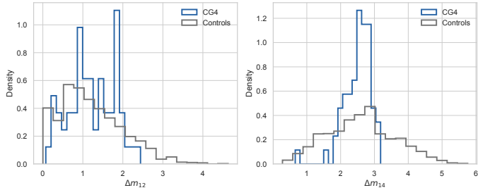
Fig. F.8. Distributions of the first–second and first–fourth magnitude gaps in CG 4 and the pooled controls.
