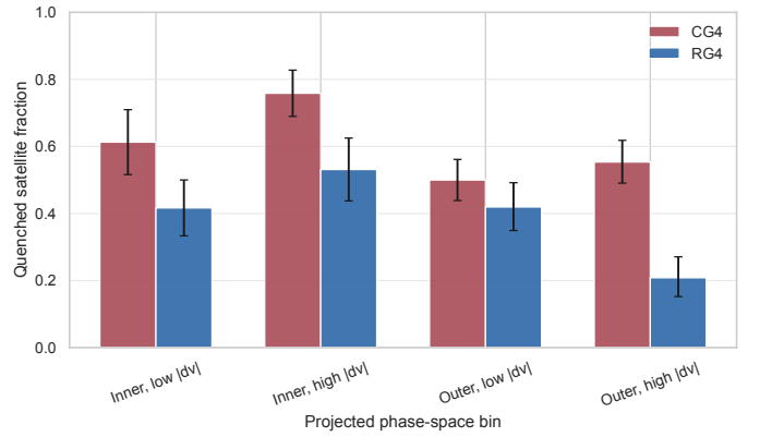
Fig. F.7. Quenched satellite fraction in coarse projected phase-space bins. Inner and outer refer to projected-distance rank from the BGG; low and high velocity are split at |\Delta v_{\text{BGG}}|/\sigma_v = 1 .
