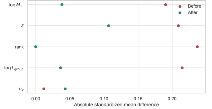
Fig. F.2. Absolute standardized mean differences before and after matching.
