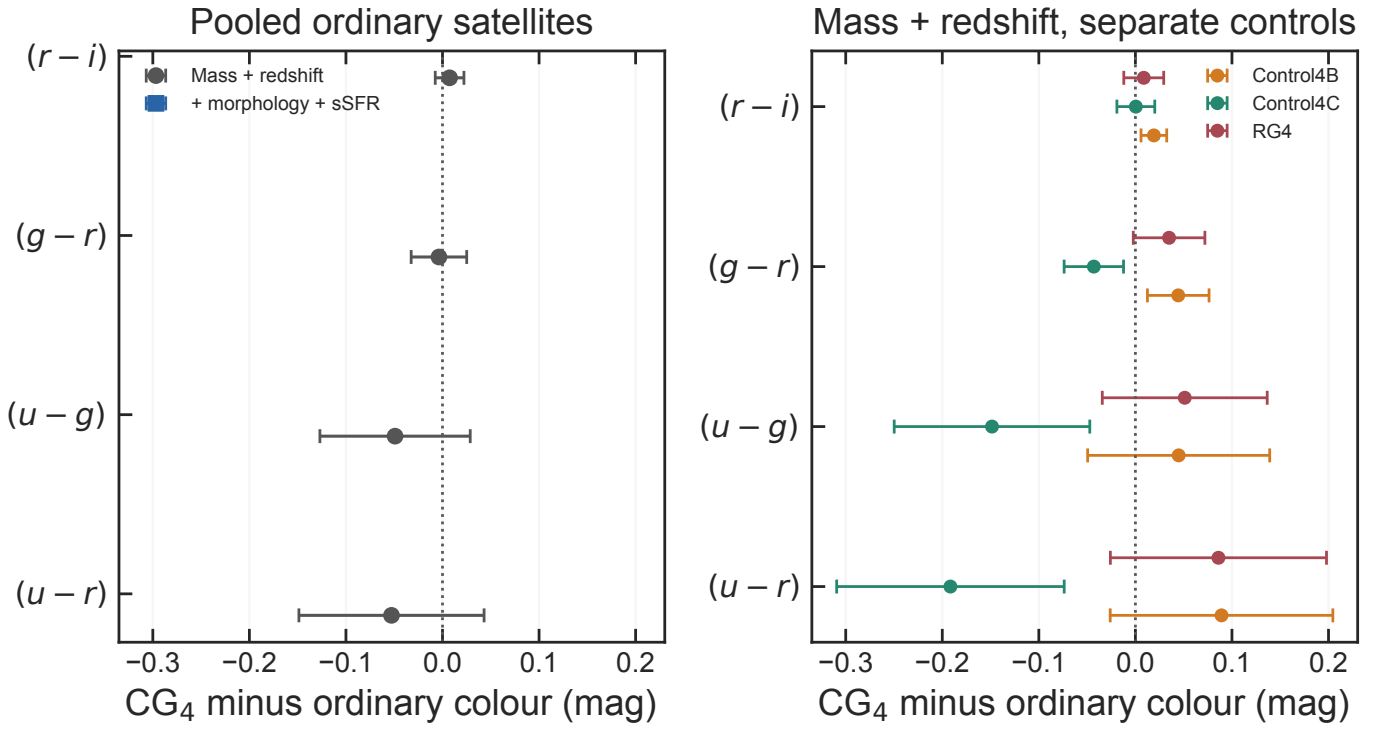
Fig. E.5. Robustness of the satellite colour coefficients. Left: pooled ordinary-group comparison before and after controlling for morphology and sSFR class. Right: mass- and redshift-adjusted comparisons against each control catalogue separately. Points show the CG_4 minus ordinary coefficient and bars show 95% confidence intervals; negative values indicate bluer CG_4 satellites.
