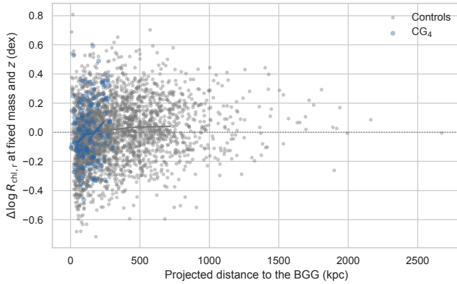
Fig. G.6. Mass- and redshift-adjusted satellite size residuals versus projected distance to the BGG. Lines connect binned medians for CG_4 and the pooled controls.
