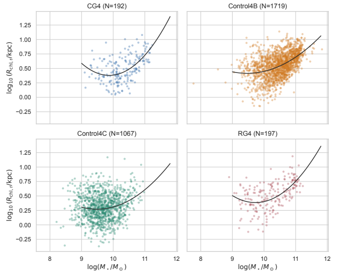
Fig. G.2. Seeing-corrected half-light radius versus stellar mass in each sample. Solid curves show the descriptive quadratic fits used to quote a predicted size at the reference stellar mass.
