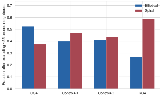
Fig. F.3. Galaxy Zoo morphology fractions after excluding galaxies with a nearest projected neighbour within 55 arcsec. The CG 4 elliptical excess persists after this closest-neighbour exclusion.
