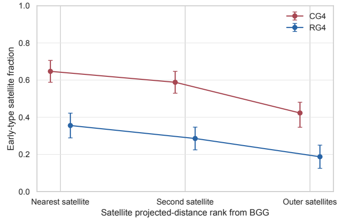
Fig. F.6. Early-type satellite fraction as a function of projected-distance rank from the BGG. Because the catalogue separates ellipticals, spirals, and uncertain morphologies but not S0 galaxies, early type is equivalent to elliptical in this diagnostic.
