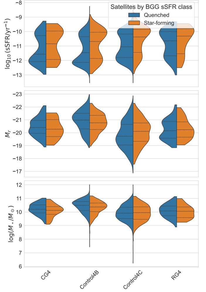
Fig. D.4. Distributions of various quantities for satellites according to the BGG sSFR class.
