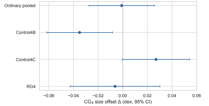
Fig. G.3. Mass- and redshift-adjusted CG 4 size coefficients against the pooled controls and against each control catalogue separately. Bars show 95% confidence intervals; negative values mean smaller CG 4 sizes at fixed mass.
