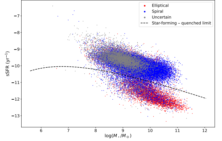
Fig. B.2. sSFR versus stellar mass, the star-forming/quenched limit, and Galaxy Zoo morphologies for the SDSS selection, excluding galaxies without sSFR estimates.
