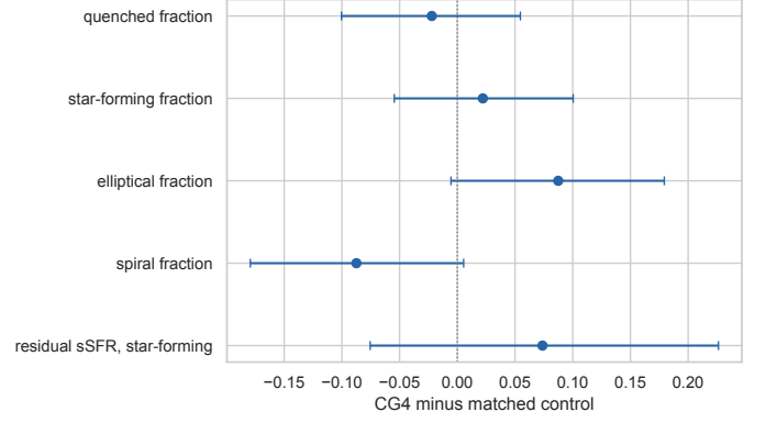
Fig. F.1. CG 4 -minus-control effects after one-to-one matching. Bars show 95% bootstrap confidence intervals.
