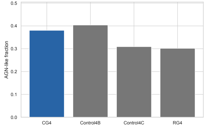
Fig. F.11. AGN-like fractions among galaxies with BPT-classifiable emission-line ratios. BPT-unclassified galaxies are not counted as non-AGN in this diagnostic.
