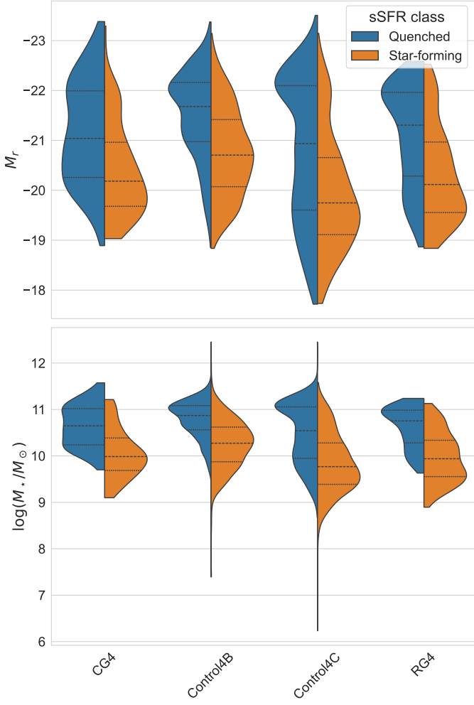
Fig. D.3. Distributions of various quantities for galaxies according to their sSFR class.
