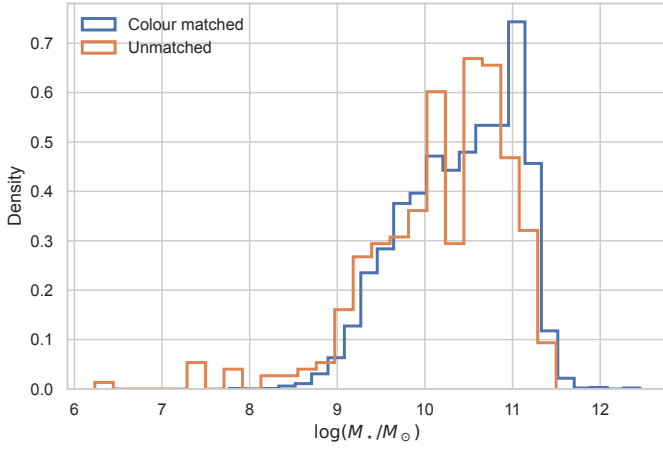
Fig. F.13. Stellar-mass distributions of galaxies with and without complete matched colour measurements.
