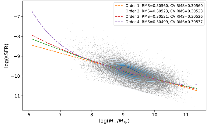
Fig. D.5. Polynomial fits of orders 1–4 to the star-forming main sequence. The legend reports residual RMS and five-fold cross-validated RMS scatter in dex; order 2 is adopted because it is the lowest-order model with the smallest cross-validated RMS scatter.
