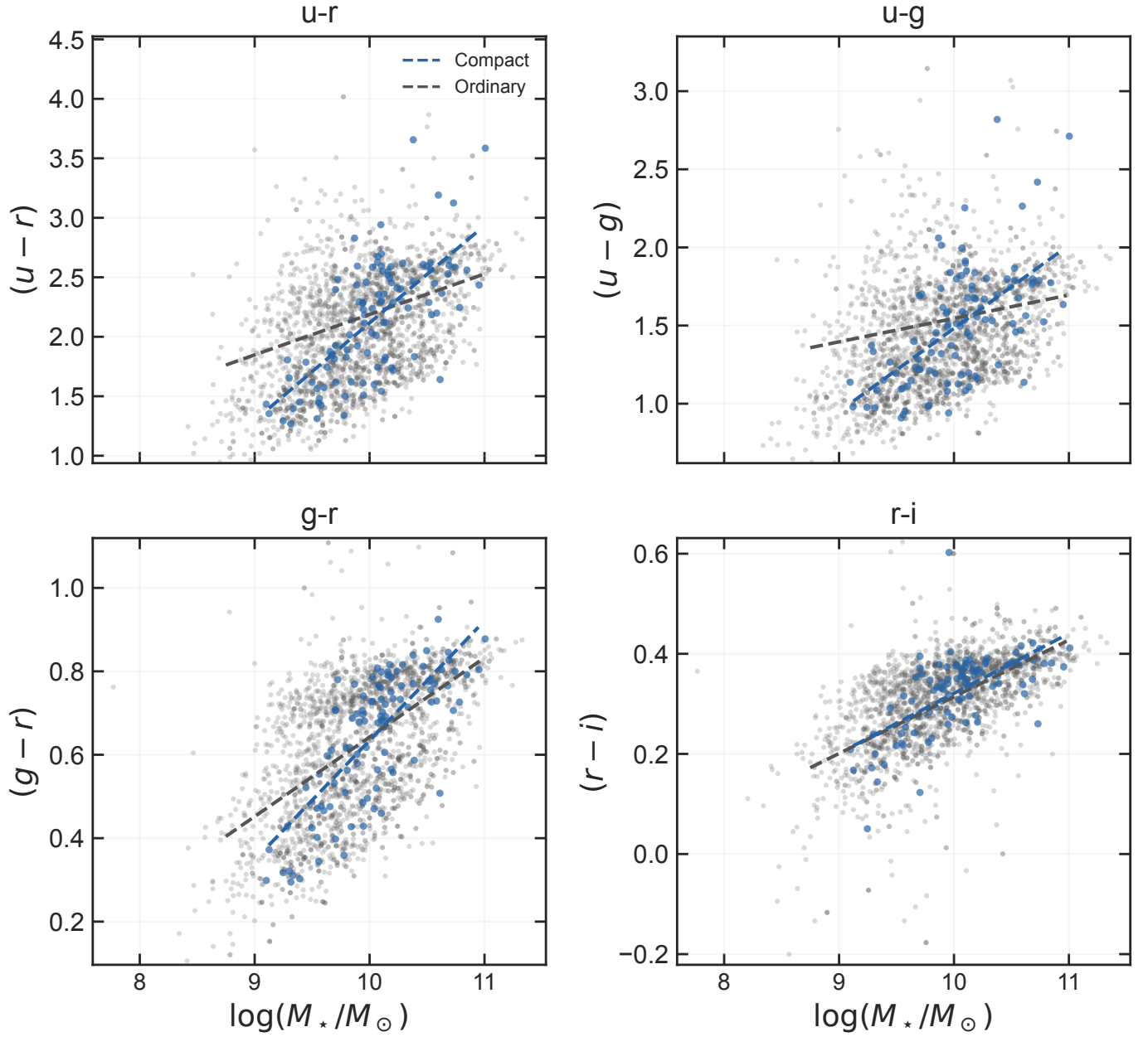
Fig. E.7. Satellite colour-mass relations in compact and ordinary groups. The fitted lines show both colour offsets at the reference mass and differences in slope.
