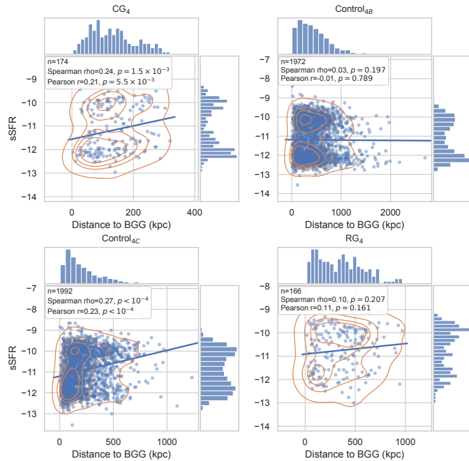
Fig. E.1. sSFR as a function of projected distance to the BGG, in kpc, for satellite galaxies in each sample.
