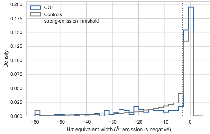
Fig. F.10. H \alpha equivalent-width distributions used for the limited recent-quenching diagnostic.
