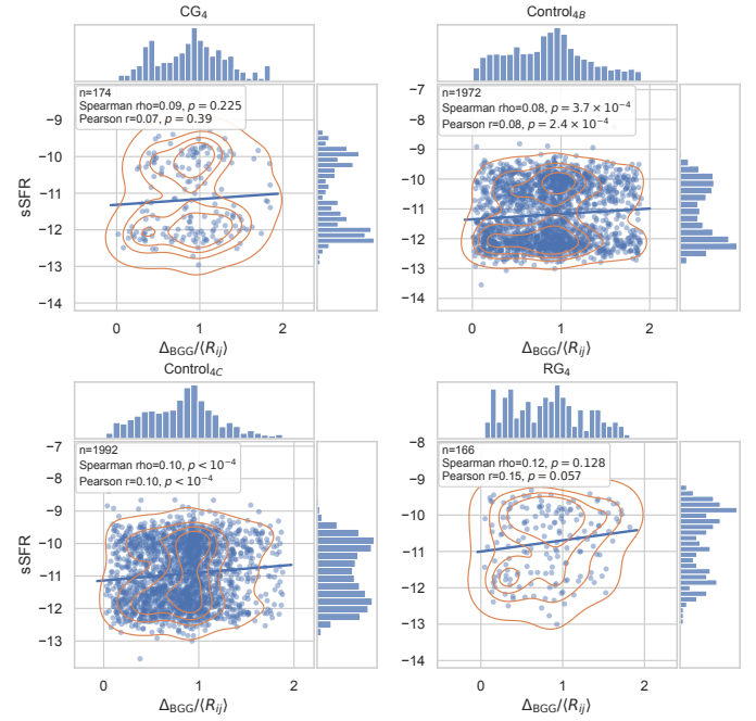
Fig. E.2. sSFR as a function of projected distance to the BGG normalized by \langle R_{ij} \rangle for satellite galaxies in each sample.
