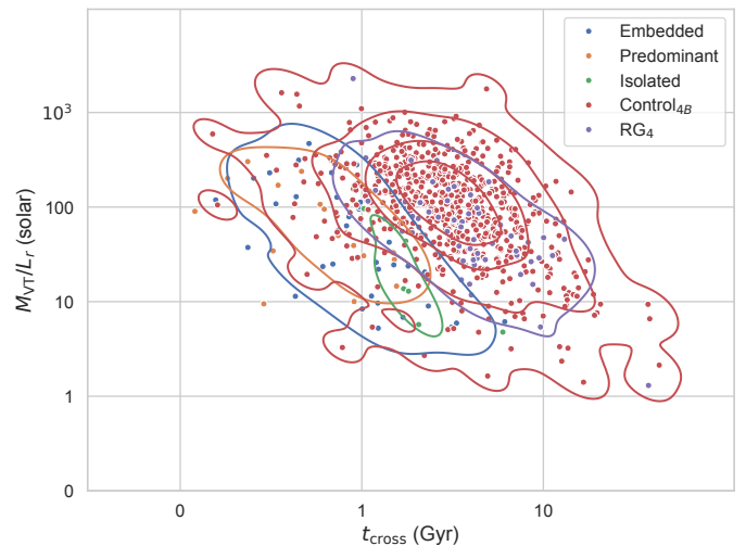
Fig. E.4. Crossing time versus virial mass-to-light ratio for the compact groups and their controls.
