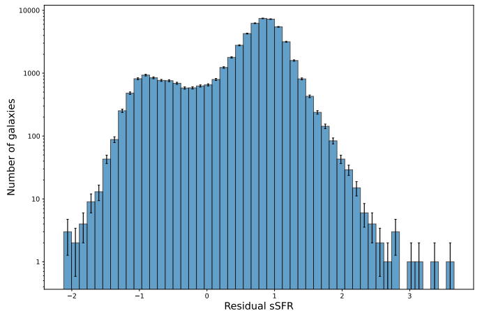
Fig. D.2. Distribution of residual sSFR offsets from the adopted star-forming main sequence.
