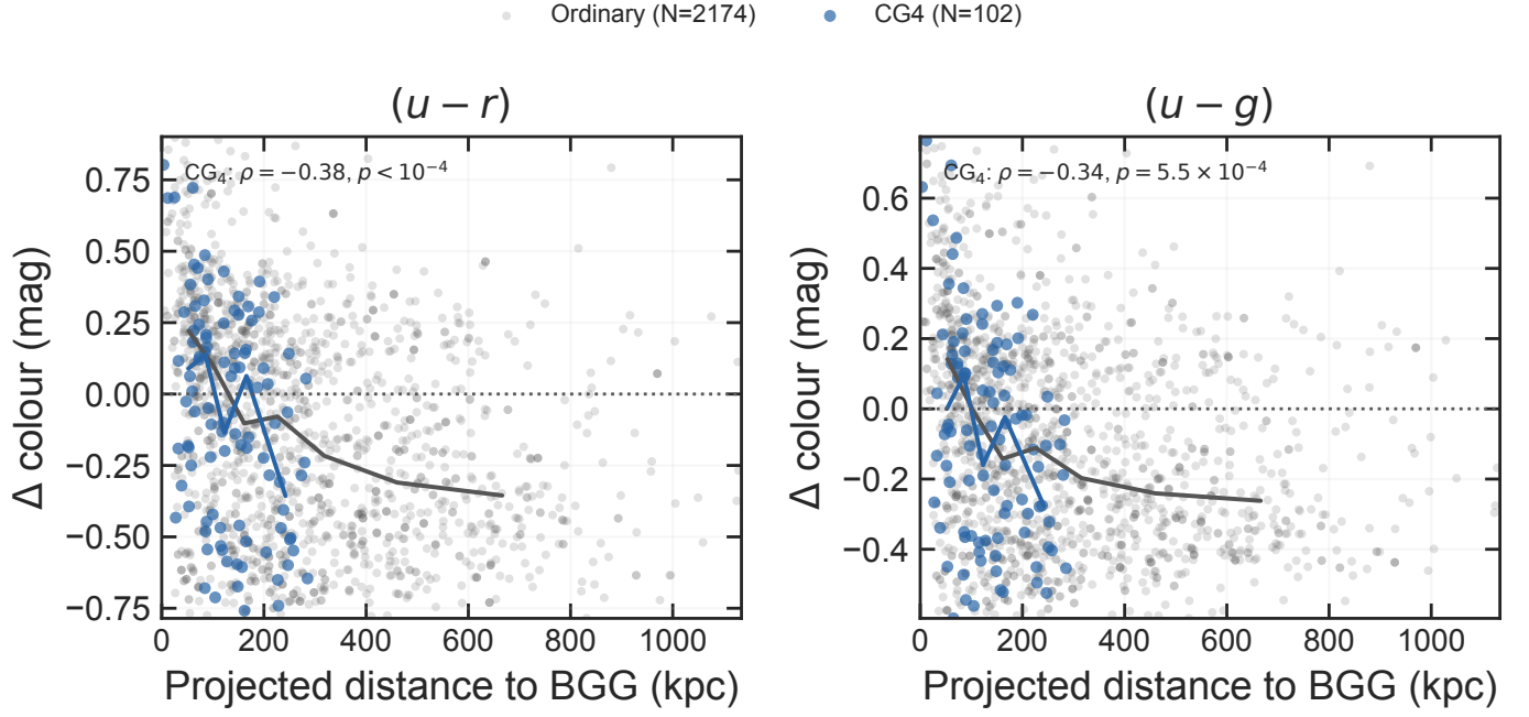
Fig. E.8. Mass- and redshift-adjusted satellite (u-r) and (u-g) residuals as a function of projected distance to the BGG. Lines connect binned medians for CG 4 and the pooled ordinary-group satellites; extreme plotting tails are omitted for readability, while the reported rank correlations use the full matched sample. More negative residuals are bluer than the ordinary-satellite reference relation.
