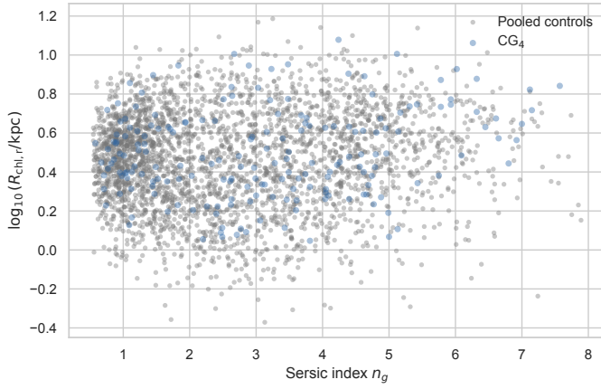
Fig. G.5. Half-light radius versus Sérsic index for CG_4 and the pooled controls, shown for galaxies with both valid Simard size and stellar mass in the mass-size analysis. This is the plane used by the S-PLUS transition-galaxy studies.
