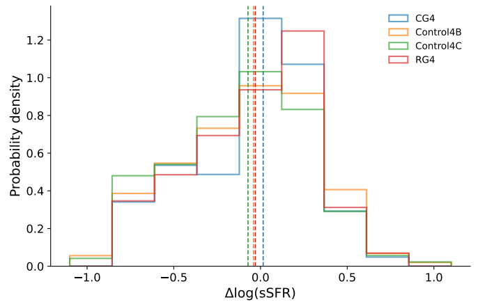
Fig. D.1. Main-sequence residual distributions for the star-forming galaxies in each sample.
