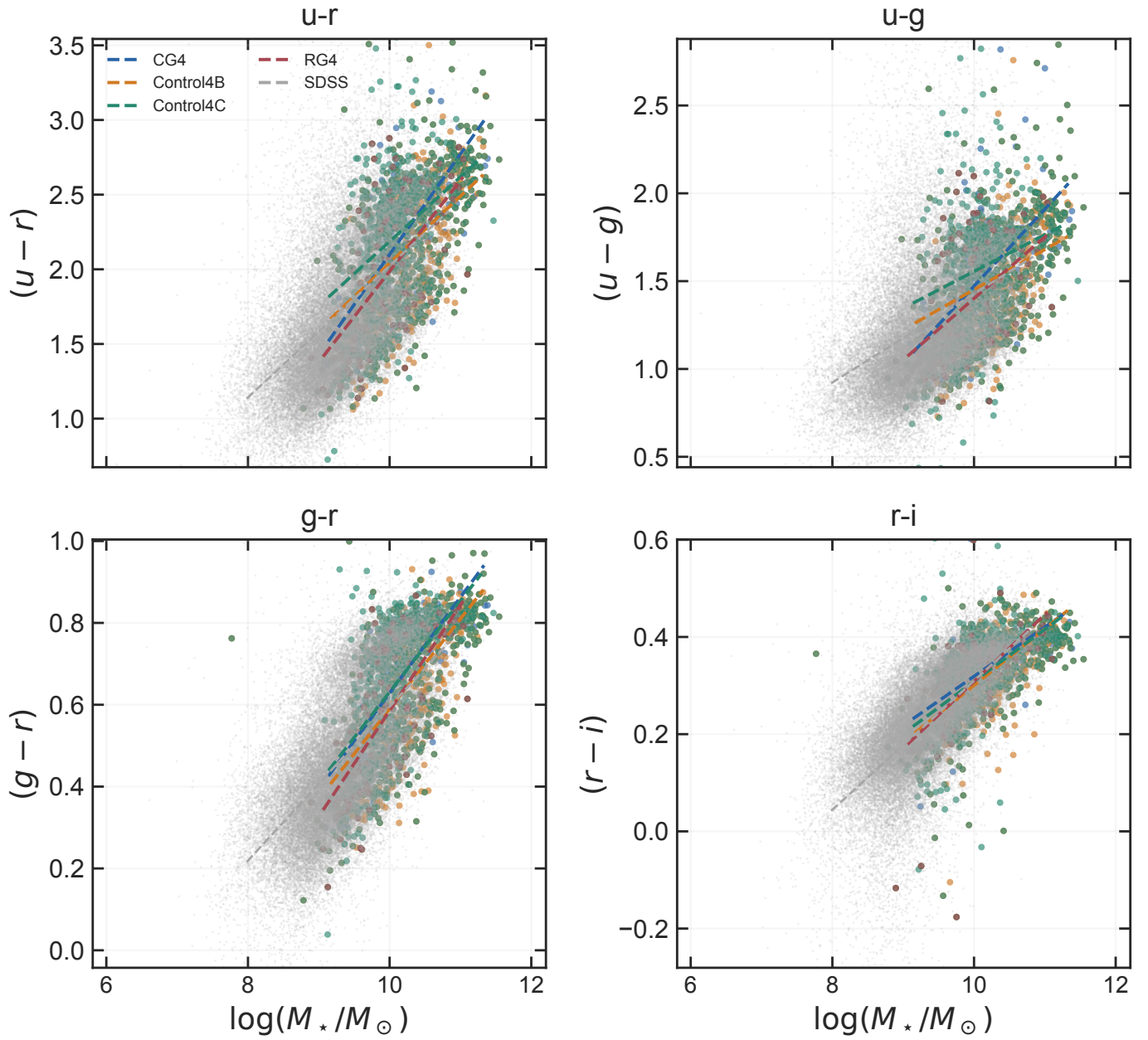
Fig. S.4. Colour–stellar-mass relations in the four catalogues. These raw relations motivate the control-specific adjusted comparisons rather than a single pooled interpretation.
