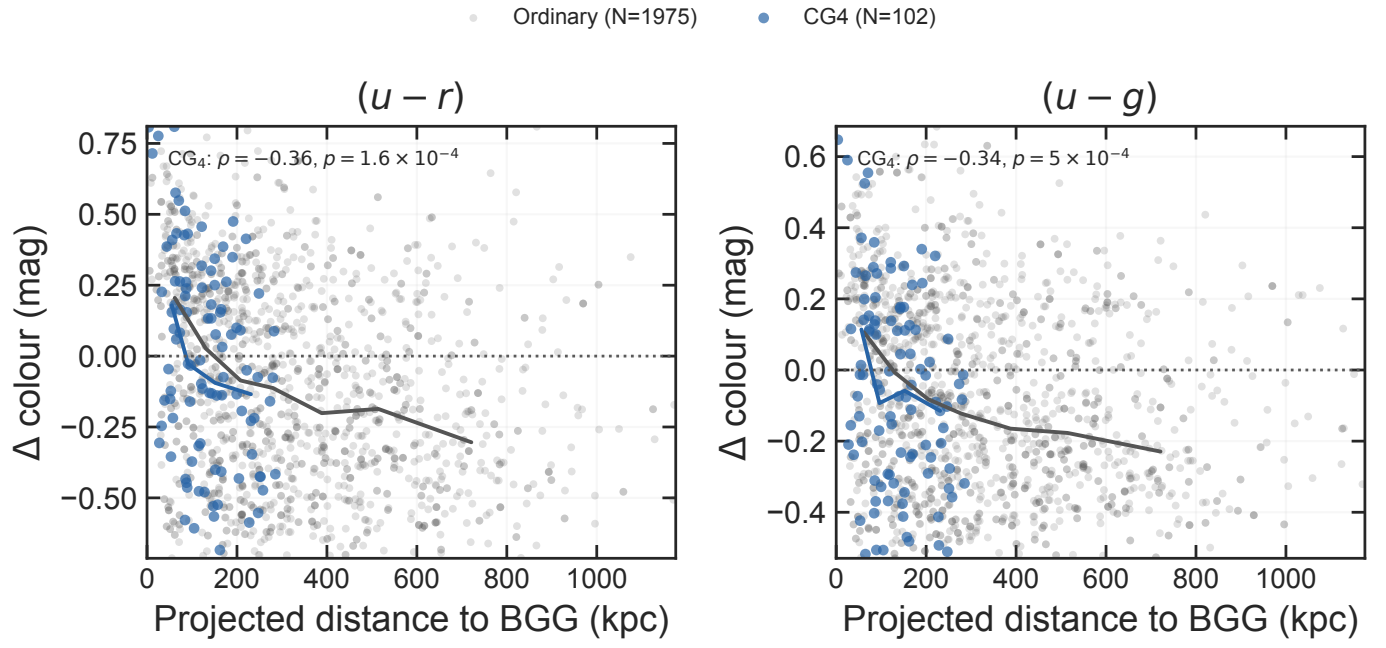
Fig. S.6. Colour residuals versus projected BGG-centric distance. These trends are exploratory and inherit the matched-photometry selection described above.
