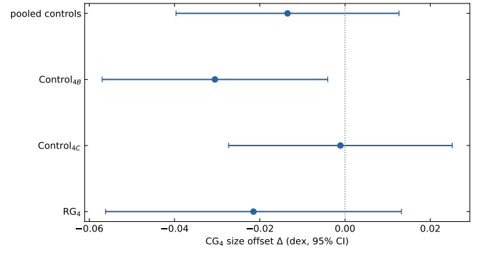
Fig. S.8. Group-adjusted CG_4 size coefficients against the deduplicated pooled controls and each control catalogue separately. Every model uses the article's main adjustment set: stellar mass, redshift, rank, group luminosity, and velocity dispersion, with physical-group-clustered uncertainties. Bars are 95% confidence intervals; negative values denote smaller CG_4 effective radii at fixed covariates.
