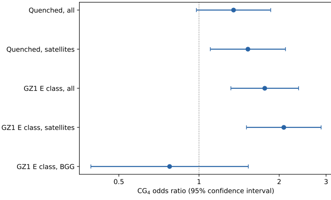
Fig. S.7. Adjusted CG_4 odds ratios from the pooled models. The GZ1 E-class outcomes refer to the smooth early-type-like GZ1 class, not to a physically pure sample of classical ellipticals. Points are odds ratios and bars are cluster-robust 95% confidence intervals; the vertical line marks no difference.
