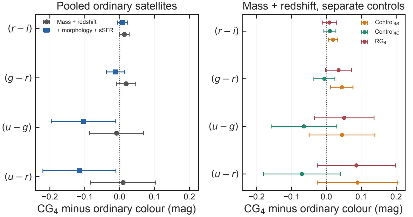
Fig. S.3. Robustness of the satellite colour coefficients. Left: pooled ordinary-group comparison before and after controlling for GZ1 E/S morphology and sSFR class. Right: mass- and redshift-adjusted comparisons against each control catalogue separately. Points show the CG_4 minus ordinary-group coefficient and bars show 95% confidence intervals; negative values indicate bluer CG_4 satellites.
