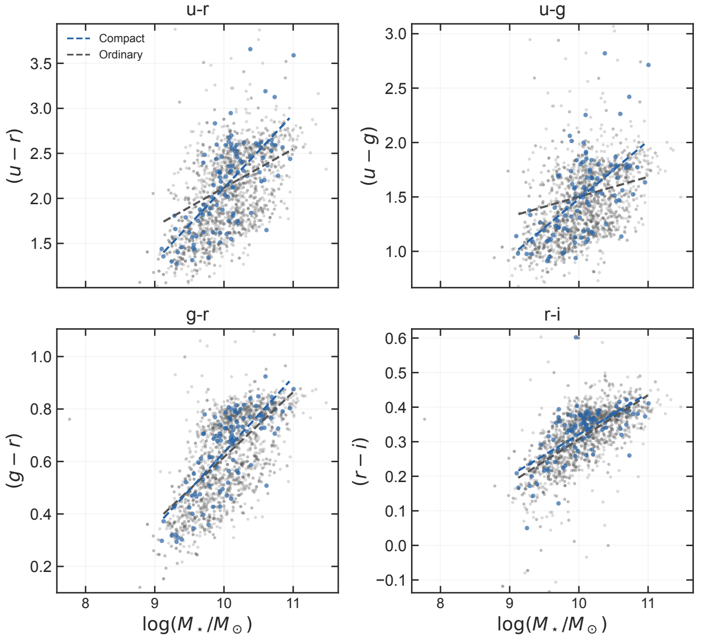
Fig. S.5. Satellite colour–mass relations split by environment. The offsets and slopes depend on the comparison catalogue.
