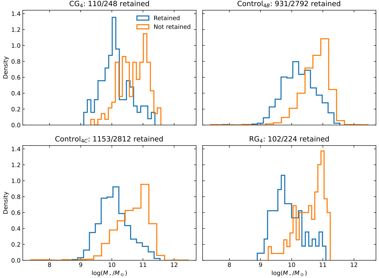
Fig. S.2. Stellar-mass selection diagnostics for the exact colour-analysis retained population versus galaxies not retained, shown separately by sample. Retained counts are 110/248 for \text{CG}_4 , 931/2792 for \text{Control}_{4B} , 1153/2812 for \text{Control}_{4C} , and 102/224 for \text{RG}_4 . These are the same retained galaxies used by the colour analysis. Histograms are density-normalised within each retained or non-retained subset.
