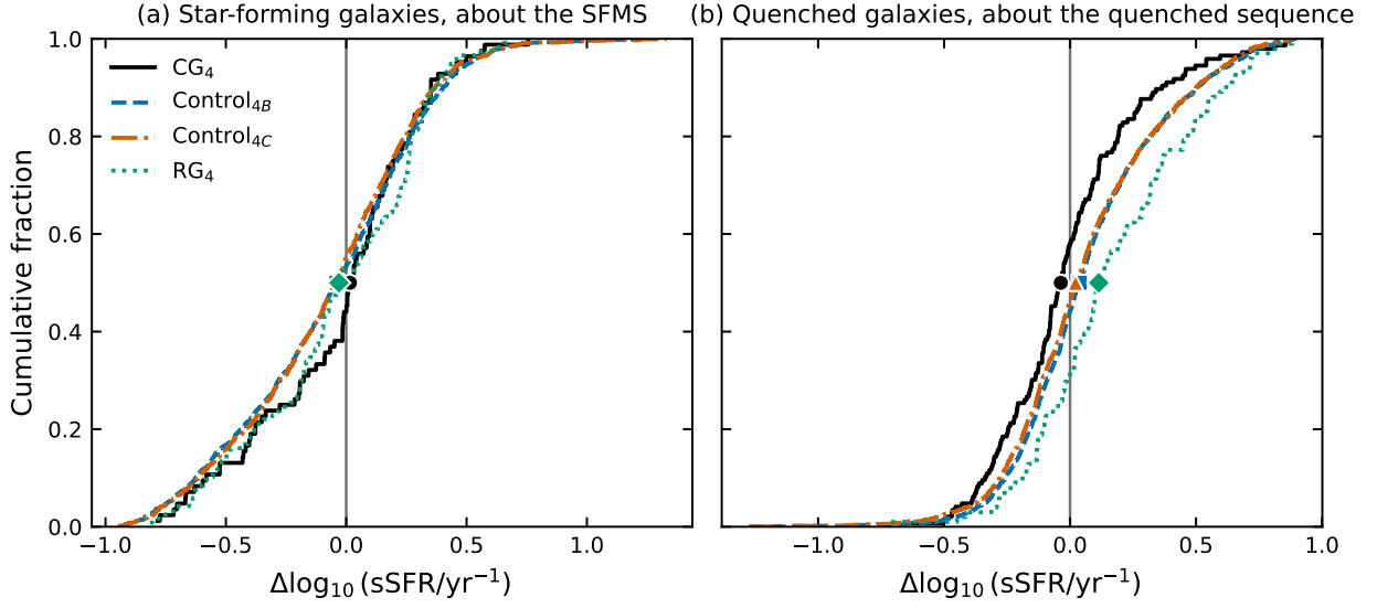
Fig. S.1. Cumulative distributions of the sSFR residuals of (a) star-forming galaxies about the order-2 star-forming main sequence and (b) quenched galaxies about the order-4 quenched sequence, both fitted to the SDSS non-AGN reference sample. Zero marks the fitted relation; filled symbols mark the sample medians. MPA-JHU sSFRs of quenched galaxies are largely D_n4000 -calibrated, so panel (b) is weakly informative.
