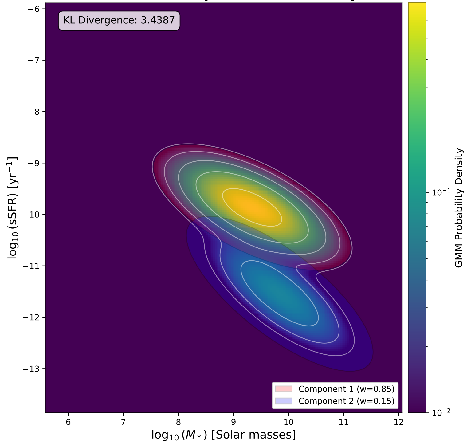
Fitted Two-Component GMM Density
