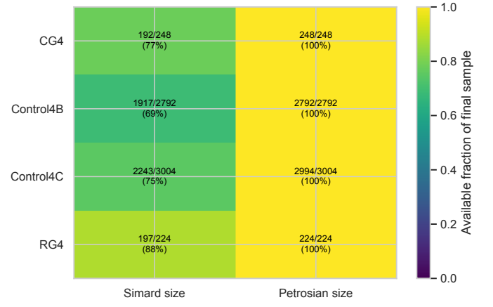
Fig. C.18. Availability of the seeing-corrected Simard half-light radius and the Petrosian half-light radius in each sample, after the bridge, quality, and blending cuts of Sect. 2.5.
