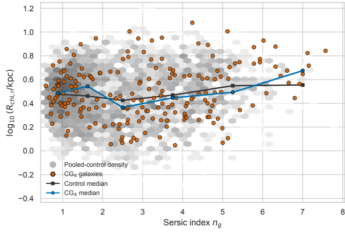
Fig. G.3. Half-light radius versus Sérsic index for CG 4 and the pooled controls, shown for galaxies with both valid Simard size and stellar mass in the mass-size analysis. The pooled controls are shown as a grey logarithmic hexbin density, while CG 4 galaxies are overplotted as foreground points; lines show binned medians where bins are sufficiently populated. This is the plane used by the S-PLUS transition-galaxy studies.
