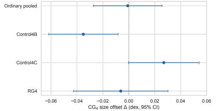
Fig. G.2. Mass- and redshift-adjusted \text{CG}_4 size coefficients against the pooled controls and against each control catalogue separately. Bars show 95% confidence intervals; negative values mean smaller \text{CG}_4 sizes at fixed mass.
