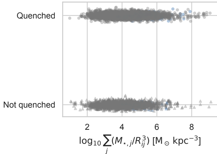
Quenched status
