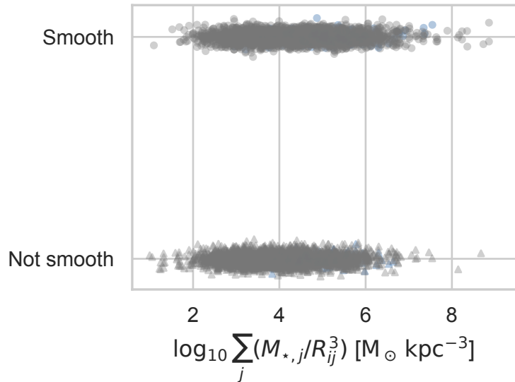
Elliptical/smooth morphology
