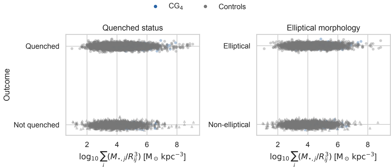
Fig. 12. Quenched status and elliptical morphology as functions of the reconstructed pairwise tidal index. Colours distinguish CG 4 from control galaxies.
