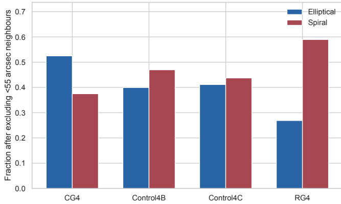
Fig. 7. Galaxy Zoo morphology fractions after excluding galaxies with a nearest projected neighbour within 55 arcsec. The CG 4 elliptical excess persists after this closest-neighbour exclusion.
