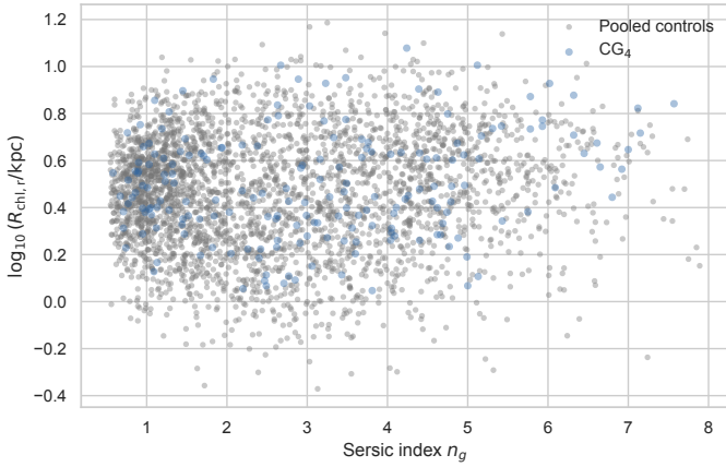
Fig. D.17. Half-light radius versus Sérsic index for CG_4 and the pooled controls, shown for galaxies with both valid Simard size and stellar mass in the mass-size analysis. This is the plane used by the S-PLUS transition-galaxy studies.
