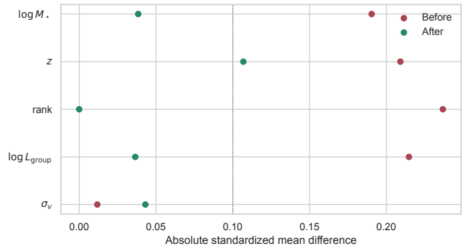
Fig. 9. Absolute standardized mean differences before and after matching.
