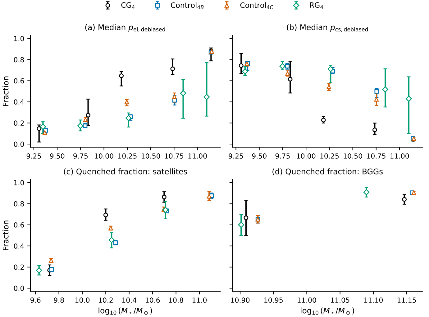
Fig. 2. Galaxy Zoo vote fractions and quenched fractions versus stellar mass. Top: median debiased elliptical and spiral vote fractions for all galaxies. Bottom: quenched fractions among valid-sSFR satellites and BGGs. All samples use the same bins within each row: edges 7.0, 9.5, 10.0, 10.5, 11.0, 12.5 for morphology and 7.0, 10.0, 10.5, 11.0, 12.5 for quenching. Each estimate is plotted at the median stellar mass of the galaxies contributing to it, rather than at the geometric bin centre; points are not connected because the displayed bins have unequal widths. Bars are 16th–84th percentile physical-group-blocked bootstrap intervals; bins with fewer than five galaxies or three groups are omitted.
