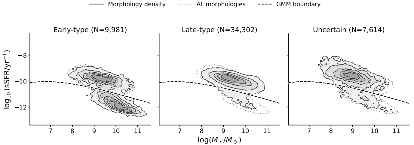
Fig. B.1. Galaxy Zoo morphology in sSFR–stellar-mass space for the SDSS non-AGN reference, excluding galaxies without sSFR estimates. Panels show early-type, late-type, and uncertain morphologies; no unavailable morphologies occur in this reference sample ( N = 0 ). Solid class-specific contours enclose 20, 40, 60, 80, and 95% of the density, grey dotted contours show the full reference distribution at the same enclosed-probability levels, and the dashed curve is the unchanged adopted star-forming–quenched GMM boundary.
