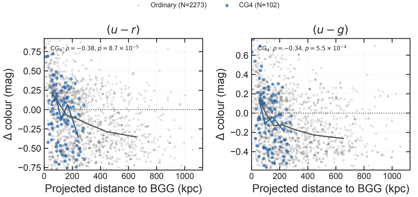
Fig. C.15. Mass- and redshift-adjusted satellite (u-r) and (u-g) residuals as a function of projected distance to the BGG. Lines connect binned medians for CG 4 and the pooled ordinary-group satellites; extreme plotting tails are omitted for readability, while the reported rank correlations use the full matched sample. More negative residuals are bluer than the ordinary-satellite reference relation.
