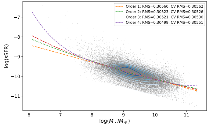
Fig. C.5. Polynomial fits of orders 1–4 to the star-forming main sequence. The legend reports residual RMS and five-fold cross-validated RMS scatter in dex; order 2 is adopted because it is the lowest-order model with the smallest cross-validated RMS scatter.
