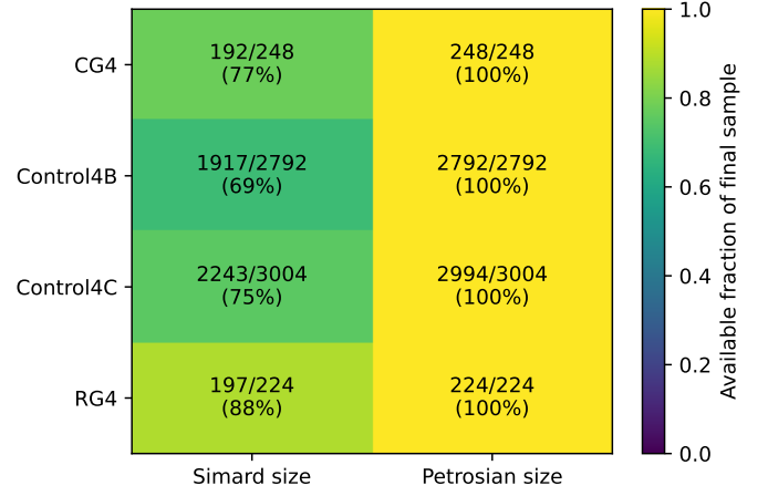
Fig. C.18. Availability of the seeing-corrected Simard half-light radius and the Petrosian half-light radius in each sample, after the bridge, quality, and blending cuts of Sect. 2.4.
