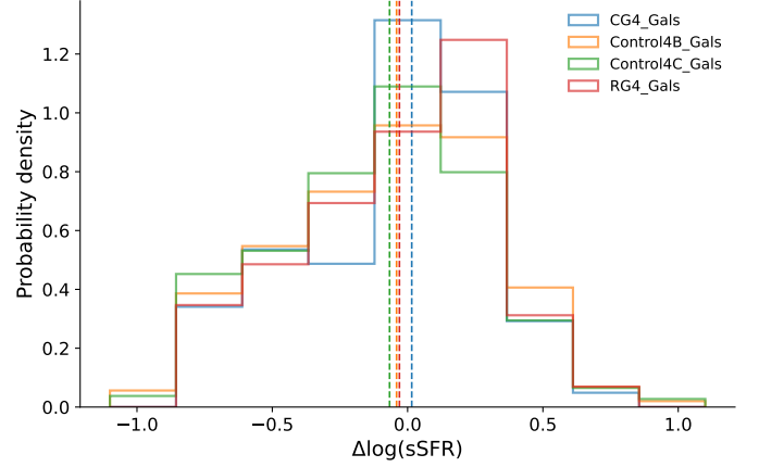
Fig. 4. Main-sequence residual distributions for the star-forming galaxies in each sample.
