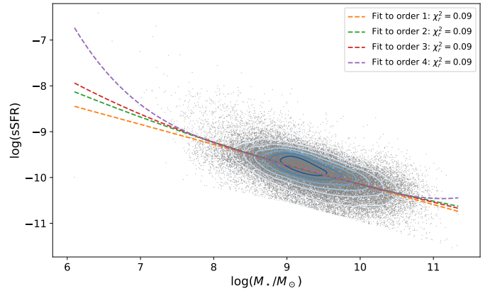
Fig. A.5. Polynomial fits of orders 1–4 to the star-forming main sequence.
