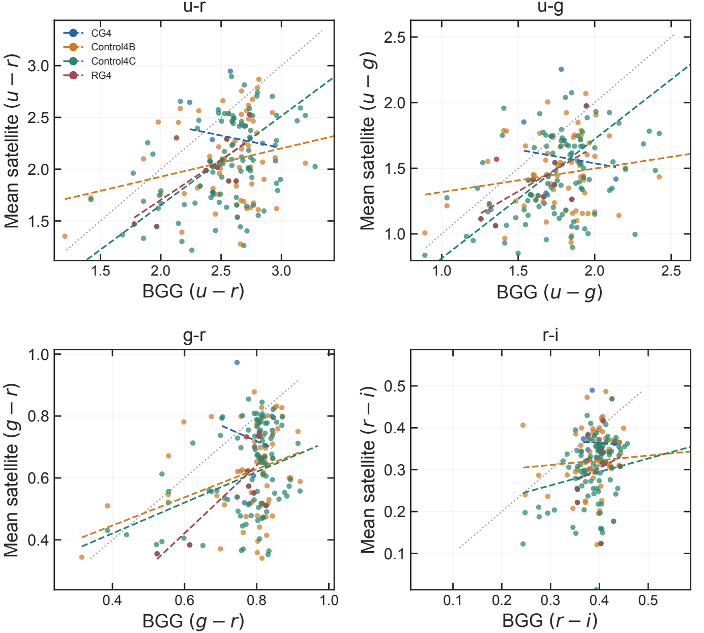
Fig. 21. Mean satellite colour versus BGG colour for groups with matched photometry. The dotted line is the one-to-one relation and dashed lines are catalogue-specific fits.
