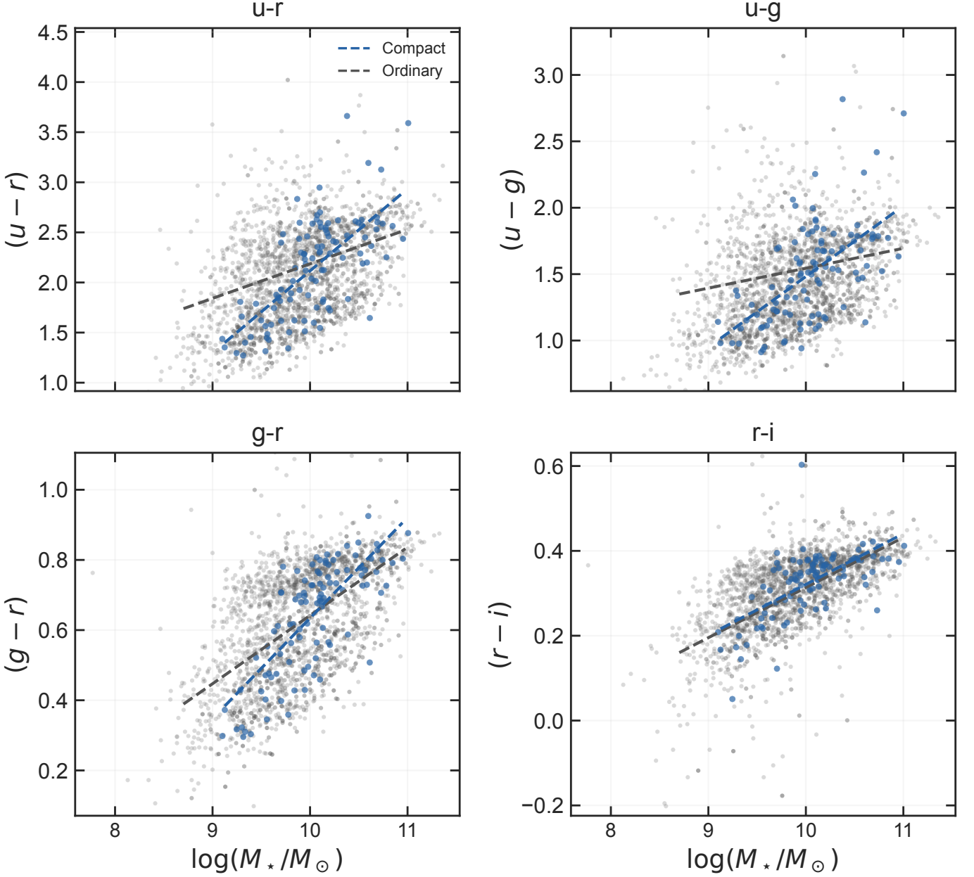
Fig. 18. Satellite colour–mass relations in compact and ordinary groups. The fitted lines show both colour offsets at the reference mass and differences in slope.
