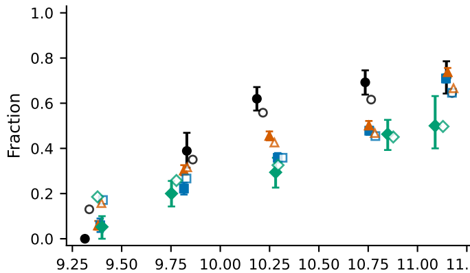
(c) Quenched fraction: satellites
