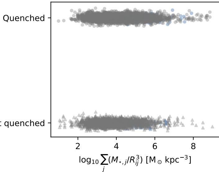
Quenched status
