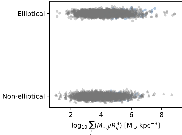
Elliptical morphology
