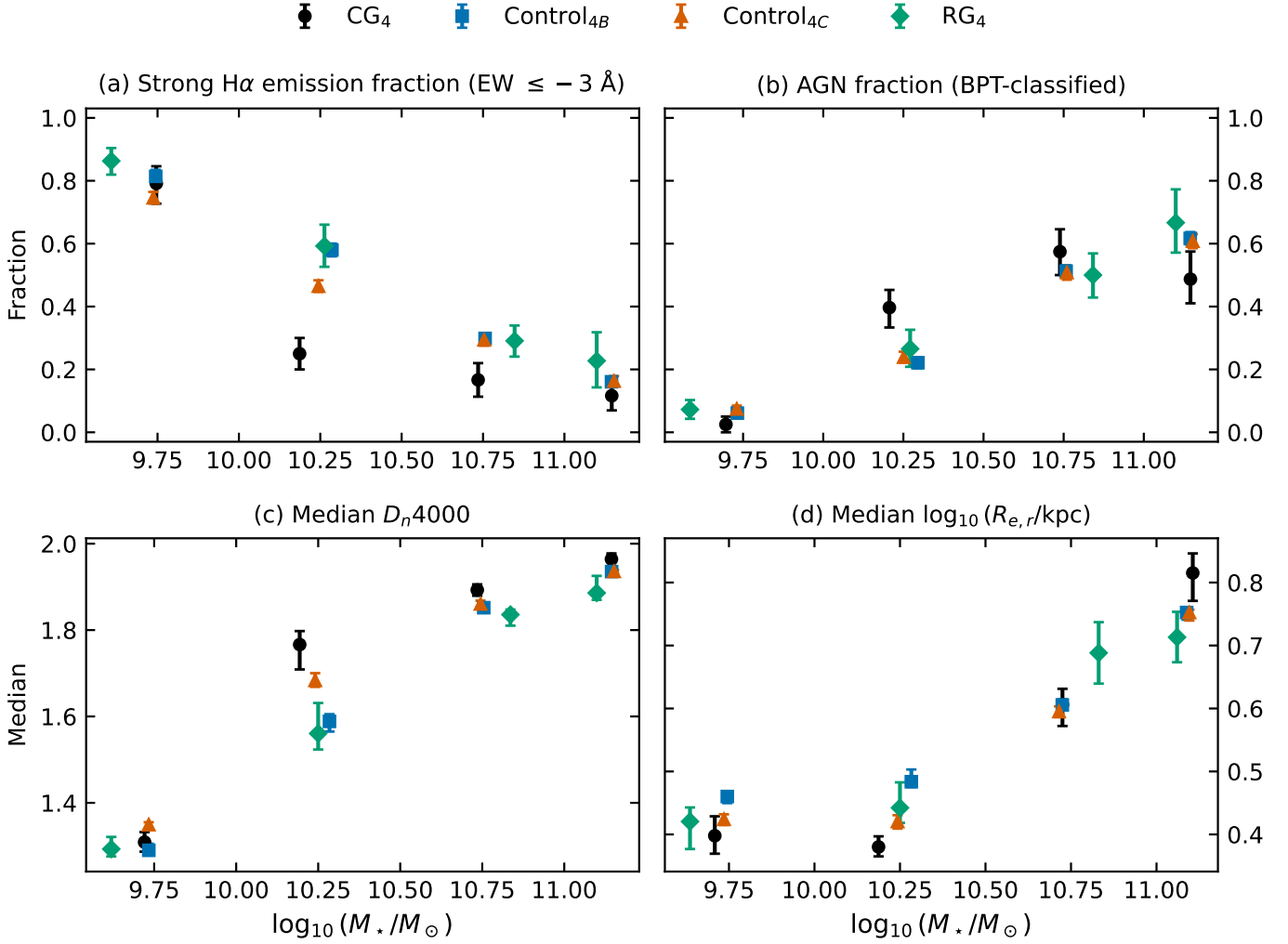
Fig. 4. Other galaxy properties versus stellar mass: (a) strong- H\alpha fraction; (b) AGN fraction among BPT-classified galaxies; (c) median D_n4000 ; (d) median seeing-corrected effective radius \log_{10}(R_{e,r}/\text{kpc}) . Bins and group-blocked intervals follow Fig. 2; these comparisons are descriptive.
