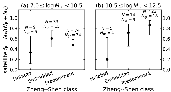
Fig. 3. Mass-controlled satellite E-class fractions. Panels use the common mass bins shown above each axis; points and bars give class fractions and Wilson 95% intervals, with classified-galaxy and contributing-group counts.
