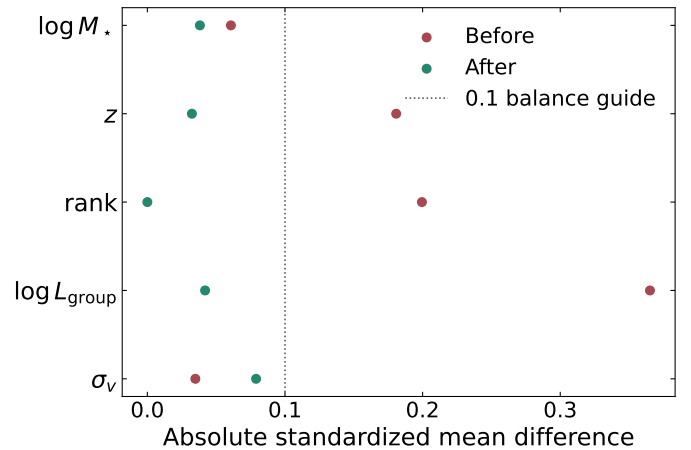
Fig. G.1. Matching balance. Absolute standardized mean differences before and after matching; the labelled 0.1 line is a conventional diagnostic guide.
