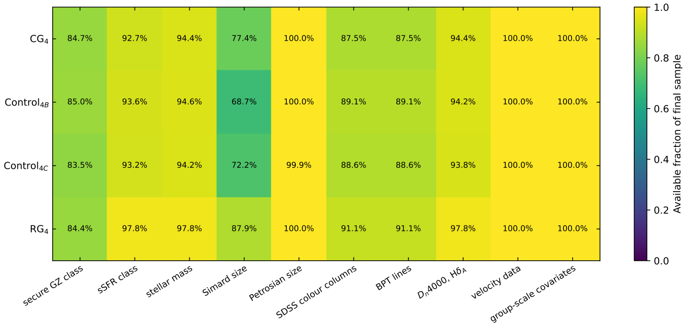
Fig. G.2. Measurement availability. Cells give percentages of the final per-sample galaxy count. The colour row describes the four derived SDSS columns, the spectral-index row requires finite non-sentinel values with positive errors, and the Simard row includes all size-quality cuts.
