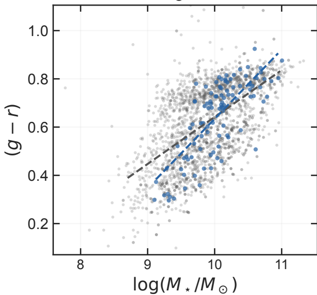
g-r
