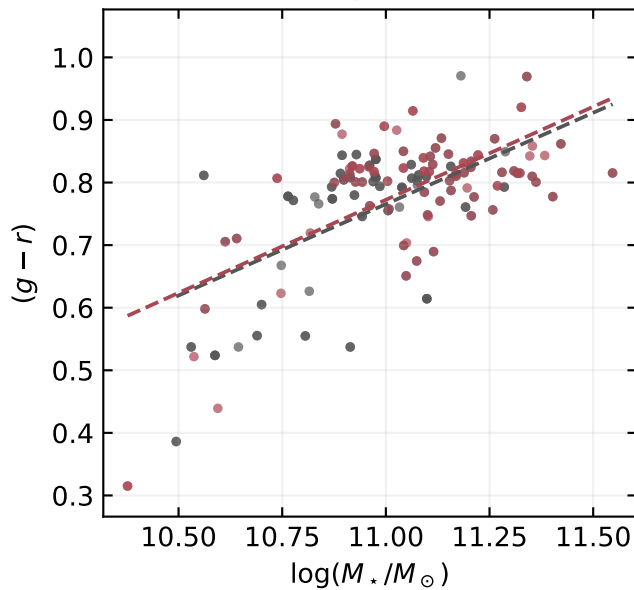
g-r
