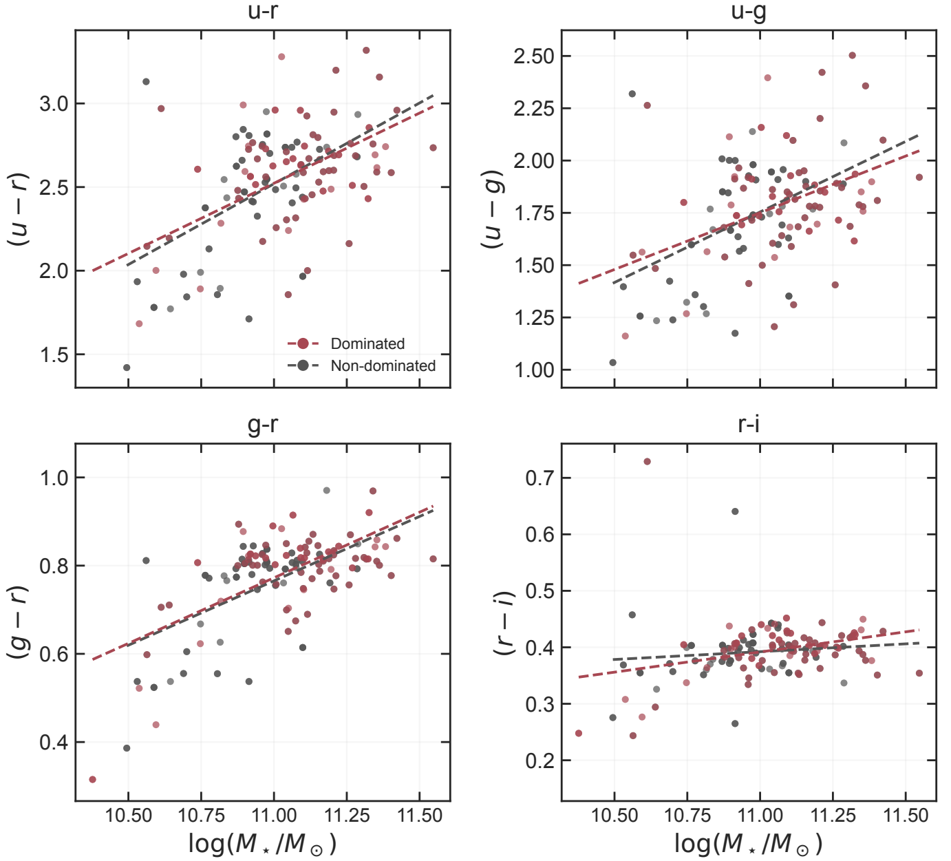
Fig. 21: BGG colour–mass relations split by luminosity domination. Comparing the fitted relations at a common stellar mass separates colour effects from the different mass distributions.
