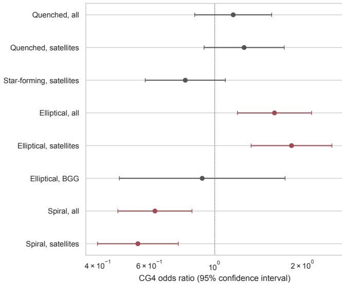
Fig. 5. Adjusted \text{CG}_4 odds ratios for star-formation and morphology diagnostics, including all-galaxy, satellite-only, and BGG-only morphology rows. Bars show 95% confidence intervals; the vertical line marks equal odds.
