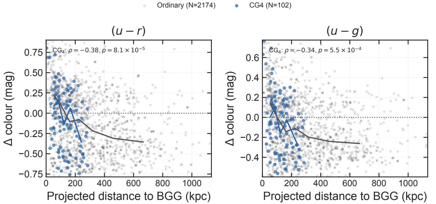
Fig. C.12. Mass- and redshift-adjusted satellite (u-r) and (u-g) residuals as a function of projected distance to the BGG. Lines connect binned medians for \text{CG}_4 and the pooled ordinary-group satellites; extreme plotting tails are omitted for readability, while the reported rank correlations use the full matched sample. More negative residuals are bluer than the ordinary-satellite reference relation.
