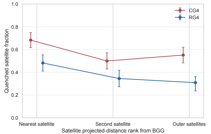
Fig. 9. Quenched satellite fraction as a function of projected-distance rank from the BGG. Points show \text{CG}_4 and \text{RG}_4 fractions; bars show group-cluster bootstrap 16th–84th percentile intervals.
