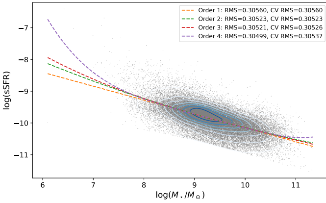
Fig. C.4. Polynomial fits of orders 1–4 to the star-forming main sequence. The legend reports residual RMS and five-fold cross-validated RMS scatter in dex; order 2 is adopted because it is the lowest-order model with the smallest cross-validated RMS scatter.
