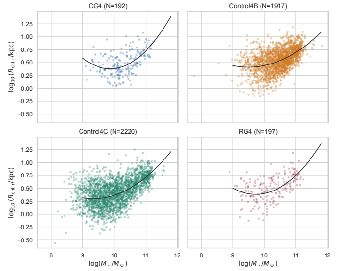
Fig. C.19. Seeing-corrected half-light radius versus stellar mass in each sample. Solid curves show the descriptive quadratic fits used to quize a predicted size at the reference stellar mass.
