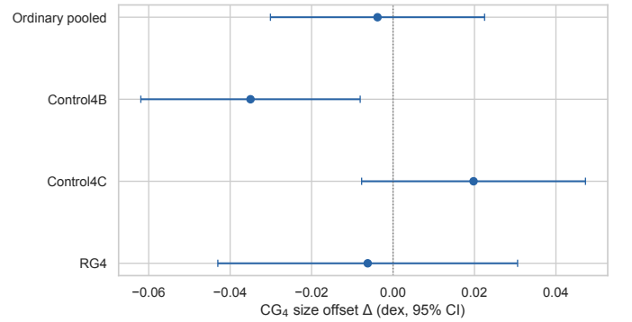
Fig. C.20. Mass- and redshift-adjusted CG4 size coefficients against the pooled controls and against each control catalogue separately. Bars show 95% confidence intervals; negative values mean smaller CG4 sizes at fixed mass.
