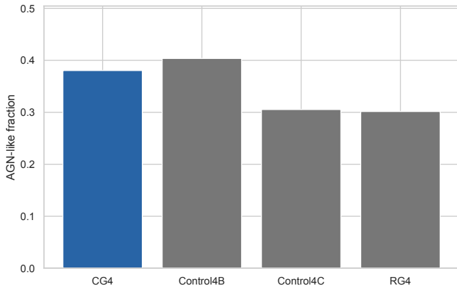
Fig. 33. AGN-like fractions from the BPT/AGN-flag classification.
