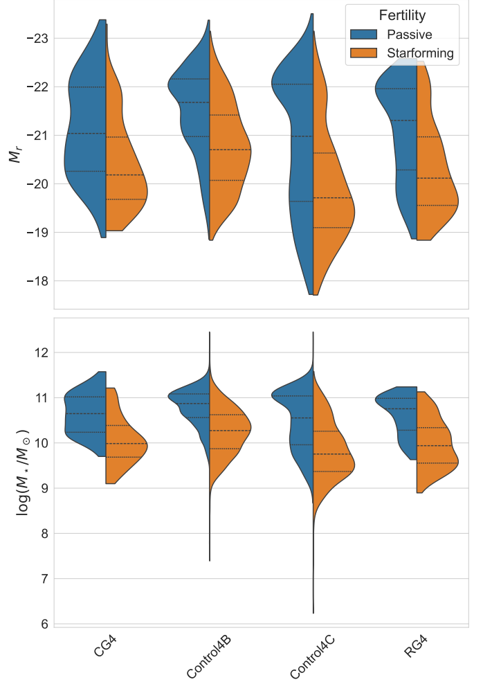
Fig. 6. Distributions of various quantities for galaxies according to their fertility.
