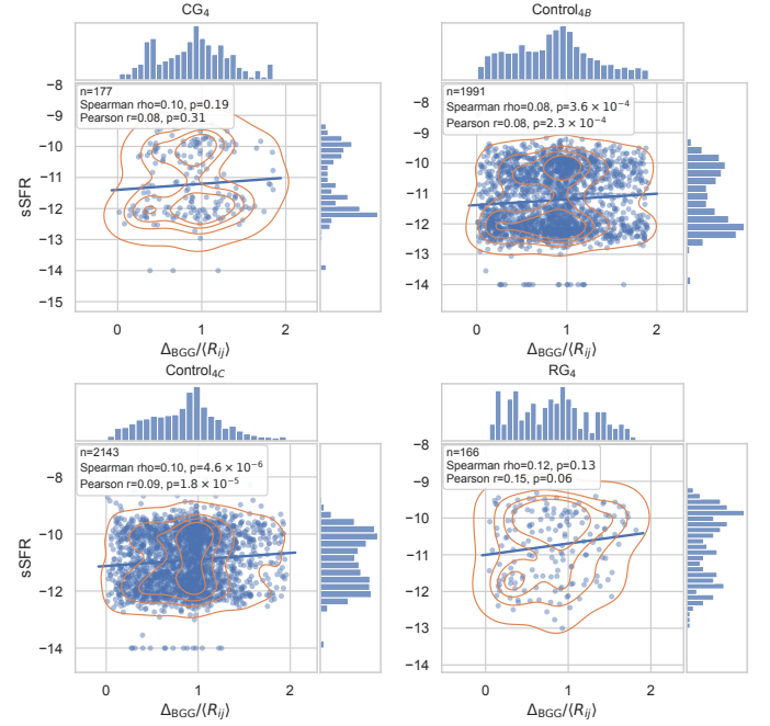
Fig. 12. sSFR as a function of projected distance to the BGG normalized by \langle R_{ij} \rangle for satellite galaxies in each sample.
