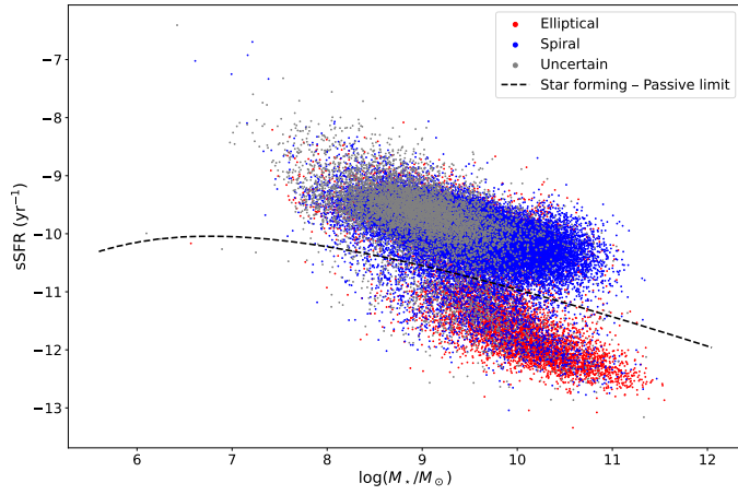
Fig. 3. sSFR vs mass, star-forming/passive limit and Zoo morphologies for the SDSS control sample, excluding quenched galaxies.
