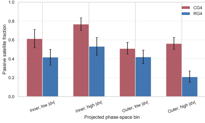
Fig. 29. Passive satellite fraction in coarse projected phase-space bins. Inner and outer refer to projected-distance rank from the BGG; low and high velocity are split at |\Delta v_{\text{BGG}}|/\sigma_v = 1 .
