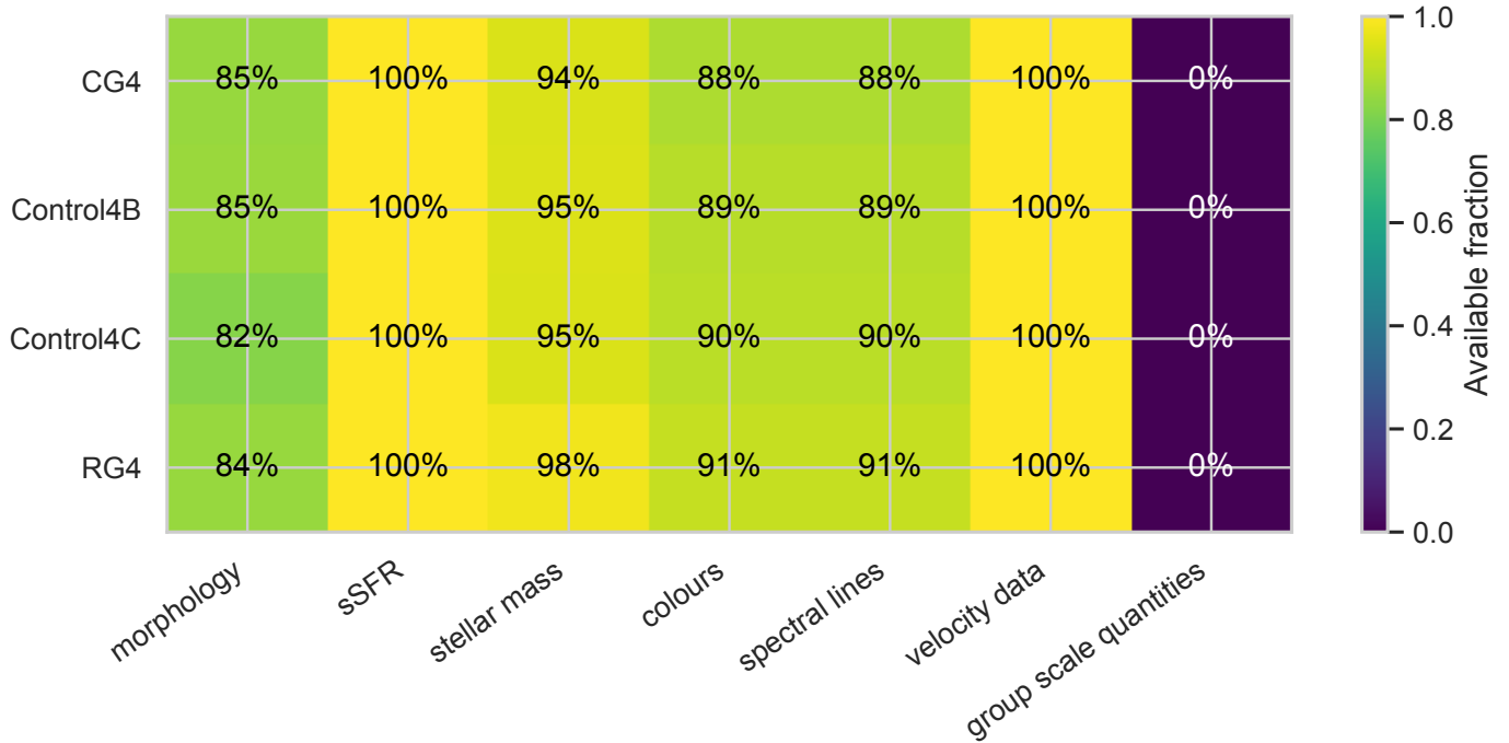
Fig. 35. Availability fractions for the major derived quantities in each sample.
