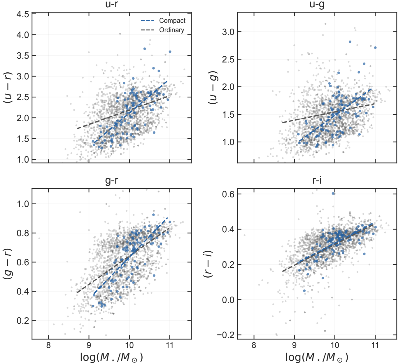
Fig. 19. Satellite colour–mass relations in compact and ordinary groups. The fitted lines show both colour offsets at the reference mass and differences in slope.
