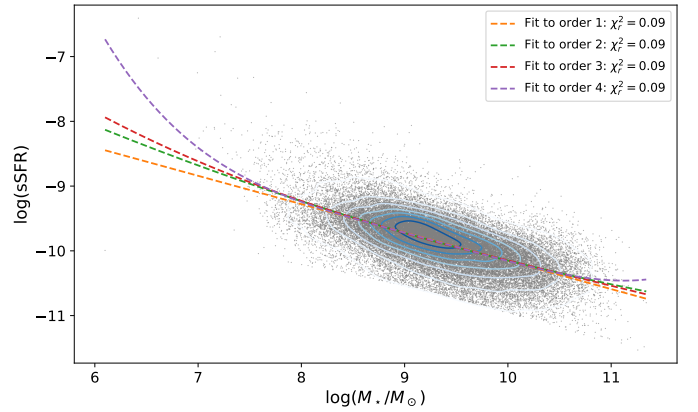
Fig. 9. Polynomial fits of orders 1–4 to the star-forming main sequence.
