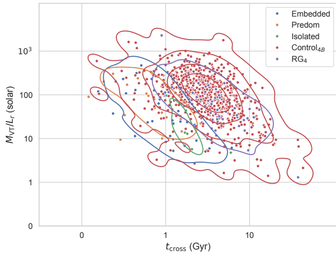
Fig. 15. Crossing time versus virial mass-to-light ratio for the compact groups and their controls.
