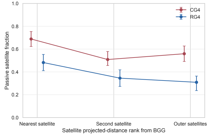
Fig. 27. Passive satellite fraction as a function of projected-distance rank from the BGG. Points show CG 4 and RG 4 fractions; bars show group-cluster bootstrap 16th-84th percentile intervals.
