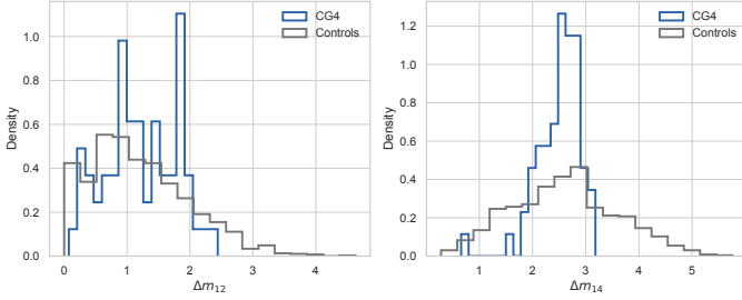
Fig. 30. Distributions of the first-second and first-fourth magnitude gaps in CG 4 and the pooled controls.
