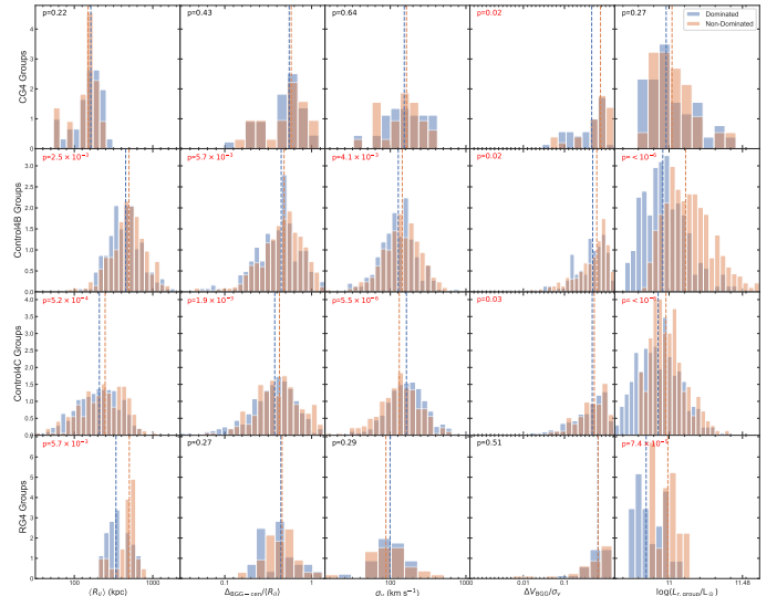
Fig. 13. Distributions of the main group-scale observables in dominated and non-dominated systems.
