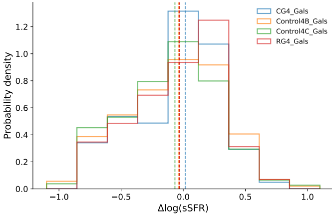
Fig. 10. Main-sequence residual distributions for the star-forming galaxies in each sample.
