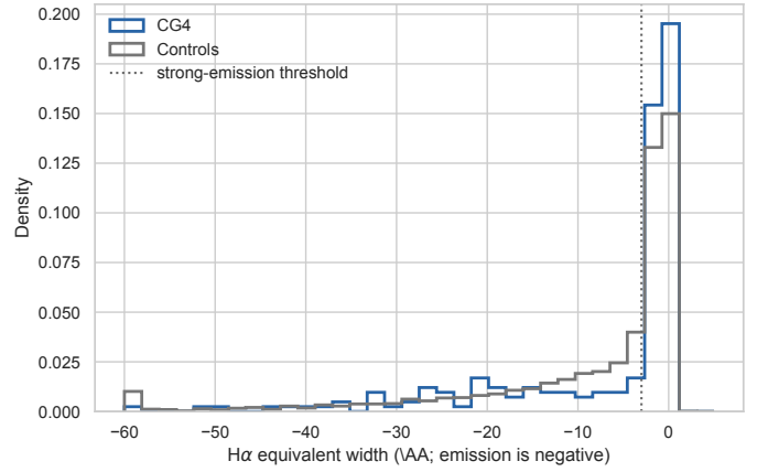
Fig. 32. H\alpha equivalent-width distributions used for the limited recent-quenching diagnostic.
