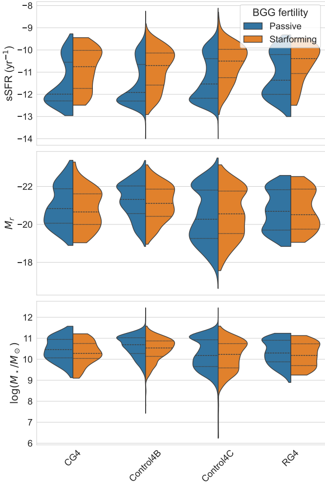
Fig. 7. Distributions of various quantities for galaxies according to the fertility of their BGG (BGG included).
