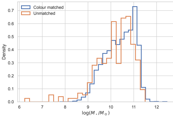
Fig. 36. Stellar-mass distributions of galaxies with and without complete matched colour measurements.
