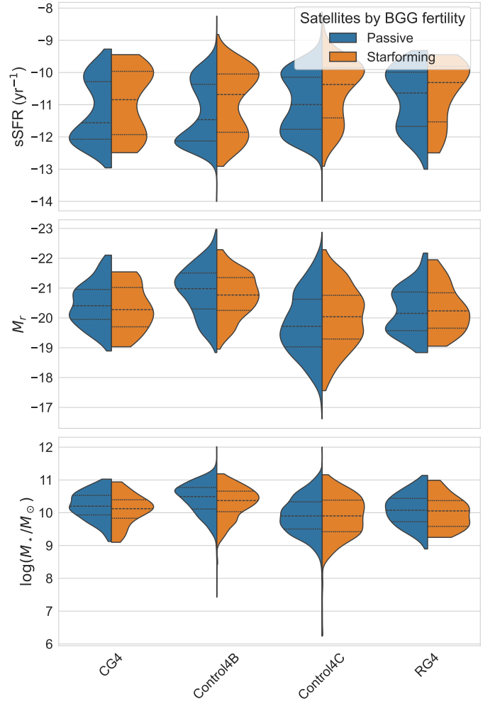
Fig. 8. Distributions of various quantities for galaxies according to the fertility of their BGG (satellites only).
