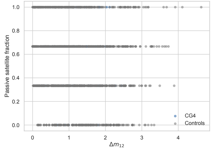
Fig. 31. Passive satellite fraction as a function of the first-second magnitude gap.
