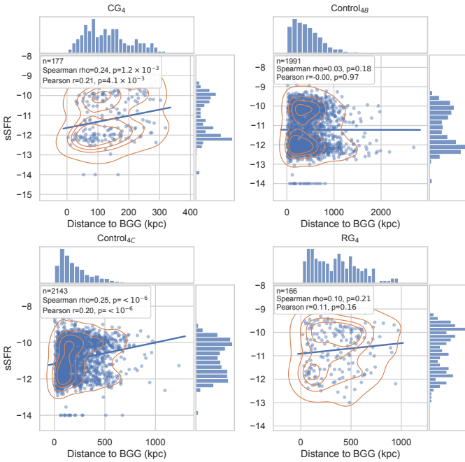
Fig. 11. sSFR as a function of projected distance to the BGG, in kpc, for satellite galaxies in each sample.
