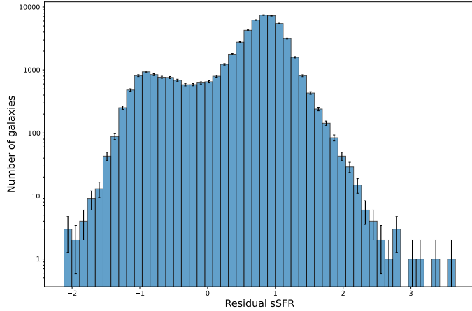
Fig. 4. Distribution of residual sSFR offsets from the adopted star-forming main sequence.
