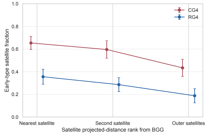
Fig. 28. Early-type satellite fraction as a function of projected-distance rank from the BGG. Because the catalogue separates ellipticals, spirals, and uncertain morphologies but not S0 galaxies, early type is equivalent to elliptical in this diagnostic.
