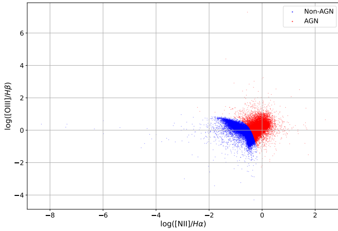
Fig. 1. BPT diagram showing our separation between non-AGN and AGN galaxies.
