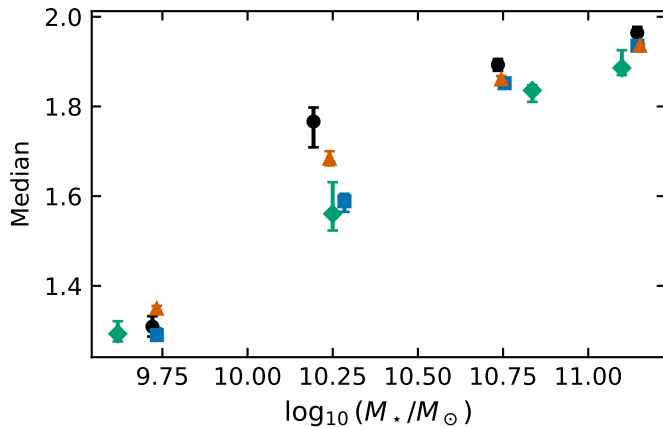
(c) Median D_n4000
