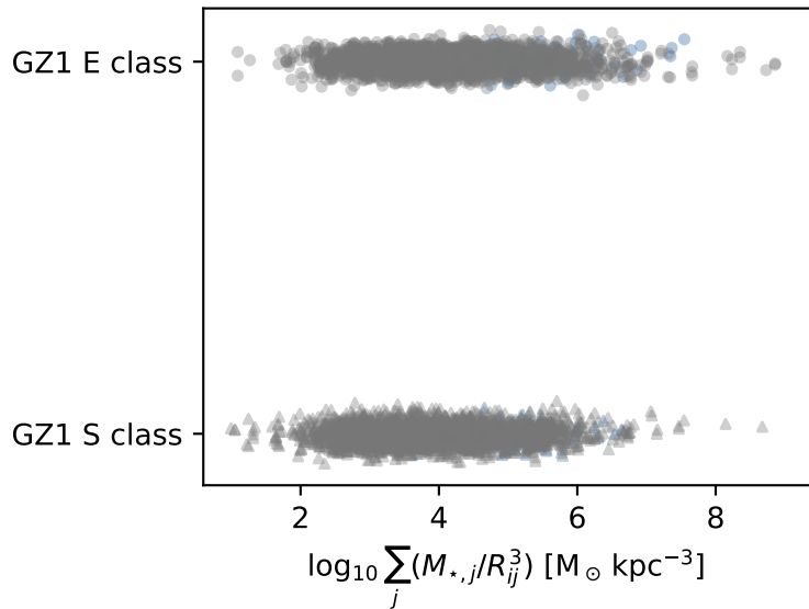
GZ1 E-class morphology
