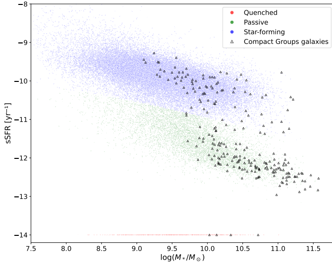
Fig. 2. sSFR and morphologies of galaxies in CG 4 and our SDSS selection. Quenched galaxies are represented at an arbitrary low value of 10^{-14.0} \text{ yr}^{-1} .
