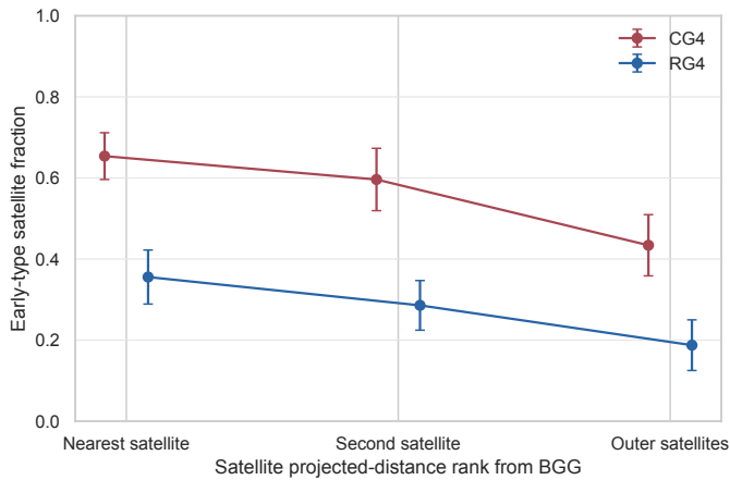
Fig. 10. Early-type satellite fraction as a function of projected-distance rank from the BGG. Because the catalogue separates ellipticals, spirals, and uncertain morphologies but not S0 galaxies, early type is equivalent to elliptical in this diagnostic.
