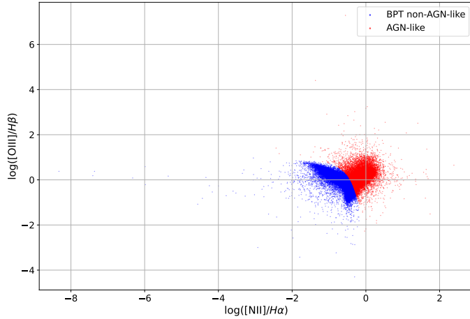
990 Fig. B.1. BPT diagram for galaxies with measured diagnostic line ratios. The AGN-like region is excluded from the sSFR calibration sample; galaxies without the required ratios are BPT-unclassified rather than classified as non-AGN by this diagram.
