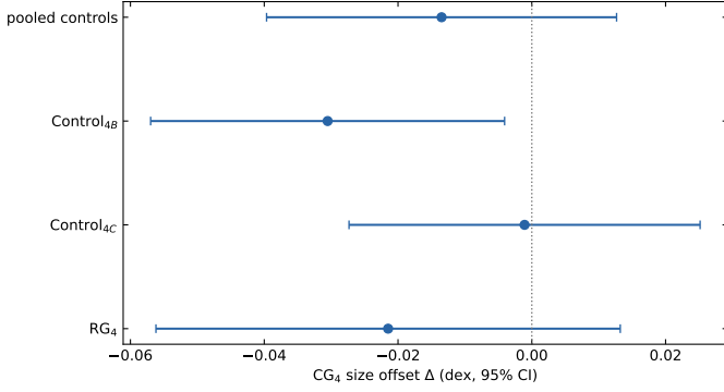
Fig. S.10. Group-adjusted CG 4 size coefficients against the deduplicated pooled controls and each control catalogue separately. Every model uses the article's main adjustment set: stellar mass, redshift, a BGG/satellite indicator, quartet luminosity, and velocity dispersion, with physical-group-clustered uncertainties. Bars are 95% confidence intervals; negative values denote smaller CG 4 effective radii at fixed co-variates.
