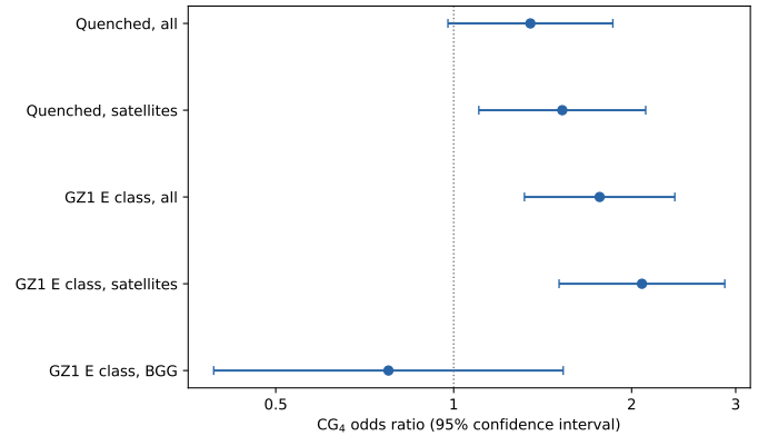
Fig. S.7. Adjusted CG 4 odds ratios from the pooled models. The GZ1 E-class outcomes refer to the smooth early-type-like GZ1 class, not to a physically pure sample of classical ellipticals. Points are odds ratios and bars are 95% confidence intervals; the vertical line marks no difference.
