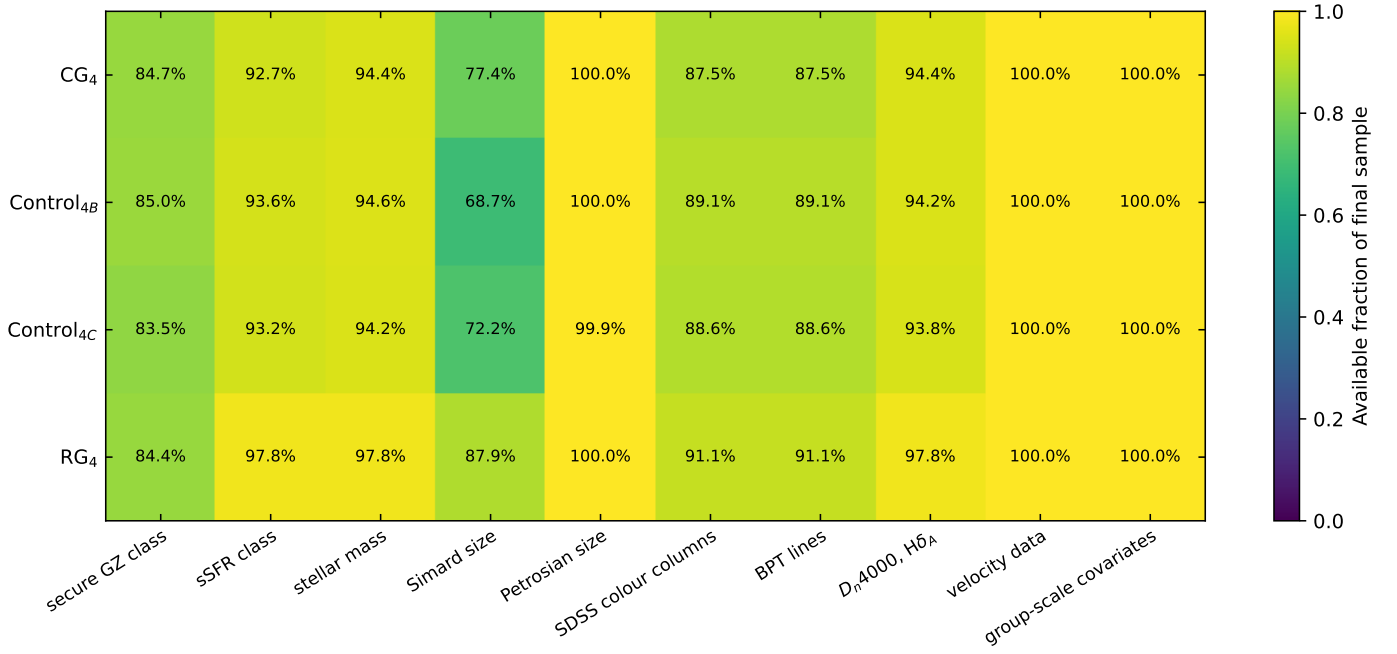
Fig. S.9. Measurement availability in the four samples. Cells give percentages of the final per-sample galaxy count. The colour row describes the four derived SDSS columns, the spectral-index row requires finite non-sentinel values with positive errors, and the Simard row includes all size-quality cuts.
