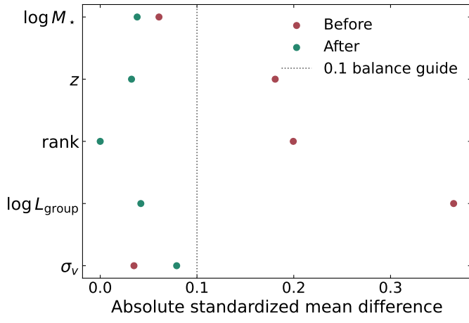
Fig. S.8. Balance of the galaxy-level match of the article’s appendix on matching. Absolute standardised mean differences before and after matching; the labelled 0.1 line is a conventional diagnostic guide.
