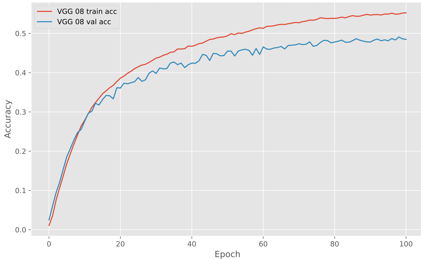
Training and Validation Accuracy per Epoch
