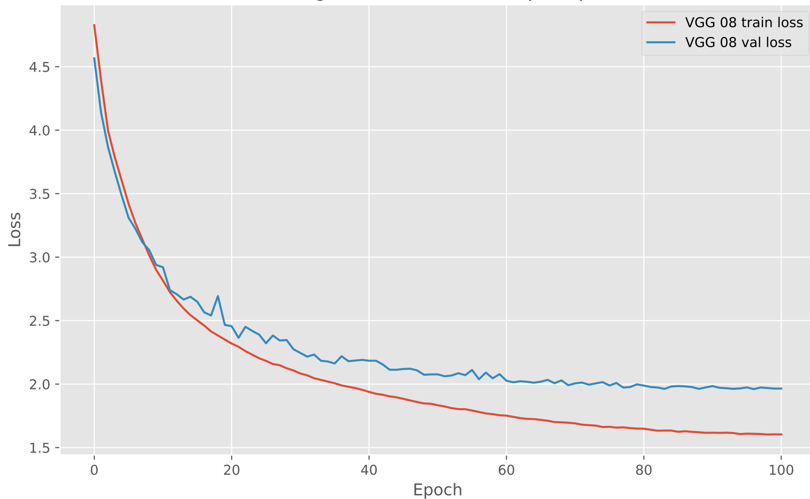
Training and Validation Loss per Epoch
