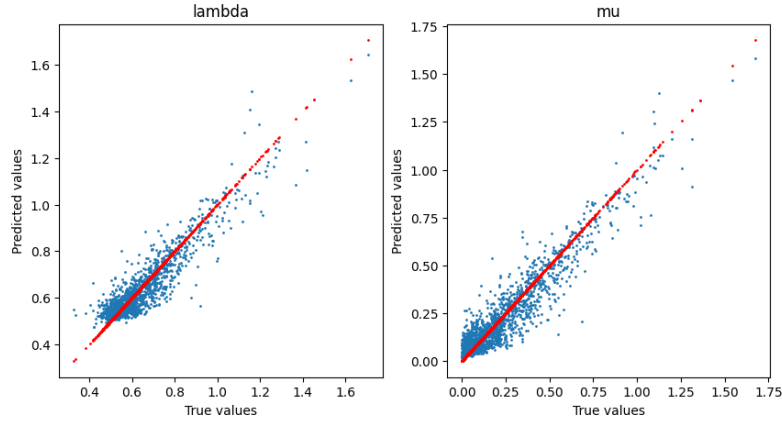
Figure 4.2. Results obtained with the Random Forest Classifier for the BD model. The red scatter points represent the true values, while the blue points represent the predicted values. The points are really close to the line y = x , which means that the predictions are accurate.
