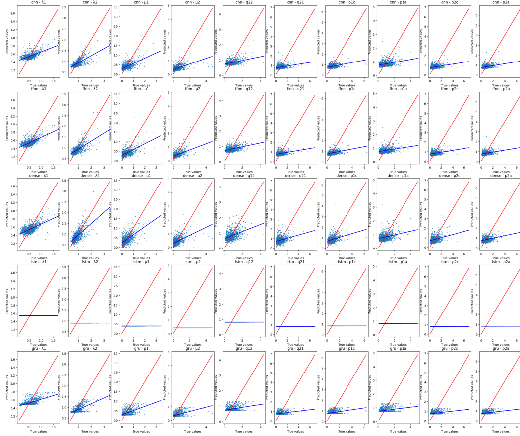
Figure 4.5. BiSSEness model, one of the most complex to infer. The state-related parameters (from the 5th column on) are difficult to be predicted due to the already discussed reasons. Notably, RNN models (GRU and LSTM, the last two rows) have the worst performance, because Summary Statistics encoding is not sequential.
