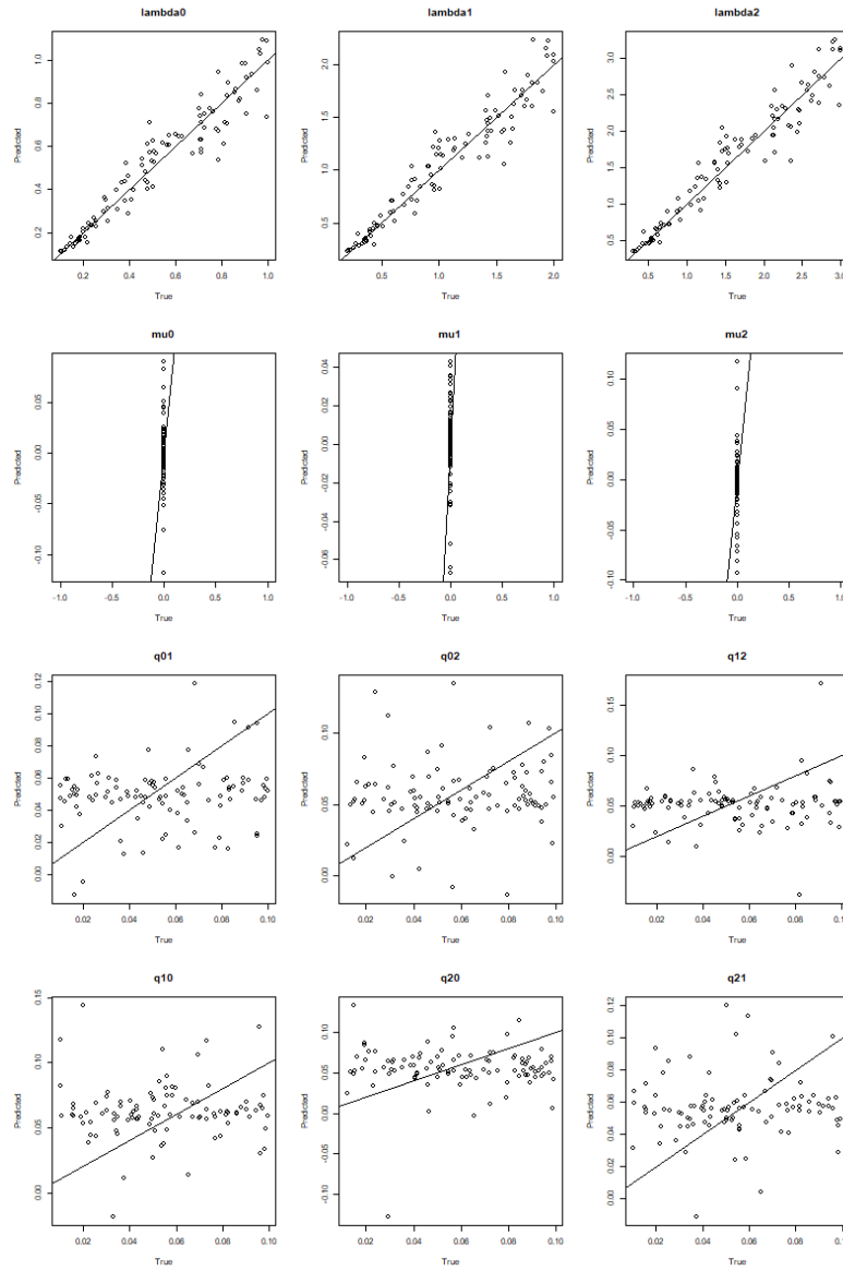
Figure 5.2. MuSSE with 3 states: True vs predicted parameters with DNN architecture and SS encoding. Only 1000 trees were used to train the models. The black line represents the true values.
