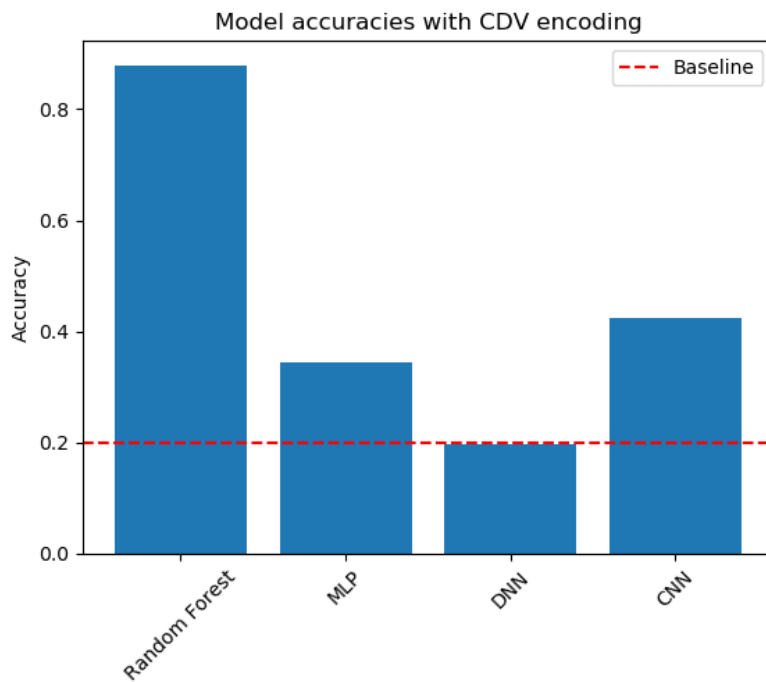
Figure 6.3. Results obtained with the different models trained on CDV encoding.
