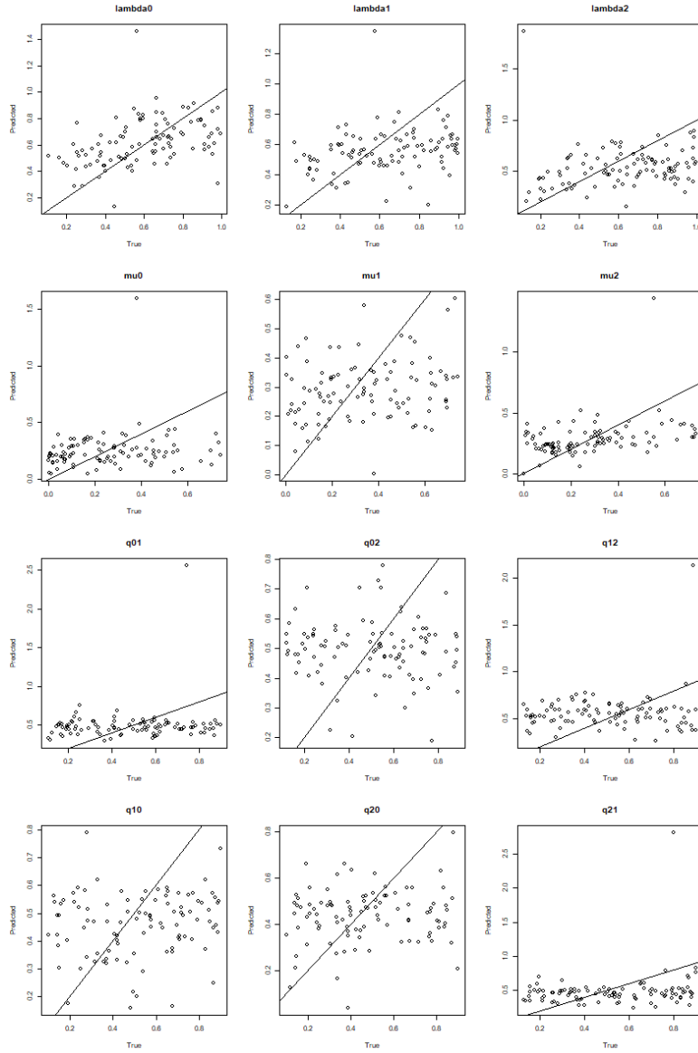
Figure 5.3. MuSSE with 3 states: true vs predicted parameters with DNN architecture and SS encoding, without the constraints imposed by the authors. The black line represents the true values. Even if the model was trained with a manipulated training set, that includes the true values of the parameters, the predictions are completely off the true values, and the model is randomly predicting the parameters: this shows that the strong constraints imposed by the authors play a crucial role in the accuracy of the predictions.
