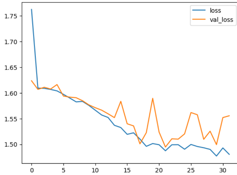
Figure 6.2. History of the training of the Convolutional Neural Network for the model predictor for the CDV encoding.
