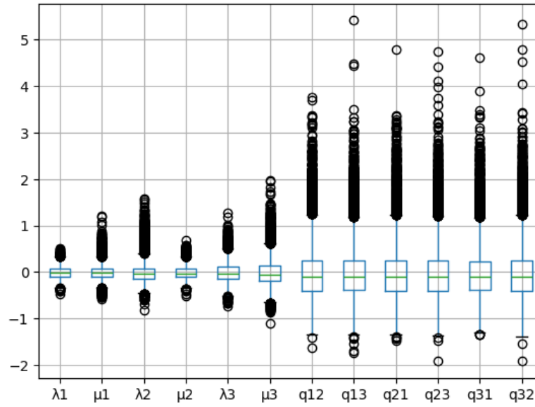
Figure 4.6. Boxplot of the error of the predictions obtained with the Random Forest Classifier for the MuSSE model. As said before, the classifier lacks in predicting the transition rates, due to tree structures not containing information about the character states and the limitation of available data, while the speciation and extinction rates are predicted with a good accuracy.
