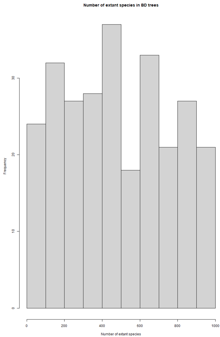
Figure 3.3. Number of species in each tree, generated with the function tree.bd . The number of species is uniformly distributed between 10 and 1000.
