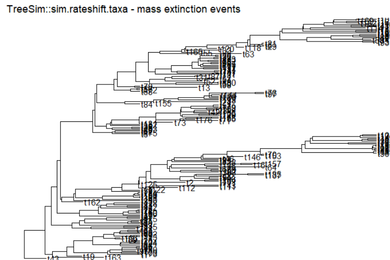
Figure 3.5. This tree was generated with sim.rateshift.taxa , from the package TreeSim . We can see how irregular the pattern is, compared to the constant birth-death models seen before, due to the presence of mass extinction events and rate shifts.
