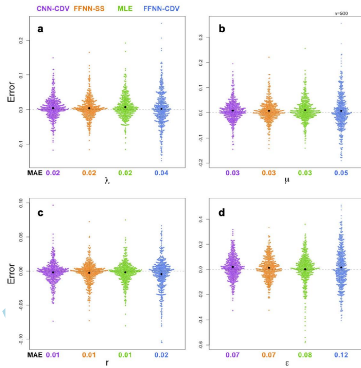
Figure 4.1. Results obtained on BD with the deep learning models trained on the CDV encoding and the SS encoding, and with the MLE method. The plots show the Mean Absolute Error (MAE) for the speciation rate, the extinction rate, net diversification and turnover rate.
