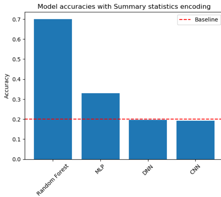
Figure 6.4. Results obtained with the different models trained on SS encoding.
