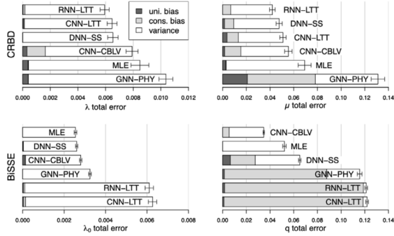
Figure 5.1. Paper results obtained with the different models and phylogeny representations.
