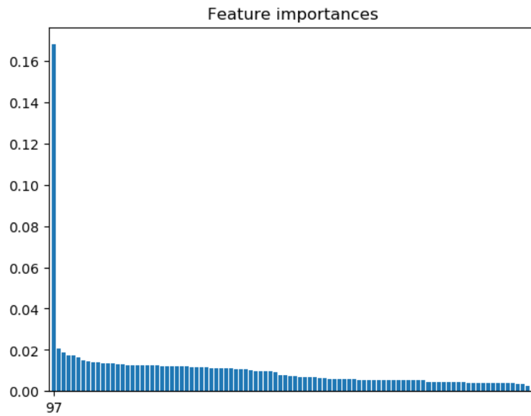
Figure 6.1. Feature importance scores for the Random Forest Classifier trained on the SS encoding. The most important feature is feature 97, which is the last feature in the dataset, and represents the scaling factor.
