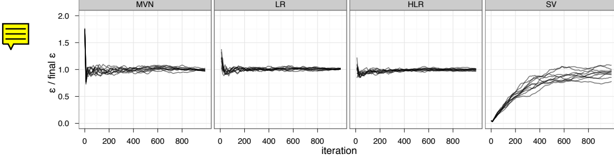
Figure 4: Plots of the convergence of \bar{\epsilon} as a function of the number of iterations of NUTS with dual averaging with \delta = 0.65 applied to the multivariate normal (MVN), logistic regression (LR), hierarchical logistic regression (HLR), and stochastic volatility (SV) models. Each trace is from an independent run. The y-axis shows the value of \bar{\epsilon} , divided by one of the final values of \bar{\epsilon} so that the scale of the traces for each problem can be readily compared.
