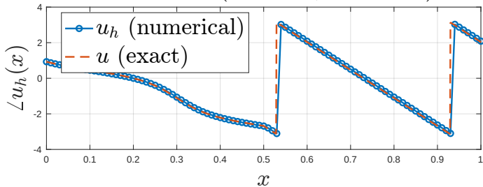
Phase of u_h ( h = 0.01 , n_{\text{El}} = 100 )
