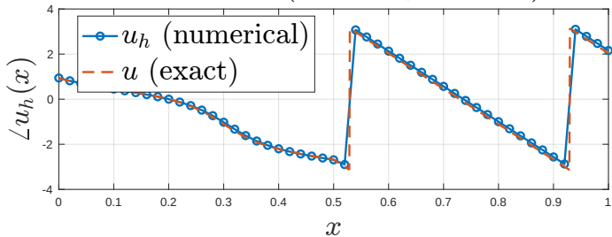
Phase of u_h ( h = 0.02 , n_{\text{El}} = 50 )
