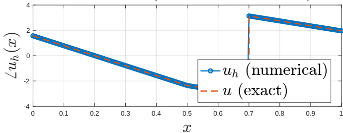
Phase of u_h ( h = 0.005 , n_{\text{El}} = 200 )
