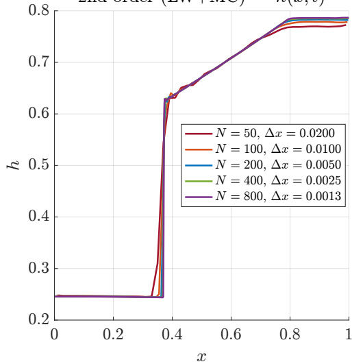
2nd order (LW+MC) — h(x, t)
