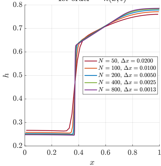
1st order — h(x, t)
