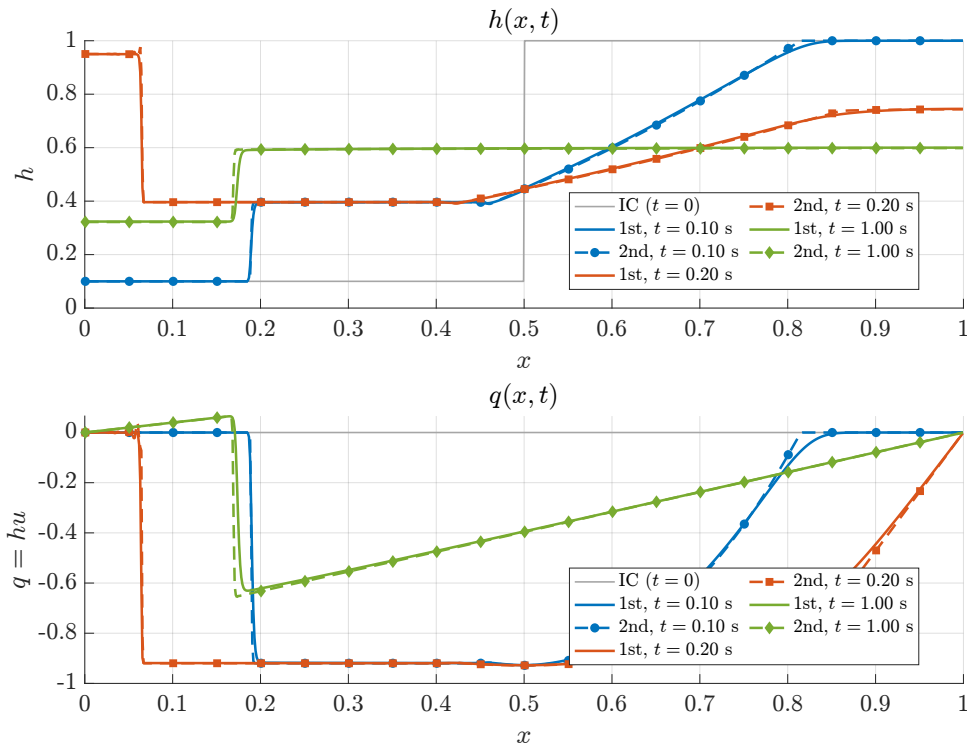
Case (b): Reverse Dam Break — \Delta x = 0.0013 , CFL = 0.15, \Delta t_{\text{avg}} \approx 0.0490 ms
